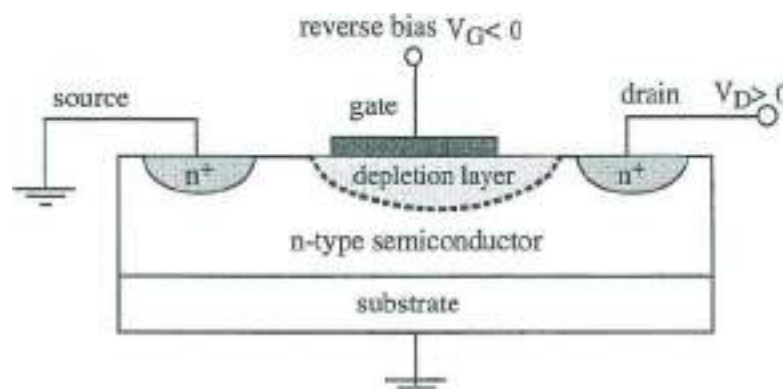
Fig. 15 Schematic illustration of the metal-semiconductor field effect transistor. The principle of operation is quite similar to the junction field effect transistor; the blocking p^+n junctions of the JFET are here replaced by the blocking metal-semiconductor contact.
