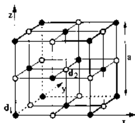
Fig. 6 Crystal structure of sodium chloride: the end-points of the basis vectors d_1 and d_2 given in Eqs. (9) of the text, are also indicated.
