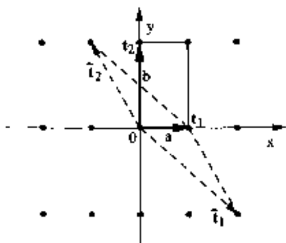
Fig. 1 Illustration of a two-dimensional rectangular Bravais lattice. The lattice can be described by the primitive translation vectors t_1 = a(1, 0, 0) and t_2 = b(0, 1, 0) . Although this is the most natural choice, infinite other choices are possible; the figure illustrates the choice \bar{t}_1 = (2a, -b, 0) and \bar{t}_2 = (-a, b, 0) . Whatever choice is done, the area of the unit cell is invariant and equals ab .
