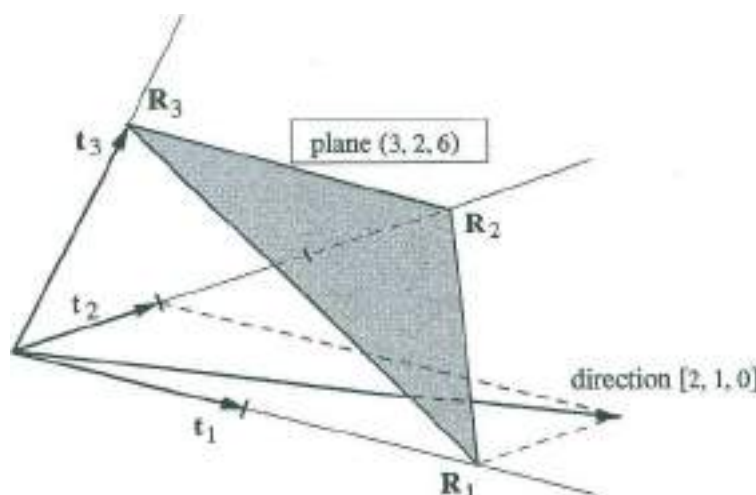
Fig. 16 Miller indices of planes and directions in a Bravais lattice.
