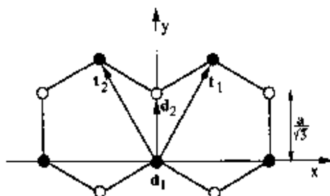
Fig. 10 Layer structure of two-dimensional graphite. The primitive translation vectors t_1 and t_2 , and the basis vectors d_1 and d_2 , given by Eqs. (13) of the text, are also indicated.
