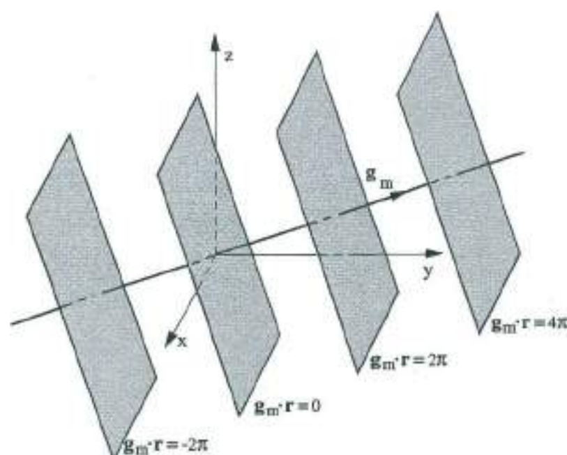
Fig. 15 Family of planes in direct space defined by the equations \mathbf{g}_m \cdot \mathbf{r} = 0, \pm 2\pi, \pm 4\pi, \dots ; all the translation vectors of the Bravais lattice belong to the family of planes.
