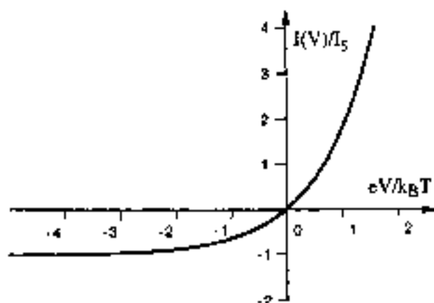
Fig. 5 Ideal I - V characteristic for a pn-junction with I(V) = I_s [\exp eV/k_B T - 1] .
