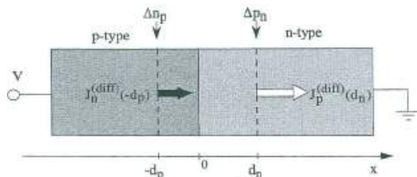
Fig. 4 Schematic representation of a pn homojunction with an applied potential V on the p side (the n-side is grounded); \Delta n_p and \Delta p_n denote the change in the concentration of minority carriers at the boundaries between the space charge region and the neutral regions. The figure refers to the case V > 0 , so that \Delta n_p and \Delta p_n are positive. J_n^{(diff)}(-d_p) denotes the electron diffusion current at x = -d_p , and J_p^{(diff)}(d_n) the hole diffusion current at x = d_n . (Notice that the electron current is in the opposite direction to the electron flow, while the hole current and the hole flow are in the same direction). The diode current is approximately the sum J_n^{(diff)}(-d_p) + J_p^{(diff)}(d_n) .
