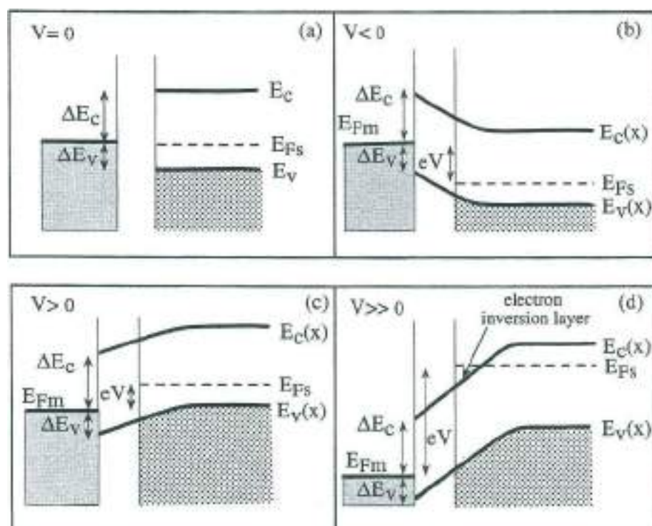
Fig. 17 Band structure of an 'ideal' metal oxide-semiconductor system and energy band profiles for V = 0 (flat-band situation), V < 0 (hole accumulation), V > 0 (hole depletion), V \gg 0 (inverse layer formation). The energy differences between the Fermi level of the metal and the band edges of the semiconductor are indicated by \Delta E_v and \Delta E_c ; these discontinuities are independent of the applied electric field.
