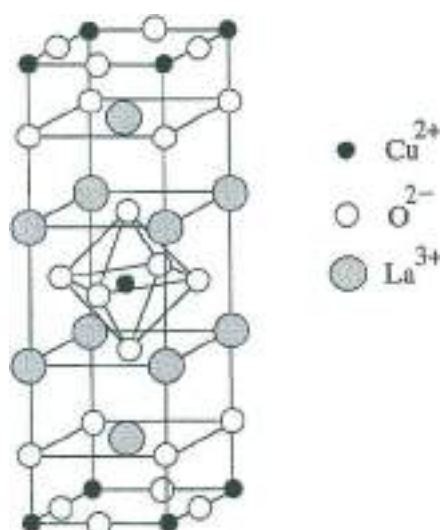
Fig. 1 Crystal structure of \text{La}_2\text{CuO}_4 .
