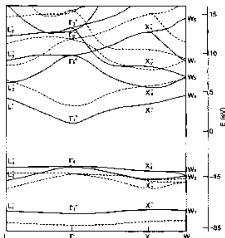
Fig. 1 Energy bands of solid argon with inclusion of correlation effects (solid line). For comparison the energy bands in the Hartree-Fock approximation are also reported (dashed lines), correlation effects shift (almost rigidly) the Hartree-Fock conduction bands to lower energies, and the Hartree-Fock valence bands to higher energies [from S. Baroni, G. Grosso and G. Pastori Parravicini, Phys. Rev. D29 , 2891 (1984), copyright 1984 by the American Physical Society].
