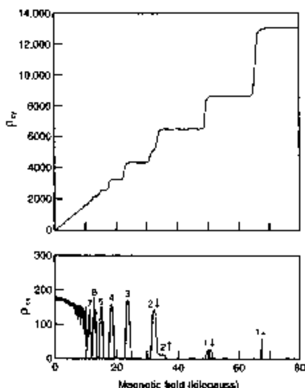
Fig. 13 Hall resistance \rho_{xy}(H) and parallel component of the resistance \rho_{xx}(H) (in ohm) of a two-dimensional electron gas at the \text{GaAs-Al}_x\text{Ga}_{3-x}\text{As} interface. The quantum Hall effect is already evident at about 10 kgauss. The numbers and the arrows above \rho_{xx}(H) maxima refer to the Landau quantum number and the spin polarization of the levels [from M. A. Paalanen, D. C. Tsui and A. C. Gossard, Phys. Rev. B 25 , 5566 (1982); copyright 1982 by the American Physical Society].
