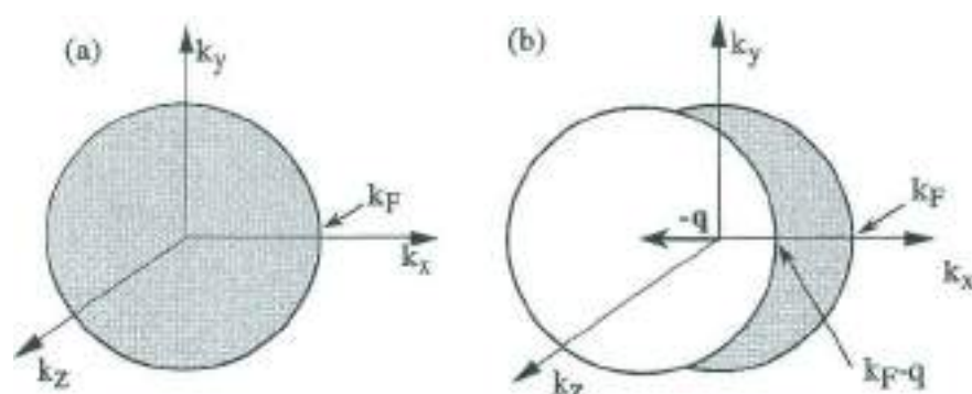
Fig. 16 Schematic representation in the k -space of the Fermi sphere of radius k_F , representing the ground-state of the free-electron gas. In (a) we have shadowed the region where the Fermi-Dirac distribution function f(k) = 1 , at zero temperature. In (b) we have shadowed the region where f(k)[1 - f(k+q)] = 1 .
