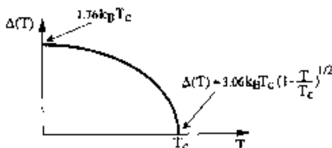
Fig. 14 Behaviour of the energy gap parameter \Delta(T) for a superconductor in the BCS theory and weak coupling limit.
