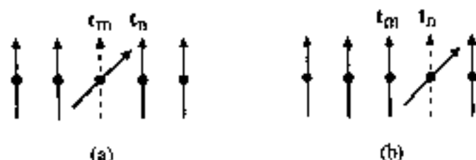
Fig. 5 Schematic representation of trial excited states of the spin Hamiltonian. In (a) there is a spin deviation at the site t_m , and in (b) there is a spin deviation at the adjacent site t_n . In the spin-wave theory, the operators which couple spin deviations on different sites produce a wave-like Bloch state.
