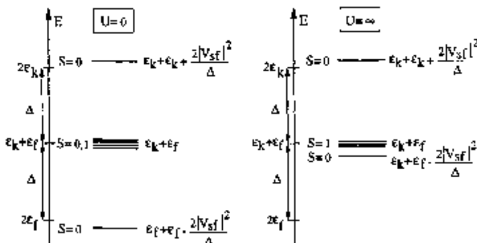
Fig. 7 Energy levels of the two-electron two-orbital molecule, with one extended orbital of energy \varepsilon_k and one localized orbital of energy \varepsilon_f , in the case the Coulomb repulsive energy U between electrons of opposite spin on the localized orbital is zero or infinity. The hybridization parameter |V_{sf}| is assumed much smaller than \Delta = \varepsilon_k - \varepsilon_f ; typical values are \Delta \approx 1 \text{ eV} , |V_{sf}| \approx 10\text{--}100 \text{ meV} , |V_{sf}|^2/\Delta \approx 1 \text{ meV} .
