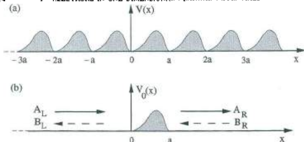
Fig. 7 Schematic representation of the periodic potential V(x) of a one-dimensional crystal (a), and of the potential V_0(x) within the unit cell (b).
