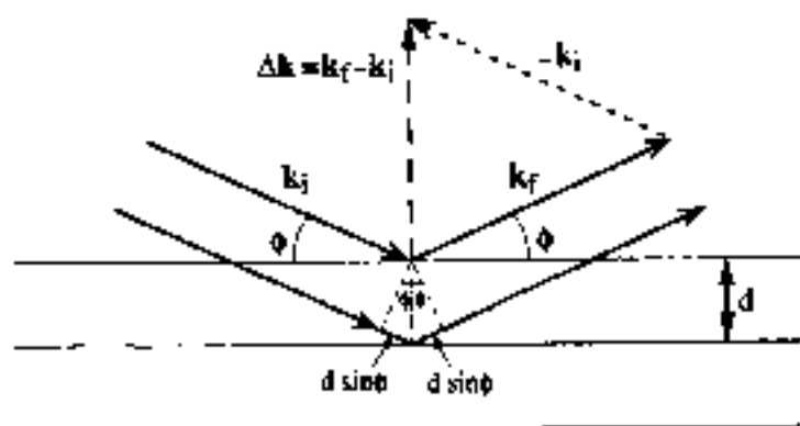
Fig. 4. Waves reflected from successive planes reinforce if 2d \sin \phi equals an integer number n\lambda of wavelengths. The geometrical construction of \Delta \mathbf{k} = \mathbf{k}_f - \mathbf{k}_i is also provided.
