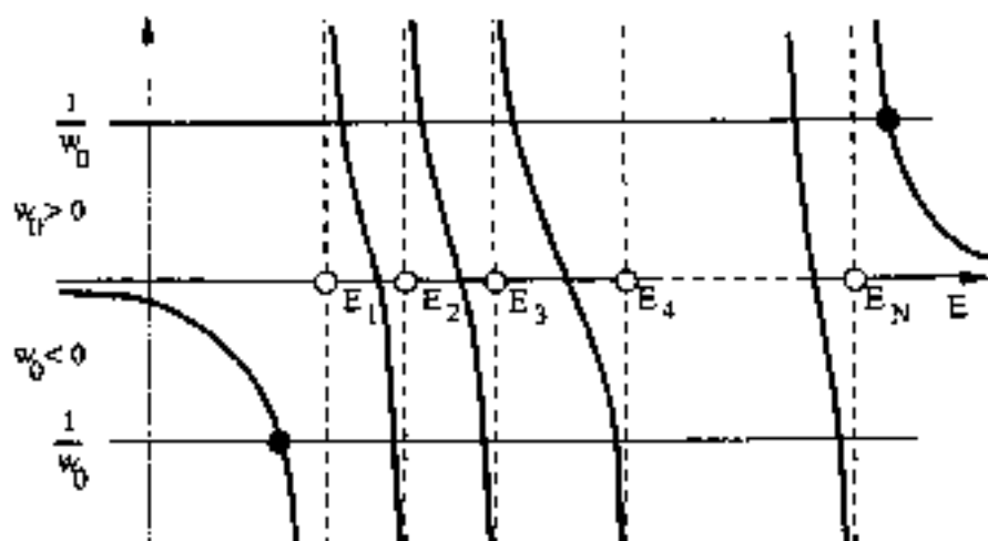
Fig. 18 Graphical solution of Eq. (85) of the text and formation of split-off states.
