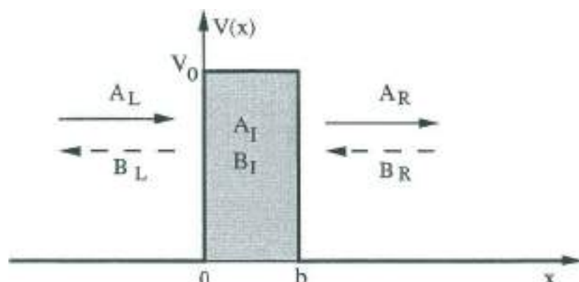
Fig. 5 Potential barrier of height V_0 and width b connecting two leads at zero potential
