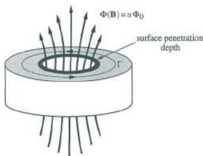
Fig. 20 Quantization of the magnetic flux through a multiply-connected superconductor with a ring shape.
