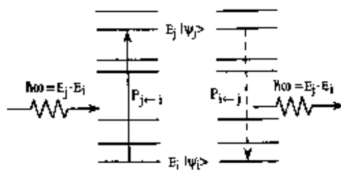
Fig. 1 Schematic representation of the radiative transition probability between a pair of electronic states |\psi_i\rangle and |\psi_j\rangle , of energy E_i and E_j ; any transition between these two states involves the absorption or the emission of a photon with energy \hbar\omega = E_j - E_i .
