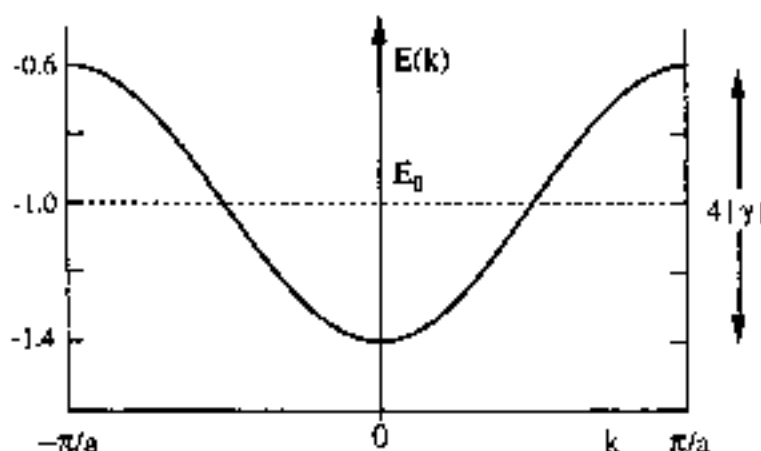
Fig. 9 Energy band E(k) = E_0 + 2\gamma \cos ka for a tight-binding model with s single orbital per site and nearest neighbour interactions; in the figure E_0 = -1 \text{ eV} and \gamma = -0.2 \text{ eV} .
