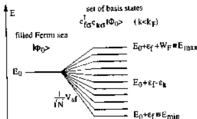
Fig. 10 Representation of the Anderson Hamiltonian on the basis of states formed by |\Phi_0\rangle and c_{f\sigma}^\dagger c_{k\sigma} |\Phi_0\rangle with k < k_F , and connected by the hybridization interaction V_{sf}/\sqrt{N} .
