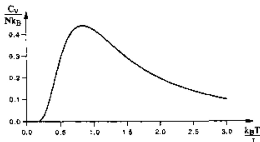
Fig. 6 Specific heat of a linear chain of spins coupled by exchange interaction in the Ising model.
