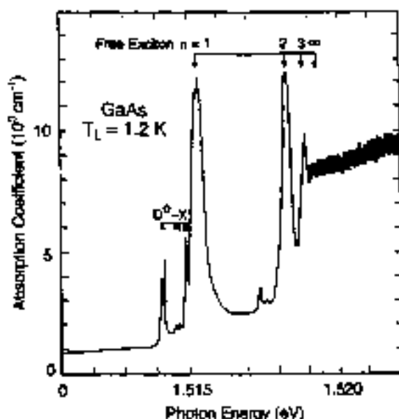
Fig. 2 Absorption spectrum at 1.2 K of a pure sample of GaAs containing residual donors. The n = 1, 2, 3 exciton peaks and the extrapolated energy gap are indicated by arrows. The peak D^0 - X corresponds to the creation of an exciton ( X ) bound to a neutral donor ( D^0 ) [from R. G. Uhrich and C. Wesbuch, unpublished; C. Wesbuch, Thesis, Université Paris VII, 1977].
