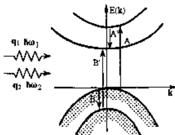
Fig. 9 Model band structure for estimating the absorption coefficient due to two-photon absorption. We indicate schematically by AA' and BB' possible second order processes contributing to the transition of an electron from the top of the valence band to the bottom of the conduction band [energy conservation and Pauli exclusion principle in the intermediate states are not operative, similarly to the discussion of Fig. 7]
