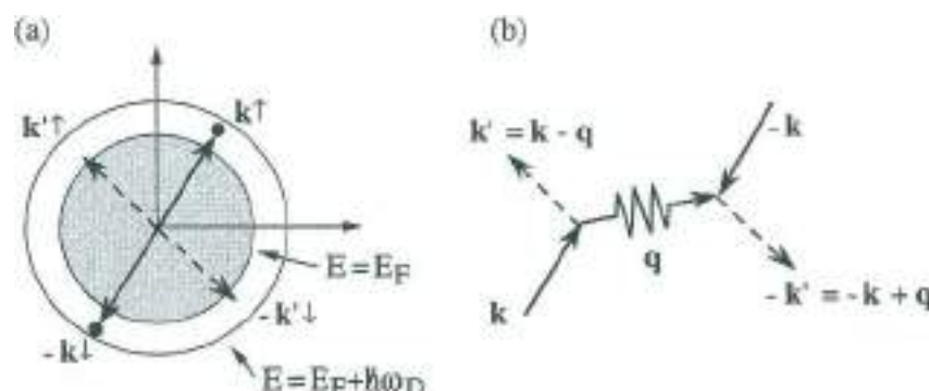
Fig. 7 (a) Schematic representation of a single Cooper pair, added to the ground-state of a free-electron gas. Two "extra electrons" in the pair state (\mathbf{k}\uparrow, -\mathbf{k}\downarrow) scatter freely to the pair states (\mathbf{k}'\uparrow, -\mathbf{k}'\downarrow) in the energy region E_F < E_k, E_{k'} < E_F + \hbar\omega_D , where the phonon-mediated attractive interaction is operative, and form a bound Cooper pair. (b) Schematic representation of the scattering of two electrons with wavevectors (\mathbf{k}, -\mathbf{k}) into the state (\mathbf{k}', -\mathbf{k}') via the emission and subsequent absorption of a phonon of momentum \hbar\mathbf{q} .
