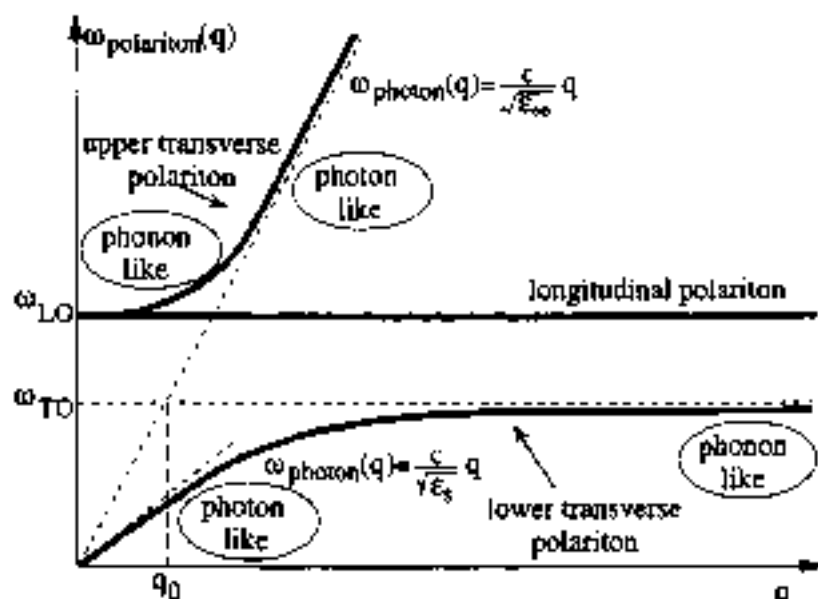
Fig. 10 Schematic description of polaritons. The dispersion curves of uncoupled transverse phonons and photons are shown by dashed lines; q_0 is the crossing point q_0 = \omega_{LO}/(c/\sqrt{\epsilon_\infty}) . Dispersion curves of the longitudinal phonon and transverse polaritons are shown by solid lines. In the lower polariton branch, the character of the dispersion curve changes from photon-like for q < q_0 to phonon-like for q > q_0 ; in the upper branch, the character changes from phonon-like to photon-like as q increases.
