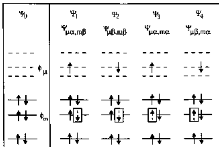
Fig. 2 Schematic representation of Hartree-Fock occupied and virtual states (here supposed to be discrete) of a closed-shell electronic system. In the four trial excited states \Psi_1, \Psi_2, \Psi_3, \Psi_4 , an electron is promoted from the occupied orbital \phi_m(\mathbf{r}) to the virtual orbital \phi_\mu(\mathbf{r}) .
