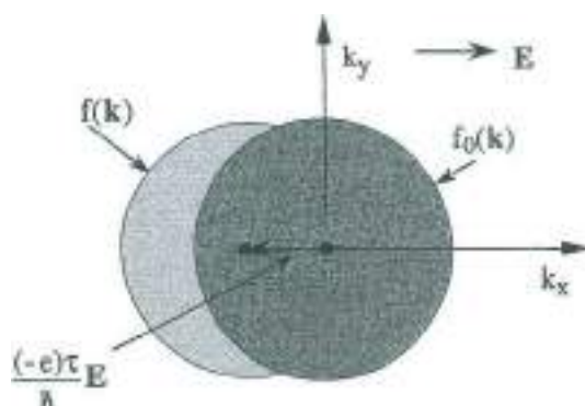
Fig. 8 Schematic representation of the equilibrium distribution function f_0(\mathbf{k}) and of the non-equilibrium distribution function f(\mathbf{k}) \approx f_0(\mathbf{k} + e\tau\hbar^{-1}\mathbf{E}) in the presence of a static electric field \mathbf{E} . The effect of the field is to shift the whole Fermi sphere by -e\tau\hbar^{-1}\mathbf{E} in the \mathbf{k} space. For sake of clarity of the figure, the value of -e\tau\hbar^{-1}\mathbf{E} has been magnified and taken of the same order as k_F .
