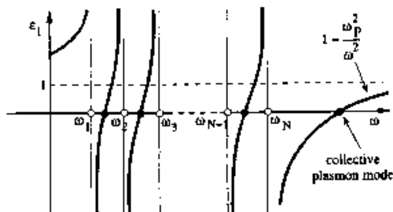
Fig. 10 Qualitative behaviour of the real part of the dielectric function of a system with proper frequencies \omega_n (indicated by white circles) in the interval [\omega_1, \omega_N] . Since \epsilon_1(q, \omega) is an even function of \omega , only the part \omega > 0 is indicated; the zeros of \epsilon_1(q, \omega) are indicated by black circles: notice the split-off collective state.
