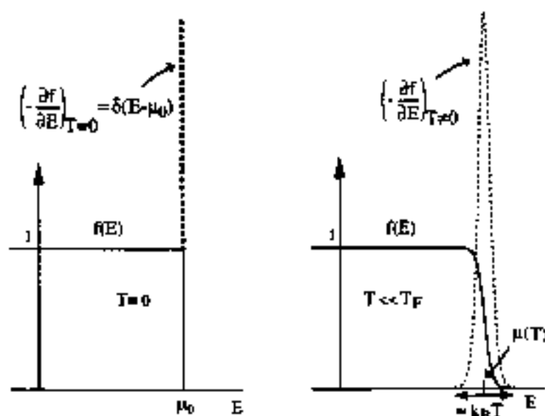
Fig. 4 The Fermi-Dirac distribution function f(E) and energy derivative (\partial f/\partial E) at T = 0 and at a finite temperature T , with T \ll T_F . \mu_0 denotes the chemical potential \mu(T) at T = 0 .
