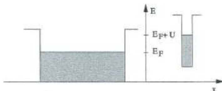
Fig. 5 Schematic representation of the linearized Thomas-Fermi approximation. On the left we have represented a metal with Fermi energy E_F , and density-of-states n(E_F) (per unit volume and both spin directions). On the right we have represented an (isolated) piece of the same metal, with all band structure rigidly shifted by a superimposed energy U . When the contact is established between the reservoir on the left and the (small) sample on the right, the Fermi energy of the sample equalizes E_F ; as a consequence, the induced electron density in the sample is n_{\text{ind}} = -n(E_F)U .
