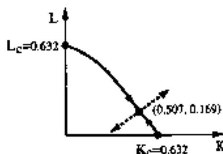
Fig. 14 Critical line representing the systems which are taken over by the renormalization transformations to the non-trivial fixed point (K^*, L^*) = (0.507, 0.169) . The critical line is the borderline between sub-critical and super-critical systems, which are taken over to the fixed points (K^*, L^*) = (0, 0) and (K^*, L^*) = (\infty, \infty) , respectively.
