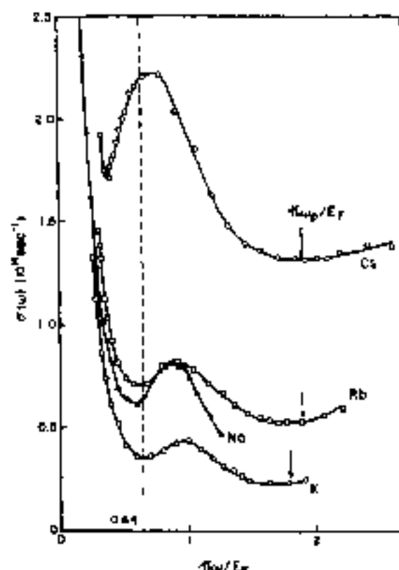
Fig. 6 Optical conductivity of the four alkali metals Na, K, Rb, Cs plotted against the normalized frequency \hbar\omega/E_F , where E_F is the free-electron Fermi energy [from N. V. Smith, Phys. Rev. B2, 2849 (1970); copyright 1970 by the American Physical Society].
