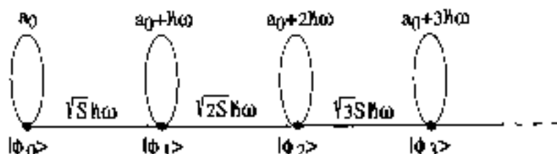
Fig. 20 Graphic representation of the Hamiltonian of the displaced oscillator on the basis of the states \{\phi_n\} of the oscillator at the origin. a_0 = (S + 1/2)\hbar\omega .
