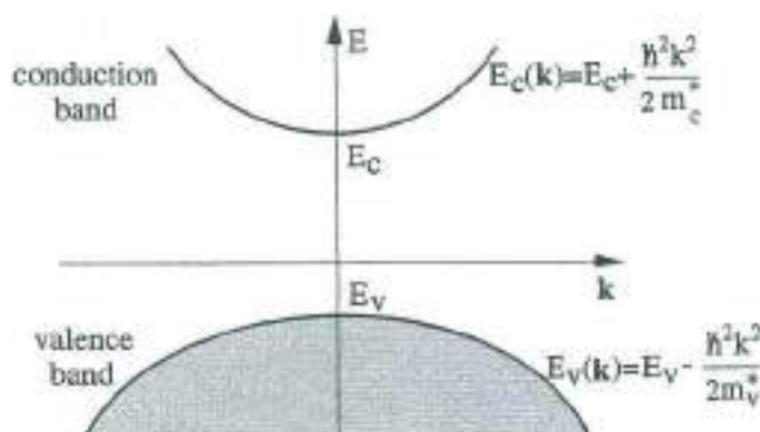
Fig. 3 Isotropic two-band model semiconductor: the valence band region has been shaded to remind its full occupancy by electrons at T = 0 .
