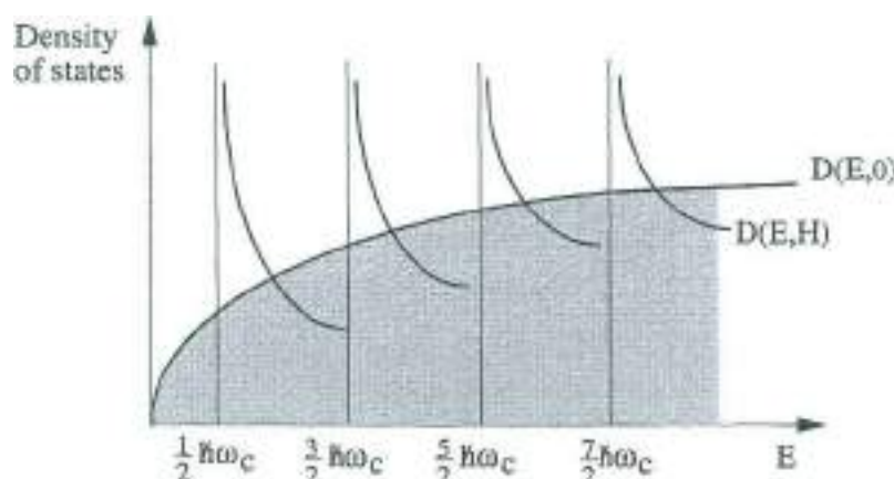
Fig. 3. Density-of-states of a three-dimensional electron gas in the presence and in the absence of a magnetic field
