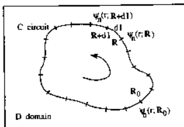
Fig. 10 Schematic representation of the sequence of states \psi_n(r; \mathbf{R}) as \mathbf{R} is changed along a circuit C drawn in the parameter space D ; it is assumed that no degeneracy point is encountered along the circuit.
