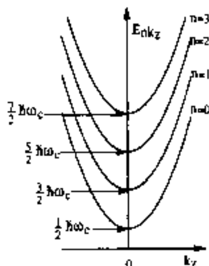
Fig. 2 Schematic representation of the energy levels for a three-dimensional electron gas in the presence of a magnetic field in the z -direction
