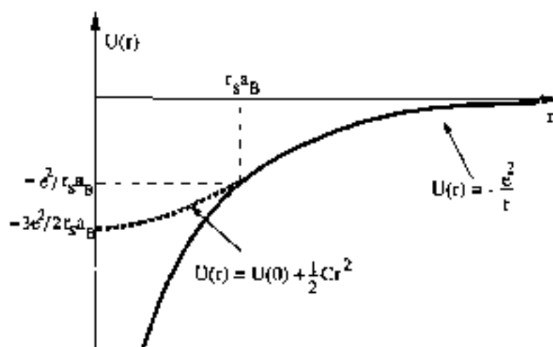
Fig. 5 Potential energy of an electron in the Coulomb field due to a uniformly charged sphere of radius r_s a_B and total charge +e . For 0 \leq r \leq r_s a_B the potential is quadratic, with "elastic constant" C = e^2/r_s^3 a_B^3 .
