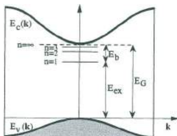
Fig. 3 Schematic energy band picture of a semiconductor in the two-band model representation. The lowest conduction band E_C(k) and the highest valence band E_V(k) are shown; the band extrema are supposed to occur both at k = 0 (the valence band region has been shadowed to remind its full occupancy by electrons). The series of excitons (with exciton wavevector equal to zero), converging towards the fundamental energy gap E_G , are indicated by straight lines: E_{ex} and E_b are the energy and the binding energy of the n = 1 exciton state.
