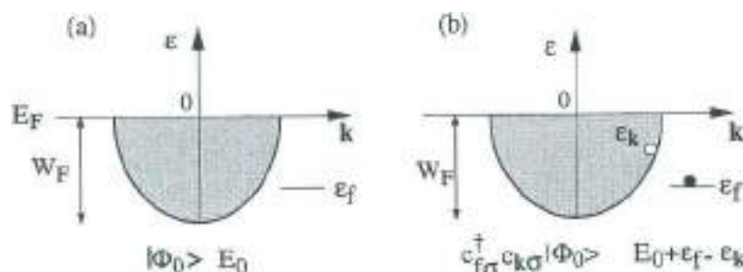
Fig. 9 (a) Schematic representation of the model Hamiltonian describing a magnetic impurity embedded in a sea of conduction electrons; the magnetic impurity is schematized with a single impurity orbital, which can accept no more than one electron. The ground-state wavefunction and energy of the filled Fermi sea are denoted by |\Phi_0\rangle and E_0 , respectively; W_F is the energy width of the conduction band occupied by electrons, and the Fermi level E_F is taken to be zero. (b) Schematic representation of the basis states interacting with the filled Fermi sea |\Phi_0\rangle , and leading to the formation of the singlet state in the Kondo problem.
