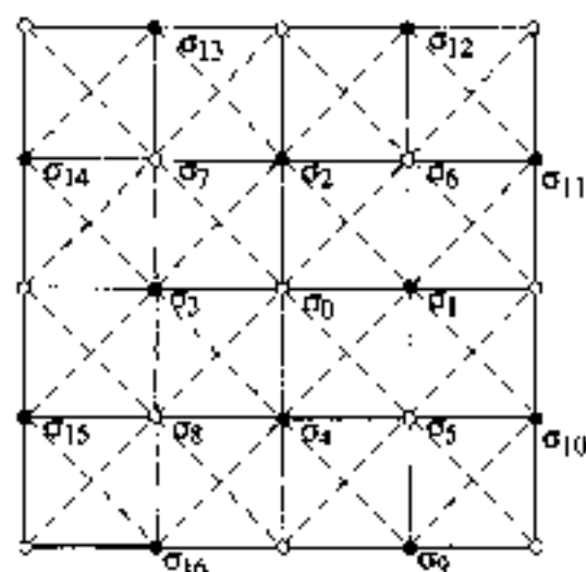
Fig. 13 Two-dimensional square lattice with nearest neighbour spin interactions (full lines) and next nearest neighbour spin interactions (dotted lines); labels of sites are introduced for the application of the renormalization procedure.
