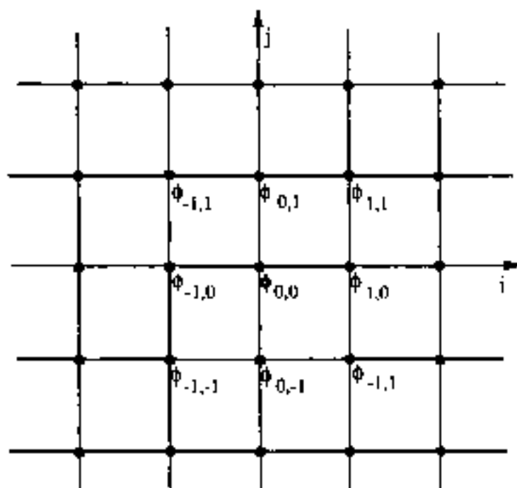
Fig. 15 Schematic graphical representation of a simple square lattice, with a single orbital per site, and nearest neighbour interactions; \phi_{i,j} indicates the orbital localized in the position (i,j) (the edge of the quadratum is taken as unit).
