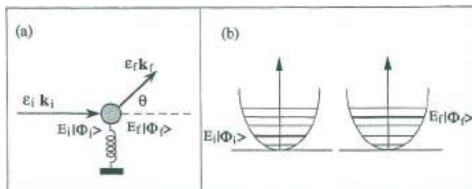
Fig. 13 (a) Diffusion of particles by a scatterer of finite mass M (an atom or a nucleus connected by a spring to a fixed center). (b) Schematic representation of initial and final energy levels and states of the harmonic oscillator scatterer, of given frequency \omega .
