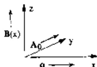
Fig. 16 Directions of the wavevector q , vector potential amplitude A_0 , and magnetic field
