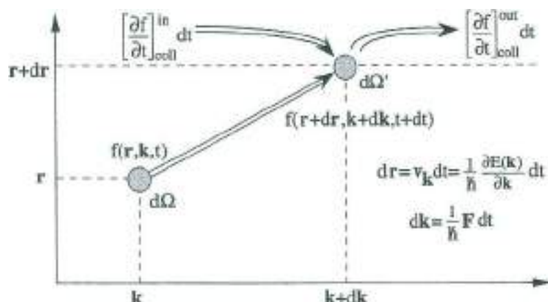
Fig. 7 Schematic representation of the conservation of the number of electrons moving in the space phase r, k . The region d\Omega around r, k at time t evolves into a new region d\Omega' , whose volume is the same as d\Omega (Liouville theorem). The distribution function f(r+dr, k+dk, t+dt) must thus equal f(r, k, t) supplemented by the net change [\partial f/\partial t]_{\text{coll}} dt = [\partial f/\partial t]_{\text{coll}}^{\text{in}} dt - [\partial f/\partial t]_{\text{coll}}^{\text{out}} dt of the number of electrons forced in and ejected out because of collision processes.
