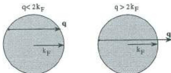
Fig. 7 Fermi sphere and excitations with wavevector transfer q < 2k_F and q > 2k_F : E(k+q) \approx E(k) is possible in the former case, but not in the latter
