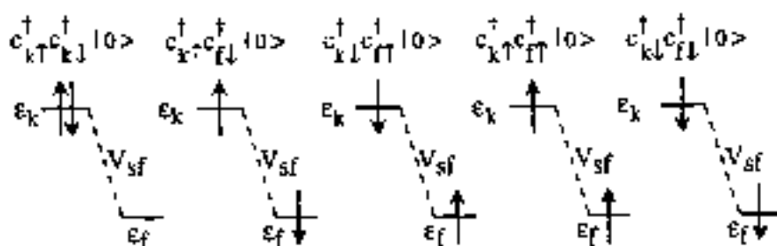
Fig. 8 Possible molecular states for two electrons in a two-orbital molecule (double occupancy of the localized orbital \psi_f is not possible in the U = \infty limit considered in the figure). The extended orbital \psi_k (of energy \varepsilon_k ) hybridizes with the localized orbital \psi_f (of energy \varepsilon_f ) via the matrix element V_{sf} , leading to the formation of the singlet molecular ground state.
