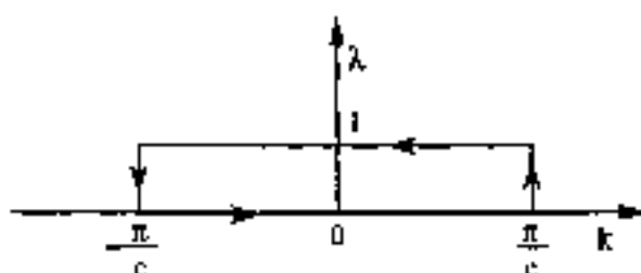
Fig. 12 Integration circuit for the calculation of electronic polarization with the Berry phase formalism.
