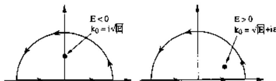
Fig. 12 Integration contour for evaluating the Green's function of the free-electron problem.
