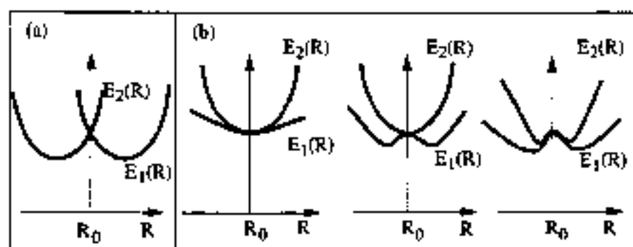
Fig. 3 Schematic representation of possible topologies of two adiabatic potential energy surfaces near a degeneracy point R_0 in nuclear coordinate space. In Fig. 3a we report the typical Jahn-Teller "conical intersection", with the presence of linear terms in R - R_0 . In Fig. 3b we report Renner-Teller "glancing intersections", with the absence of linear terms in R - R_0 , and positive or negative second derivatives. In general, terms linear in certain symmetry-breaking distortions are always possible for any type of degeneracy (except for Kramers degeneracy and some levels in linear molecules).
