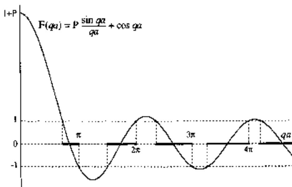
Fig. 2 Graphical solution of the compatibility equation P(qa)^{-1} \sin qa + \cos qa = \cos ka of the Kronig-Penney model. The dimensionless parameter P has been set equal to 3\pi/2 ; the qa regions where the compatibility equation is satisfied have been enhanced for convenience.
