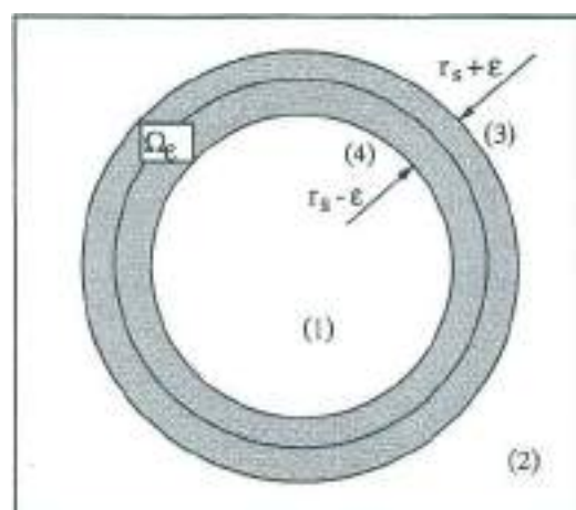
Fig. 11 Schematic representation of the four contributions (two volume contributions and two surface contributions) for the calculation of the matrix elements of the crystal Hamiltonian between augmented plane waves.
