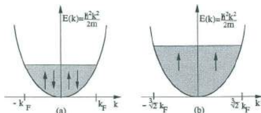
Fig. 3 (a) Schematic representation of the normal state of the free-electron gas. (b) Schematic representation of the fully polarized state of the free-electron gas.
