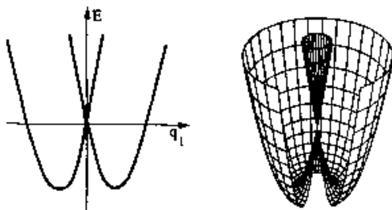
Fig. 5 Adiabatic potential-energy surfaces of the E \otimes e Jahn-Teller system. Fig. 5a shows the section of the two branches with the q_2 = 0 plane. When rotation by 2\pi through the energy axis is performed, the lower branch takes the shape of a "Mexican Hat" and the upper branch takes the shape of a conical "Wizard Hat" [from Lai-Sheng Wang, B. Niu, Y. T. Lee, D. A. Shirley, E. Chelchikyan, and E. R. Grant, J. Chem. Phys. 83, 6318 (1985), copyright 1990 by the American Physical Society].
