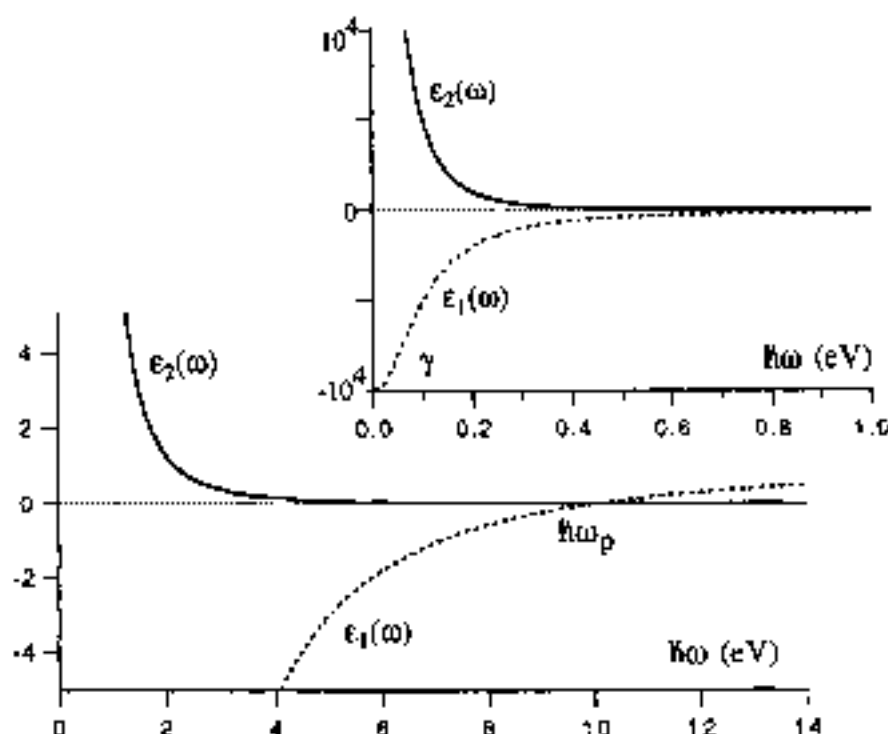
Fig. 3 Behaviour of real and imaginary part of the dielectric function of a free-electron gas with the Drude model; we have taken \hbar\omega_p = 10 eV and \gamma = \hbar/\tau = 0.1 eV.
