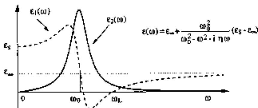
Fig. 13 Schematic behaviour of the real and imaginary part of the dielectric function \epsilon(\omega) of a polar crystal in the infrared region. Since \epsilon_1(\omega) and \epsilon_2(\omega) are even and odd functions of \omega , respectively, only the part \omega > 0 is indicated. For \eta \rightarrow 0^+ , the real part \epsilon_1(\omega) presents a pole at \omega = \omega_0 , while the imaginary part \epsilon_2(\omega) presents a \delta -like singularity at \omega = \omega_0 .
