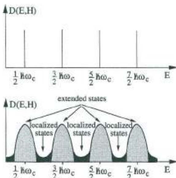
Fig. 14 Density-of-states D(E, H) of the two-dimensional electron gas in a magnetic field H : (a) in a pure material, the density-of-states is composed by a series of delta functions at the Landau levels; (b) in the presence of disorder, the Landau levels are broadened into bands, constituted by extended and localized states.
