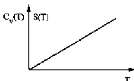
Fig. 5 Electronic contribution C_V(T) to the heat capacity of a metal at constant volume, as a function of temperature; the same expression holds for the electronic contribution to the entropy.
