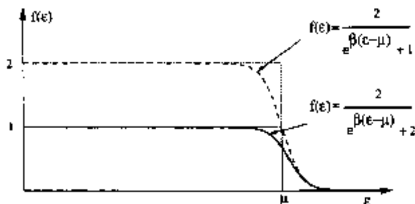
Fig. 7 Average occupation number (dashed line) for an orbital of energy \epsilon that can accept up to two electrons of either spin (standard Fermi-Dirac statistics). The average occupation number (solid line) for an orbital of energy \epsilon that can accept only one electron of either spin is also reported. For \epsilon - \mu \gg k_B T the two curves coincide.
