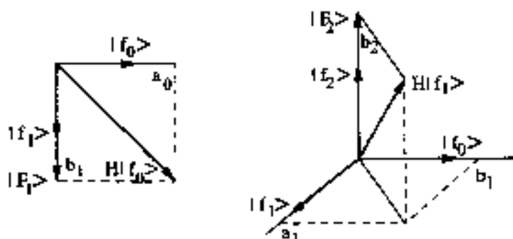
Fig. 13 Schematic representation of the Lanczos recursion procedure.
