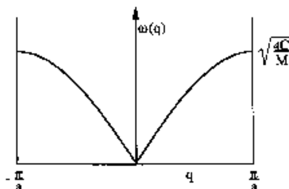
Fig. 2 Phonon dispersion curve for a monatomic linear lattice with nearest neighbour interactions only; the Brillouin zone is the segment between -\pi/a and +\pi/a .
