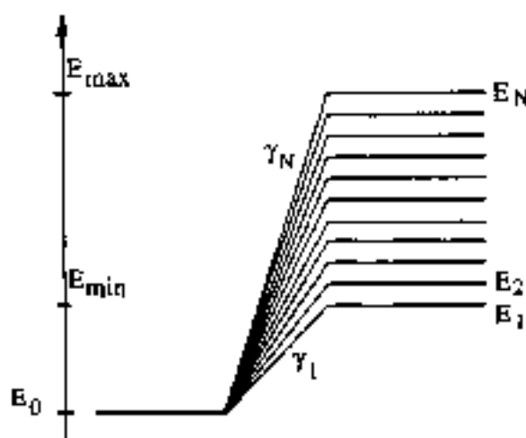
Fig. 16 Schematic representation of a system consisting of a discrete state of energy E_0 , interacting with a manifold of states in the energy range E_1 = E_{\min} and E_N = E_{\max} .
