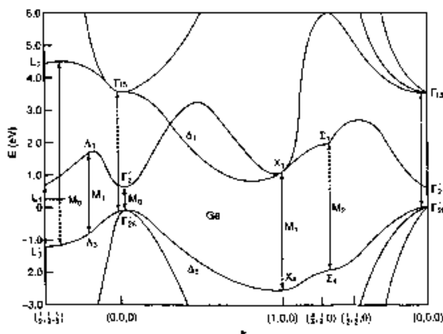
Fig. 3 Energy bands of germanium along symmetry directions, with the empirical pseudopotential method. The k wavevector is in units of 2\pi/a . Relevant direct interband edges are indicated by arrows [from D. Brust, J. C. Phillips and F. Bassani, Phys. Rev. Lett. 9 , 94 (1962), copyright 1962 by the American Physical Society].
