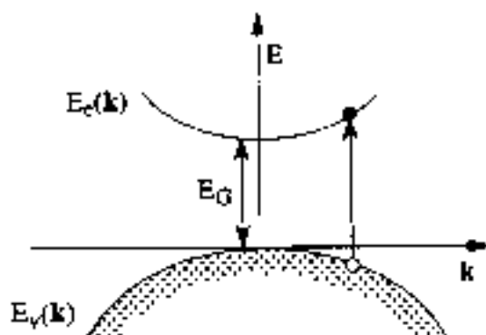
Fig. 2 Schematic representation of vertical transitions.
