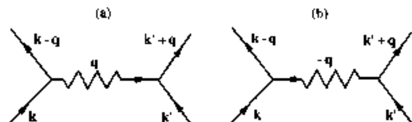
Fig. 25 Origin of the electron-electron interaction via phonons.
