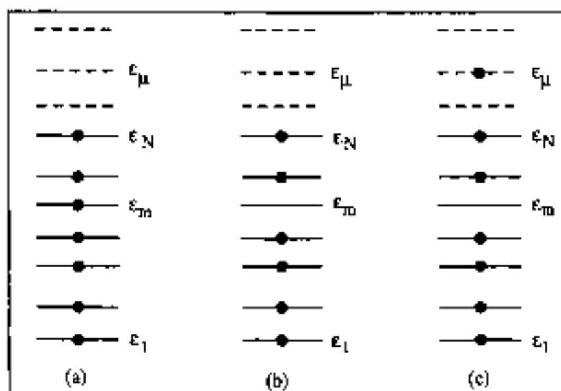
Fig. 1 Schematic representation (a) of occupied spin-orbitals (solid lines), in increasing order of energy, for the ground state of an N -electron system in the Hartree-Fock approximation; virtual spin-orbitals are represented with broken lines. (b) represents an ionized state of the N -electron system, with an electron removed from the occupied spin-orbital \psi_m (and transferred to infinity). (c) represents an excited state of the N -electron system, with an electron removed from the occupied spin-orbital \psi_m and transferred to the virtual spin-orbital \psi_\mu .
