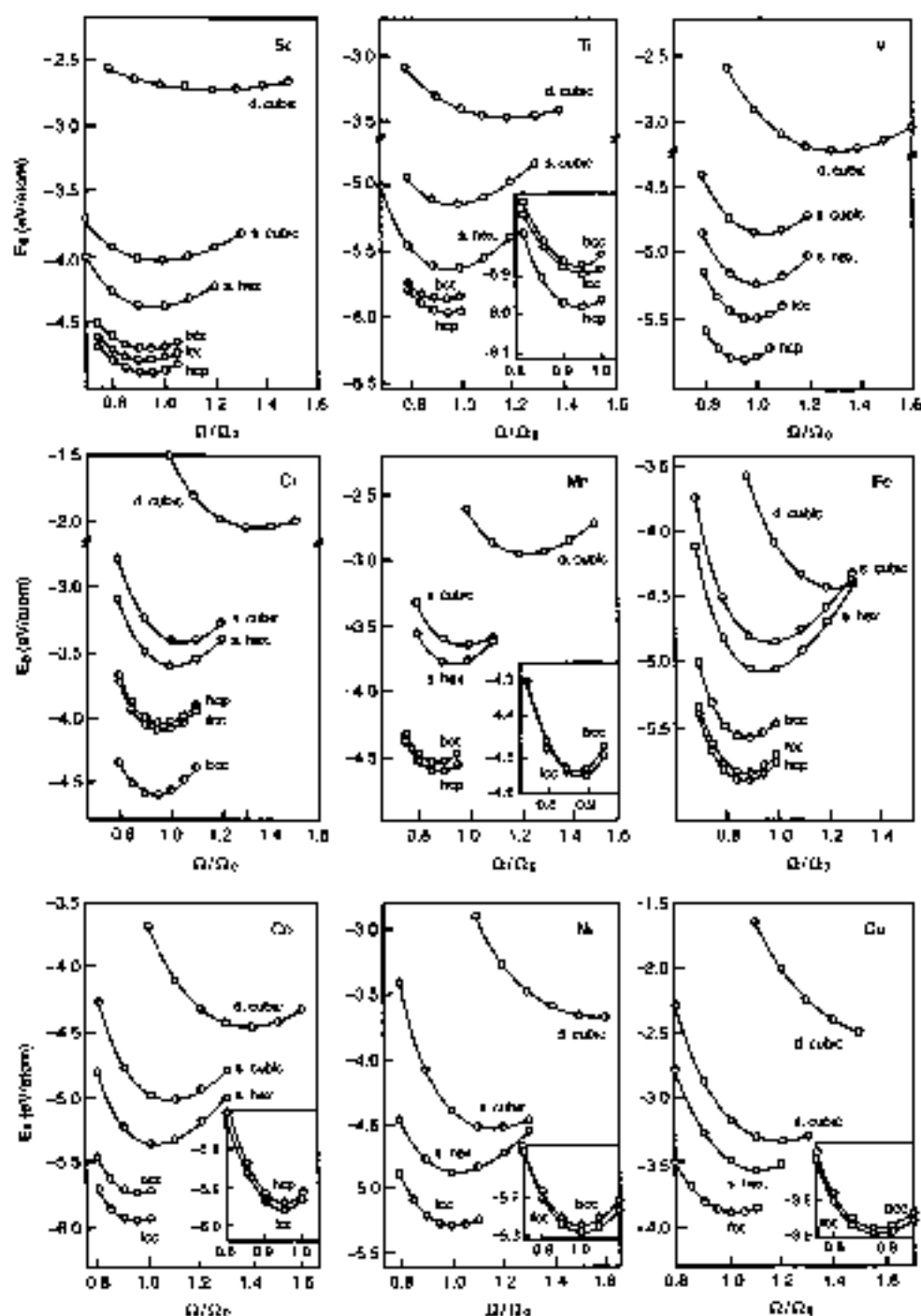
Fig. 15 Structural energy-volume curves in the 3d transition metals: cohesive energy (eV/atom) versus atomic volume normalized to the experimental atomic volume V_0 . Structures are fcc, bcc, hcp, simple hexagonal, simple cubic and diamond cubic; curves in insets are shown with expanded scales [from A. T. Paxton, M. Methfessel and H. M. Polatoglou, Phys. Rev. B41, 8127 (1990), copyright 1990 by the American Physical Society].
