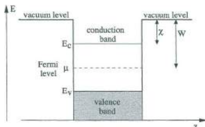
Fig. 8 Model semiconductor for the calculation of the thermionic emission. The work function W is the difference between the energy of an electron at rest in the vacuum and the chemical potential. The electronic affinity \chi is the energy difference between the vacuum level and the bottom of the conduction band. The work function W equals \chi + (E_C - \mu) .
