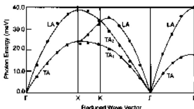
Fig. 5 Phonon dispersion curves of aluminum along symmetry directions. The solid lines represent the calculations of A. A. Quong and H. M. Klein, Phys. Rev. B46 , 10734 (1992) (copyright 1992 by the American Physical Society). Longitudinal and transverse acoustic branches are indicated by LA and TA (or TA 1 and TA 2 ), respectively. The experimental points are from the papers of C. Gilat and R. M. Nicklow, Phys. Rev. 143 , 487 (1966) and R. Stedman, S. Almqvist and G. Nilsson, Phys. Rev. 162 , 549 (1967).
