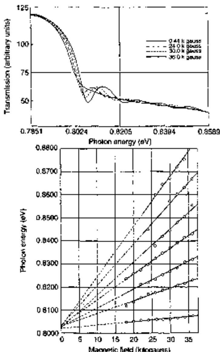
Fig. 5 (a) Oscillatory magneto absorption in germanium. (b) Energies of consecutive transmission minima as a function of the magnetic field. The lowest curve corresponds to transitions between Landau levels with n=0 ; the successive curves correspond to transitions with higher quantum states of both conduction and valence bands (from S. Zwerdling and B. Lax, Phys. Rev. 106 , 51 (1957), copyright 1957 by the American Physical Society).
