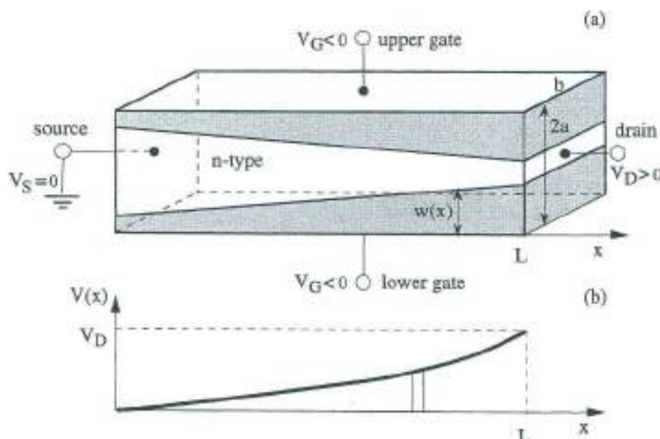
Fig. 9 (a) Model for a semi-quantitative account of the I-V characteristics of a junction field-effect transistor. (b) Voltage between source and drain.
