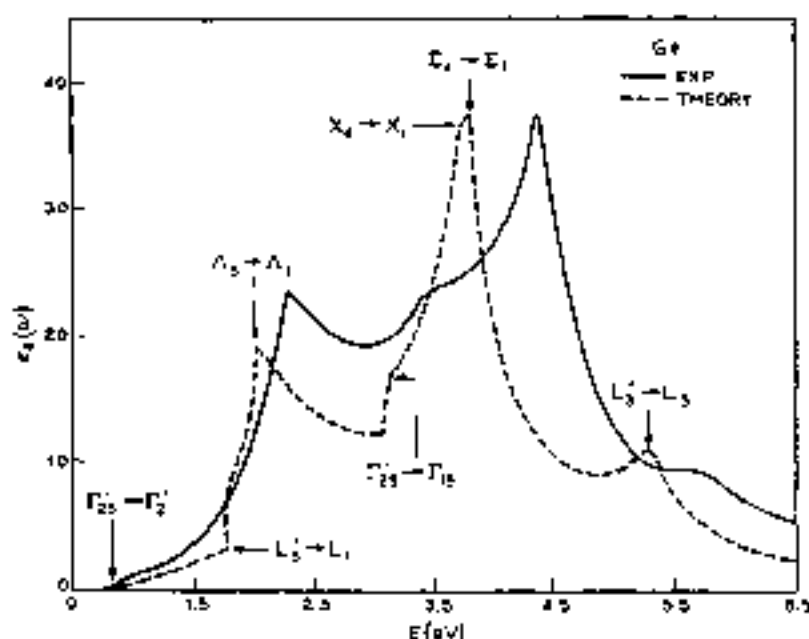
Fig. 4 Spectral structure of \epsilon_2(\omega) (solid line) compared with the theoretical results of interband transitions for Ge (dashed line with edges emphasized to account for critical points) [from D. Brust, J. C. Phillips and F. Bassani, Phys. Rev. Lett. 9 , 94 (1962) and D. Brust, Phys. Rev. 134 , A1337 (1964), copyright 1964 by the American Physical Society].
