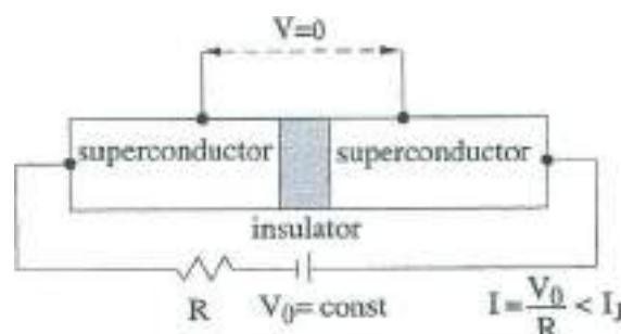
Fig. 23 Schematic illustration of the dc Josephson effect, a direct supercurrent (up to a maximum value I_J ) flows without dissipation through the insulating layer.
