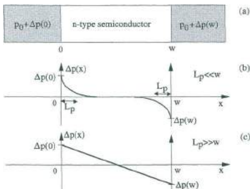
Fig. 11 (a) Schematic representation of an n-type semiconductor, with hole concentration p_0 + \Delta p(0) for x < 0 and p_0 + \Delta p(w) for x > w , we assume \Delta p(0) > 0 and \Delta p(w) < 0 . (b) Distribution of excess holes (and excess electrons) as a function of x in the case L_p \ll w . (c) Distribution of excess holes (and excess electrons) as a function of x in the case L_p \gg w .
