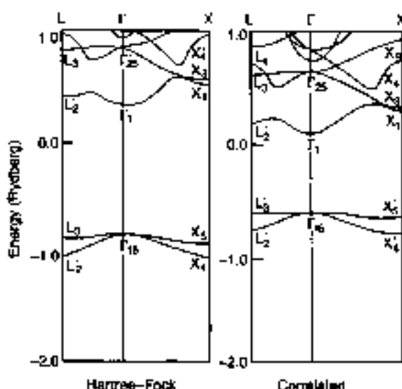
Fig. 7 Hartree-Fock and correlated energy bands of NaCl. The state \Gamma_{15} is the top of the valence bands and the state \Gamma_1 is the bottom of the conduction bands [from A. B. Kunz, Phys. Rev. B26, 2056 (1982); copyright 1982 by the American Physical Society].
