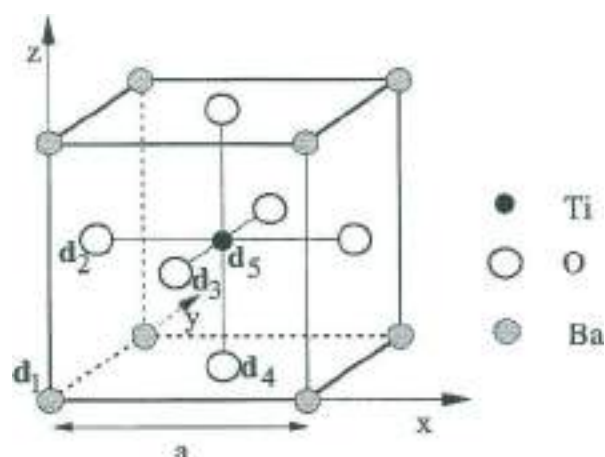
Fig. 8 Cubic structure of barium titanate: the end points of the basis vectors d_1, d_2, d_3, d_4 and d_5 are also indicated.
