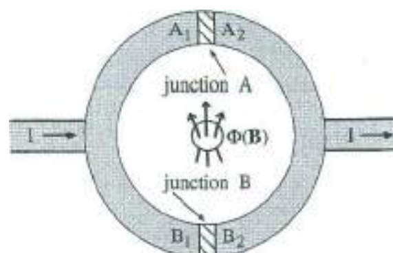
Fig. 24 Schematic diagram of a dc superconducting quantum interference device for detecting an enclosed magnetic field of flux \Phi(\mathbf{B}) .
