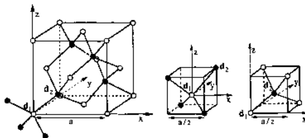
Fig. 6 Diamond structure with the two for composing sublattices represented with white and shaded circles, respectively. The inversion of bond orientations in the two for sublattices is illustrated in the two smaller cubes, which provide the four atoms surrounding d_1 = 0 and d_2 = (a/4)(1, 1, 1) .
