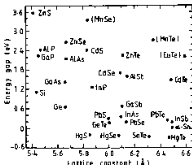
Fig. 1 Energy gap and lattice constant of some semiconductor crystals at room temperature [from M. Jaxon "Physics and Applications of Semiconductor Microstructures" (Clarendon Press, Oxford 1989); by permission of Oxford University Press].
