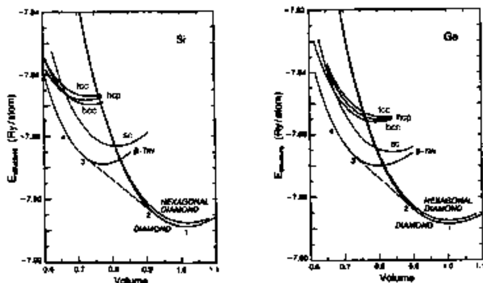
Fig. 9 Total energy curves for seven structures of Si and Ge, as a function of the atomic volume (normalized to the experimental volume). Dashed line is the common tangents of the energy curves for the diamond phase and the \beta -tin phase [from M. T. Yin and M. L. Cohen, Phys. Rev. B26, 5668 (1982), copyright 1982 by the American Physical Society].
