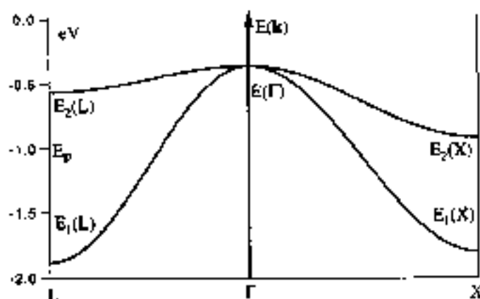
Fig. 3 Schematic behaviour of p -like bands in a fcc crystal lattice with the tight-binding method; E_p is the energy of the p -like orbitals. The values of E(\Gamma) , E_1(X) , E_2(X) , E_1(L) , E_2(L) are given by Eqs. (14) of the text. The figure refers to the case E_p = -1 eV, V(pp\sigma) = 0.2 eV and V(pp\pi) = -0.02 eV.
