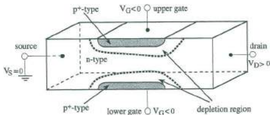
Fig. 8 Schematic illustration of the junction field-effect transistor
