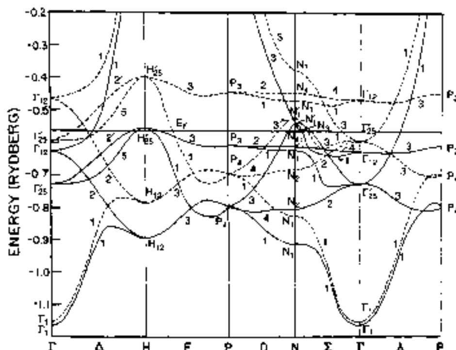
Fig. 15 Energy bands in ferromagnetic iron along some lines of high symmetry; solid lines are majority-spin states, dashed are minority-spin states [from J. Callaway and C. S. Wang, Phys. Rev. B16, 2095 (1977); copyright 1977 by the American Physical Society]
