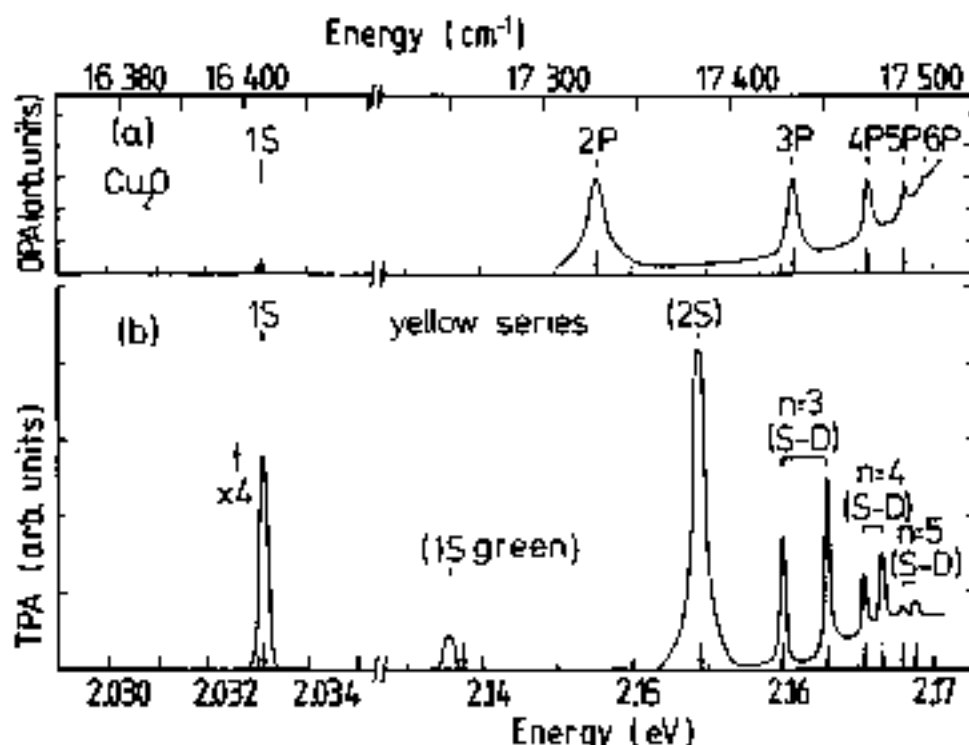
Fig. 12 One-photon absorption (OPA) and two-photon absorption (TPA) spectra of \text{Cu}_2\text{O} . One-photon data at 4.2 K are from J. B. Grin and S. Nikitine, J. Phys. (Paris) 23 , 159 (1962). Two-photon data at 4.5 K are from Ch. Uihlein, D. Fröhlich and R. Kenkies, Phys. Rev. B 28 , 2731 (1981) (copyright 1981 by the American Physical Society). The arrows indicate the calculated exciton energies in an appropriate multiband model.
