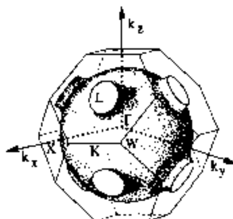
Fig. 14 Brillouin zone for the face-centered cubic lattice and Fermi surface of copper.
