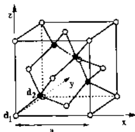
Fig. 9 Crystal structure of diamond and zincblende; the end-points of the vectors d_1 and d_2 of the bases are also indicated. In the diamond structure the two sublattices are occupied by atoms of the same type; in the zincblende structure the two sublattices are occupied by different types of atoms.
