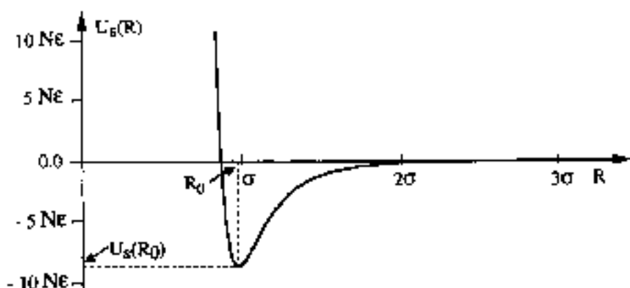
Fig. 3 Behaviour of the crystal energy U_c(R) for a rare-gas solid as a function of the nearest neighbour distance R . The minimum of the curve provides the cohesive energy U_c(R_0) and the equilibrium position R_0 . The slope is related to the applied pressure, and the curvature near R_0 is related to the bulk modulus.
