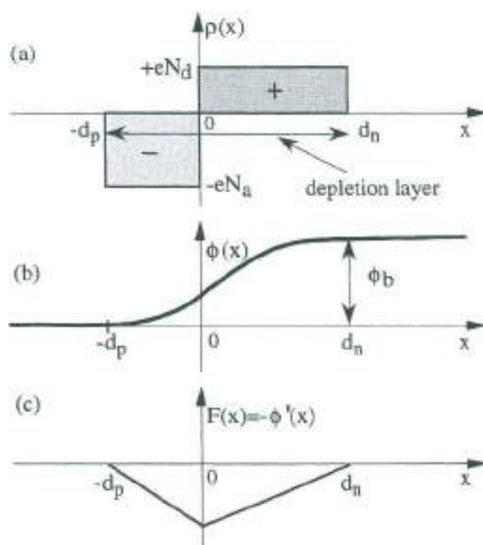
Fig. 2 Charge density \rho(x) at a pn junction in the depletion layer approximation, electrostatic potential \phi(x) , and internal electric field F(x) .
