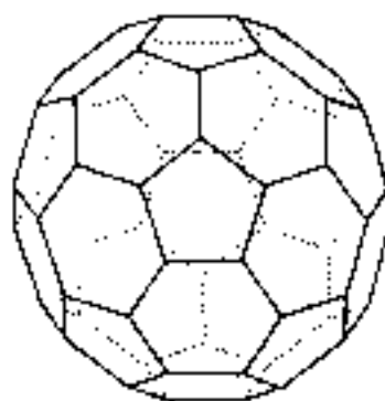
Fig. 12 The structure of C_{60} molecule in its regular truncated icosahedron geometry. The polygon has 60 vertices and 32 faces, 12 of which are pentagonal and 20 hexagonal. The bond lengths forming pentagons are 1.47 \text{ \AA} ; the bond lengths common to two hexagons are 1.41 \text{ \AA} [from P. Milani, Rivista del Nuovo Cimento 1B, N 11 (1996); copyright 1996 by Società Italiana di Fisica].
