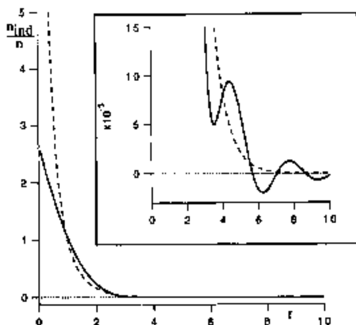
Fig. 8 Behaviour of the induced electron density n_{ind}(r) , relative to the unperturbed density n , when a point charge +e is inserted in a metal at the origin. The Thomas-Fermi approximation is indicated with a dashed line; the Lindhard approximation with a continuous line ( r is in units of the Bohr radius a_0 ; k_F = 1 a_0^{-1} ; r_s = 1.92 ).
