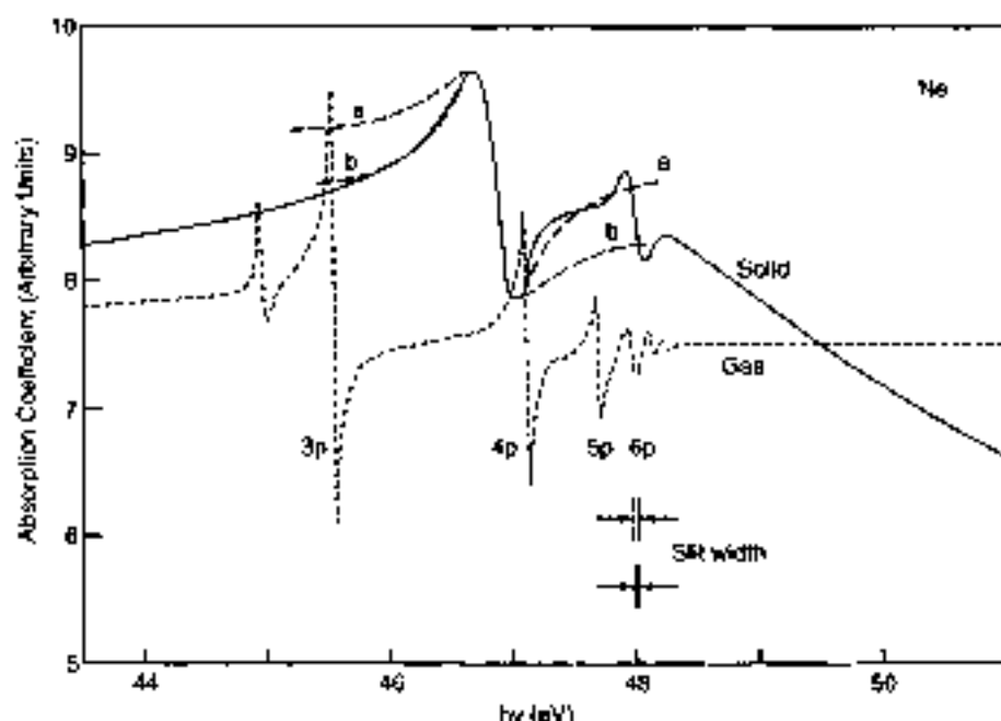
Fig. 15 Absorption spectrum of solid Ne (solid curve) and gaseous Ne (dashed curve). The theoretical curves a and b are fitted on the absorption cross-section of Fano, with two different sets of parameters (see Table 1) [from R. Haensel, G. Keitel, C. Kunz and P. Schreiber, Phys. Rev. Lett. 25 , 206 (1970); copyright 1970 by the American Physical Society].
