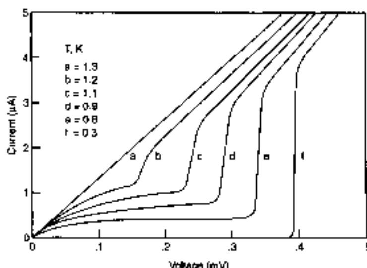
Fig. 10 Typical current-voltage characteristics of an Al-Al 2 O 3 -Al superconductor-insulator-superconductor junction (only quasiparticle tunneling current is considered). The onset of the sharp break in the curves for T < T_c occurs when eV \approx 2\Delta(T) ; the critical temperature is T_c = 1.26 K, and 2\Delta_0/k = 0.379 mV [from D. N. Langenberg, D. J. Scalapino and B. N. Taylor, Proc. IEEE 54, 560 (1966), copyright 1996 IEEE].
