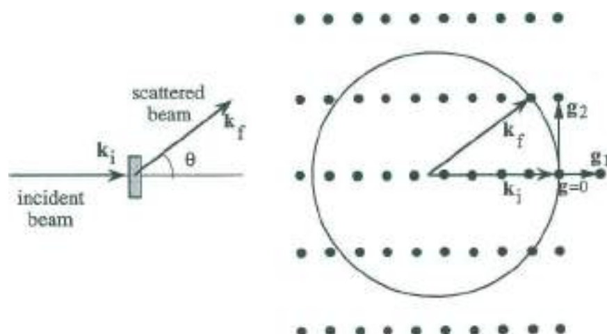
Fig. 5 Scattering of X-rays and Ewald construction.
