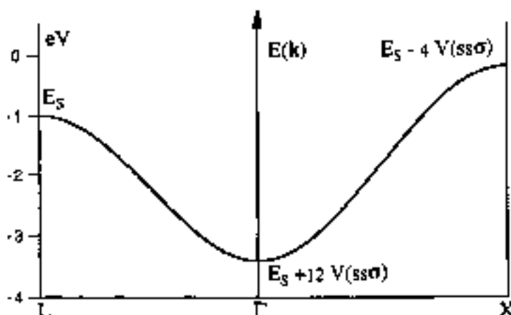
Fig. 2. Schematic behaviour of an s -like band in a fcc crystal lattice with the tight-binding method: E_s is the energy of the s -like orbital, V(ss\sigma) < 0 is the two-center potential integral between nearest neighbour s -like atomic orbitals. The values of the wavevector \mathbf{k} at the points \Gamma , X and L are \mathbf{k} = 0 , \mathbf{k} = (2\pi/a)(1, 0, 0) and \mathbf{k} = (2\pi/a)(1/2, 1/2, 1/2) , respectively. In the figure, we have taken E_s = -1 eV and V(ss\sigma) = -0.2 eV.
