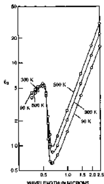
Fig. 4 Imaginary part of the dielectric function of copper at different temperatures [from S. Roberts, Phys. Rev. 118 , 1509 (1960); copyright 1960 by the American Physical Society.]
