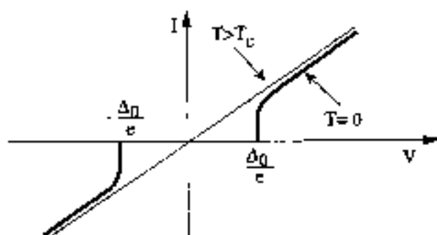
Fig. 12 Schematic representation of the I - V characteristics of a normal metal-insulator-superconductor junction at zero temperature and above the critical temperature; \Delta_0 is the energy gap parameter of the superconductor. At finite temperature 0 < T < T_c the presence of thermally excited electrons contribute to smear out and shift the strongly nonlinear T = 0 current-voltage characteristics.
