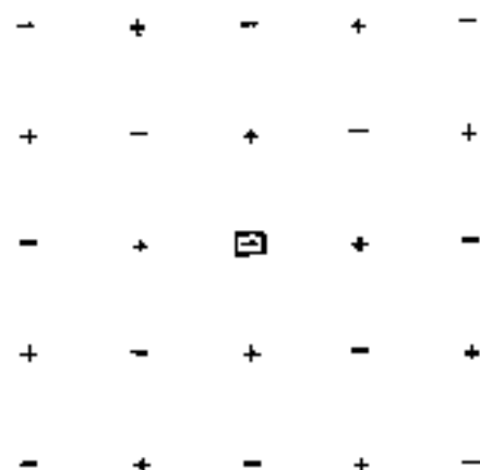
Fig. 6. Schematic representation of a two-sublattice ionic crystal in the point ion approximation, for the calculation of the Madelung constant. The ion at the origin has been surrounded by a box.
