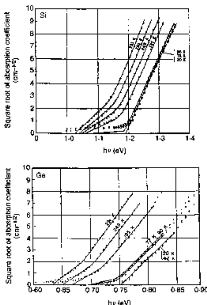
Fig. 8 (a) Indirect transitions in silicon; dots indicate experimental measurements; the full lines are calculated using Eq. (29) of the text. [from G. G. Macfarlane and V. Roberts, Phys. Rev. 98 , 1665 (1955); copyright 1955 by the American Physical Society] (b) Indirect transitions in germanium [from G. G. Macfarlane and V. Roberts, Phys. Rev. 87 , 1714 (1955); copyright 1955 by the American Physical Society].
