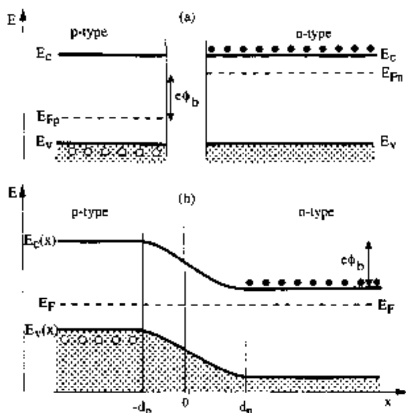
Fig. 1 (a) Energy bands and Fermi levels in two physically separated p-type and n-type non-degenerate semiconductors. The majority carriers (electrons in n-type and holes in p-type regions) are indicated by full dots and empty dots, respectively, while minority carriers are not indicated for simplicity. (b) Energy band profile and Fermi level across the pn junction at equilibrium.
