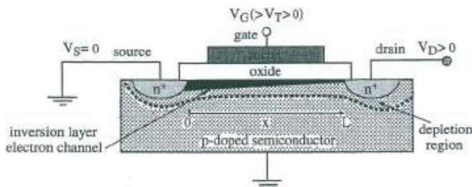
Fig. 20 Schematic representation of a MOSFET transistor.
