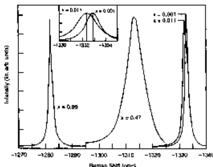
Fig. 9 Raman spectra of diamond specimens ^{12}\text{C}_{1-x}^{13}\text{C}_x for x = 0.001 , x = 0.011 (natural composition), x = 0.47 and x = 0.89 : the change of the optical mode frequency \omega_0 with the isotopic composition x follows approximately the M^{-1/2} dependence, where M is the average atomic mass [from R. Vogelgesang, A. K. Ramdas, S. Rodriguez, M. Grimsditch and T. R. Anthony, Phys. Rev. B54, 3989 (1996); copyright 1996 by the American Physical Society].
