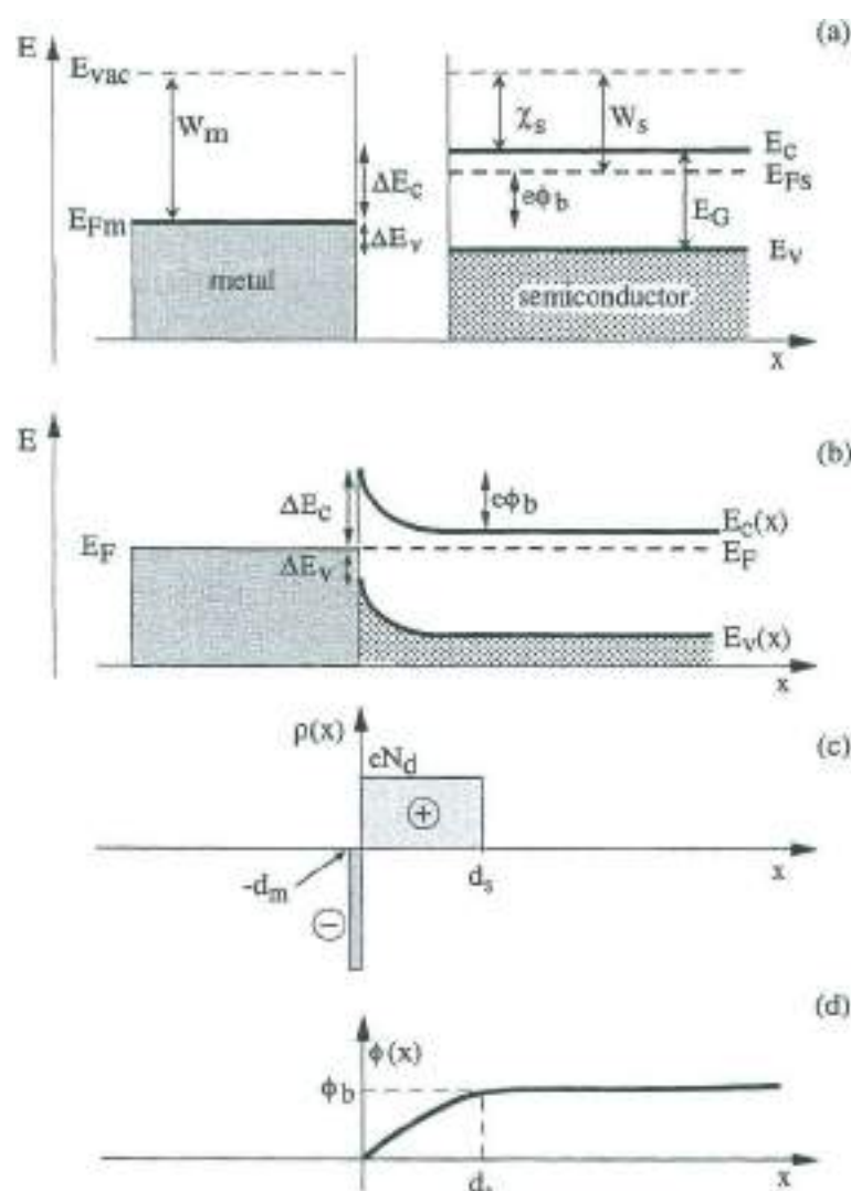
Fig. 13 (a) Energy bands of separated metal and n-type semiconductor. It is assumed that the Fermi energy of the metal is lower than the Fermi energy of the semiconductor, but still within the forbidden energy gap of the semiconductor. (b) Energy band profile for the metal and the n-type semiconductor in contact at equilibrium. The space charge region \rho(x) and the internal electrostatic potential barrier \phi(x) are also shown.
