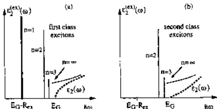
Fig. 10 Schematic diagram of the imaginary part of the dielectric function for first-class and second-class optical transitions neglecting exciton effects (dashed lines) and including exciton effects (solid lines).
