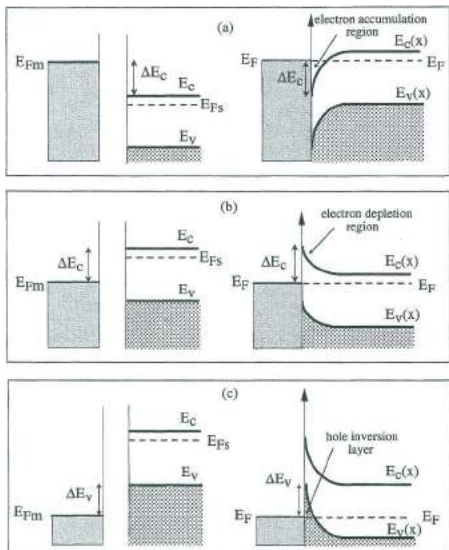
Fig. 12 Energy band diagrams of a metal and an n-doped semiconductor before contact (left panel) and after contact (right panel); the energy bands of the two materials before contact are referred to the vacuum level. Case (a) corresponds to an ohmic contact. Case (b) corresponds to a blocking contact. Case (c) corresponds to the formation of an inversion layer. The energy difference between the Fermi level of the metal and the band edges of the semiconductor are indicated by \Delta E_C and \Delta E_V ; these discontinuities are the same before and after contact.
