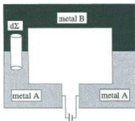
Fig. 14 Standard bimetallic circuit for illustration of the Peltier effect, the temperature is uniform throughout the whole circuit
