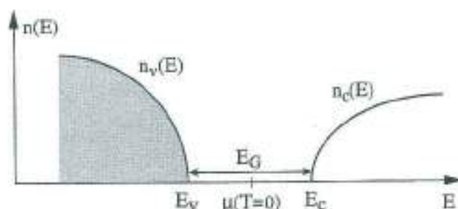
Fig. 2 Schematic representation of the density-of-states of an intrinsic semiconductor. The top of the valence band is E_v and the bottom of the conduction band is E_c . The energy gap is E_c - E_v = E_g ; the Fermi level at zero temperature lies at the middle of the band gap.
