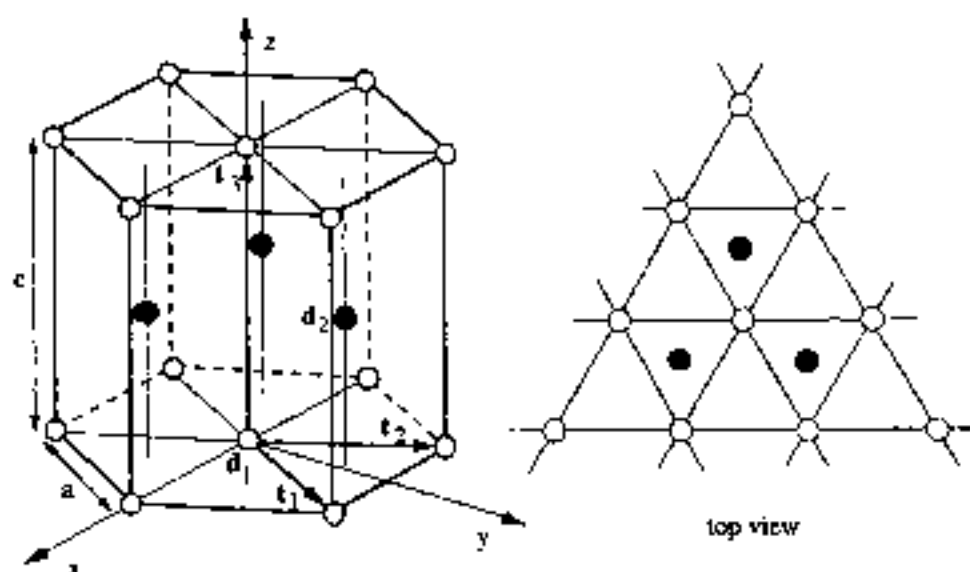
Fig. 13 Hexagonal close-packed structure. The primitive translation vectors t_1, t_2, t_3 and the end points of the basis vectors d_1 and d_2 , given in Eqs. (15) of the text, are also indicated. The top view of the structure is also shown for convenience.
