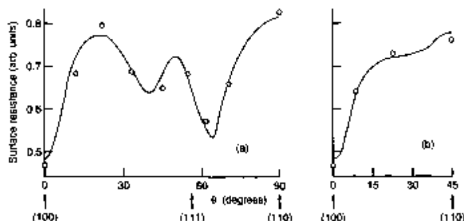
Fig. 10 Surface resistance (arbitrary units) versus orientation for copper, in the extreme anomalous region. The angle \theta subtends from (100) to the (110) direction, following two different arrangements (a) and (b) [from A. B. Pippard, Phil. Trans. Roy. Soc. (London) A250, 325 (1957)].
