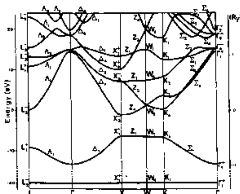
Fig. 5 Band structure of solid lithium hydride with the orthogonalized plane wave method [from S. Baroni, G. Pastori Parravicini and G. Pezzica, Phys. Rev. B 32 , 4077 (1985), copyright 1985 by the American Physical Society].
