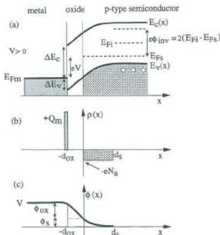
Fig. 18 Energy band profile, charge density and electrostatic potential of an ideal metal-oxide-semiconductor structure under (moderate) positive bias of the metal.
