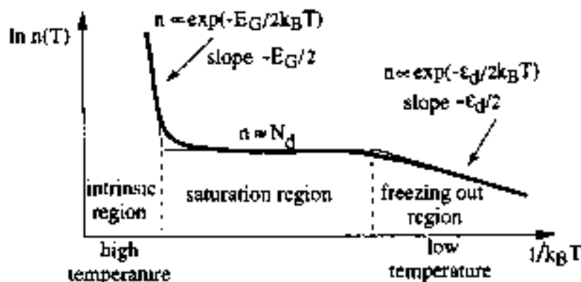
Fig. 8. Schematic variation of the electron concentration as a function of 1/k_B T in an n-type semiconductor with N_d donor impurities per unit volume.
