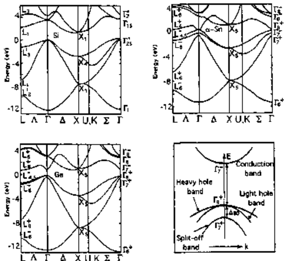
Fig. 8 Band structure for silicon, germanium and grey-tin [from J. R. Chelikowsky and M. L. Cohen, Phys. Rev. B 14, 556 (1976), copyright 1976 by the American Physical Society]. The typical band structure of cubic semiconductors near the gap at k = 0 is also schematically reported; \Delta_{so} denotes the spin-orbit splitting.
