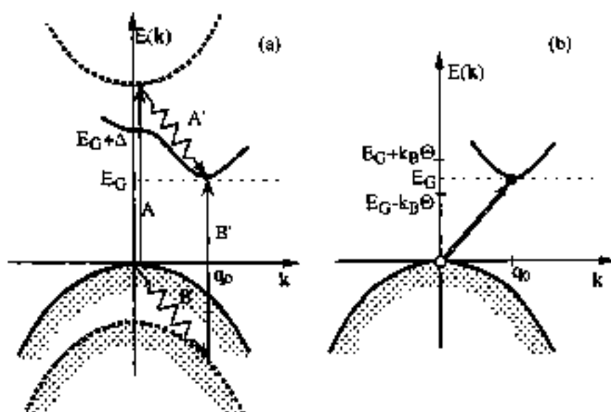
Fig. 7 Model band structure for estimating the absorption coefficient due to indirect transitions. In Fig. 7a we indicate schematically possible second-order processes contributing to the scattering of an electron from the top of the valence band \psi_{vk_1} ( k_1 \approx 0 ) to the bottom of the conduction band \psi_{ck_2} ( k_2 \approx q_0 ). The mechanism A A' consists of a direct transition from \psi_{vk_1} to a virtual state \psi_{vk_2} (occupied or empty), followed by a phonon-assisted scattering to \psi_{ck_2} . The mechanism B B' consists of a phonon-assisted scattering from \psi_{vk_1} to a virtual state \psi_{vk_2} (occupied or empty), followed by a direct transition to \psi_{ck_2} (energy conservation and Pauli exclusion principle can be ignored in the virtual states, as discussed in the text). In Fig. 7b we indicate only the highest valence band and the lowest conduction band; near their respective edges, the second-order scattering amplitude (indicated with a double line) is taken as approximately constant. The energy thresholds for photon absorption, with absorption or emission of a phonon of energy k_B \Theta , are also indicated.
