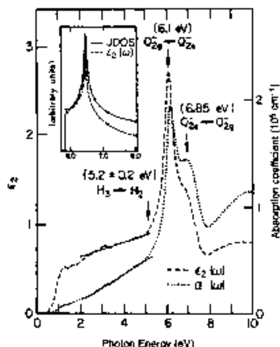
Fig. 8. Imaginary dielectric constant \epsilon_2(\omega) and absorption coefficient \alpha(\omega) due to interband electronic transitions in hexagonal boron nitride from experimental measurements [from D. M. Hoffman, G. L. Doll and P. C. Eklund, Phys. Rev. B 30 , 6051 (1984); copyright 1984 by the American Physical Society]. The inset is the joint density of states and \epsilon_2(\omega) calculated in the two-dimensional approximation near the saddle point singularity.
