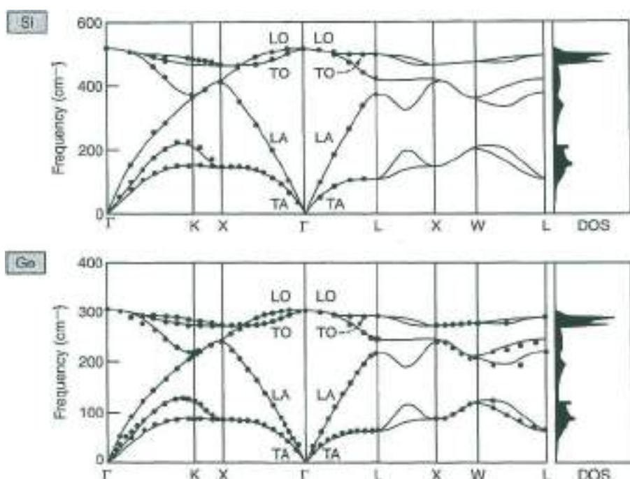
Fig. 6 Phonon dispersion curves and density-of-states of Si and Ge calculated by P. Giannozzi, S. de Gironcoli, P. Pavone and S. Baroni, Phys. Rev. B43 , 7231 (1991) (copyright 1991 by the American Physical Society). Longitudinal and transverse acoustic (or optical) modes are indicated by LA and TA (LO and TO), respectively. The experimental points are from G. Dolling, in "Inelastic Scattering of Neutrons in Solids and Liquids" edited by S. Eklund (IAEA, Vienna 1963) Vol.II, p.37; G. Nilsson and G. Nelin, Phys. Rev. B3 , 364 (1971) and Phys. Rev. B6 , 3777 (1972). Conversion to meV units can be done noting that 1 \text{ cm}^{-1} = 0.124 \text{ meV} .
