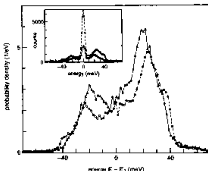
Fig. 15 Absorption probability density for \alpha -iron (circles, dashed line) and stainless steel (triangles, solid line), after removing the elastic peak. The inset shows the raw data [from W. Sturlach, T. S. Toellner, E. E. Alp, X. Zhang, M. Ando, Y. Yoda, S. Kikuta, M. Sato, C. W. Kimball and B. Dabrowski, Phys. Rev. Lett. 74 , 3832 (1995); copyright 1995 by the American Physical Society].
