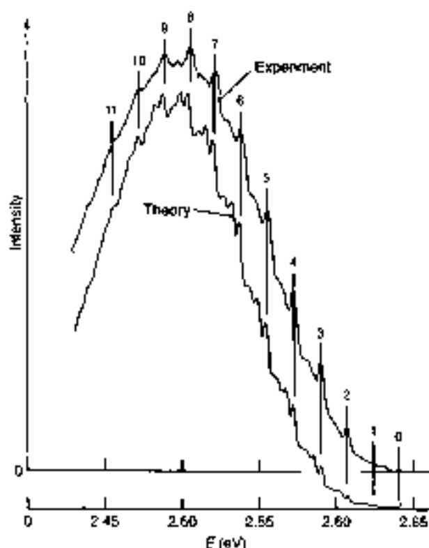
Fig. 19 Comparison of the theoretical and experimental luminescence intensity of AgBr at 2 K containing residual iodine atoms. [Experimental results are taken from W. Czaia, J. Phys. C 16, 3197 (1983); theoretical results and interpretation are taken from A. Tessa, C. Cesaia, A. Quattropani and P. Schwendimann, J. Phys. C 20, 1253 (1987)]
