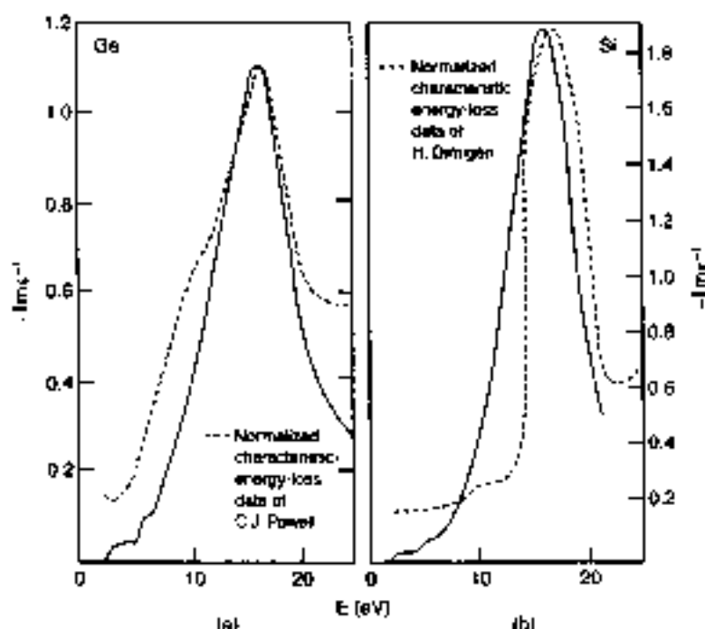
Fig. 12 Comparison of the energy-loss function -\text{Im } 1/\epsilon(0, \omega) obtained from the results of optical measurements and characteristic-energy-loss experiments for Ge and Si [from H. R. Philipp and H. Ehrenreich, Phys. Rev. 129 , 1550 (1963); copyright 1963 by the American Physical Society].
