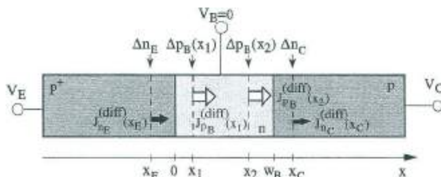
Fig. 7 Effect of applied emitter and collector potentials on the concentration of minority carriers at the borders of the space-charge regions. The electron diffusion current at x = x_E , the hole diffusion current at x = x_1 and x = x_2 , and the electron diffusion current at x = x_C are indicated (the signs of the currents correspond to V_E > 0 and V_C < 0 ). The emitter current is J_E = J_{pE}^{(diff)}(x_E) + J_{pB}^{(diff)}(x_1) ; the collector current is J_C = J_{pB}^{(diff)}(x_2) + J_{nC}^{(diff)}(x_C) ; the base current is J_B = J_E - J_C .
