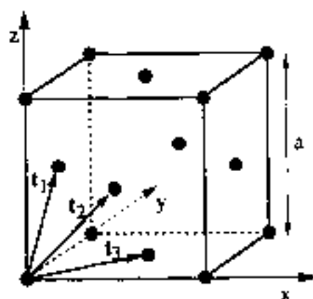
Fig. 4 Face-centered cubic lattice and primitive translation vectors t_1, t_2, t_3 given by Eq. (7) in the text.
