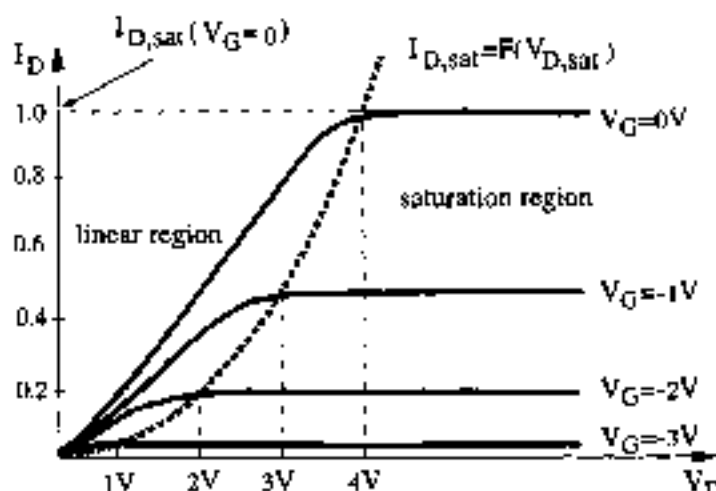
Fig. 10 Idealized I_D - V_D characteristics of a junction field-effect transistor. For V_D > V_{D,sat} the drain current remains constant. The current I_{D,sat}(V_G = 0) has been taken as the unit of current. The curve I_{D,sat} = F(V_{D,sat}) is given by Eq. (36) of the text. The parameters of the JFET of the figure are taken to be \phi_b = 1 V and V_p = 5 V. V_{D,sat} equals V_s - \phi_b - |V_G| .
