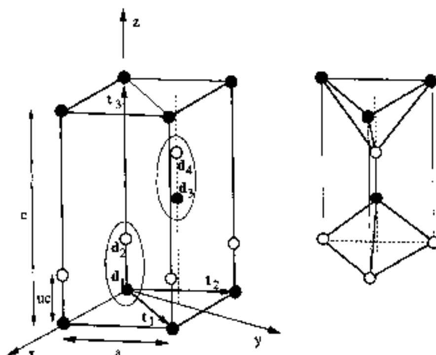
Fig. 14 Hexagonal wurtzite structure. The primitive translation vectors t_1, t_2, t_3 and the end points of the basis vectors d_1, d_2, d_3 and d_4 , given by Eq. (16) of the text, are indicated; the two molecules of the unit cell are encircled for convenience. The orientations of adjacent tetrahedra surrounding d_1 and d_4 are also shown
