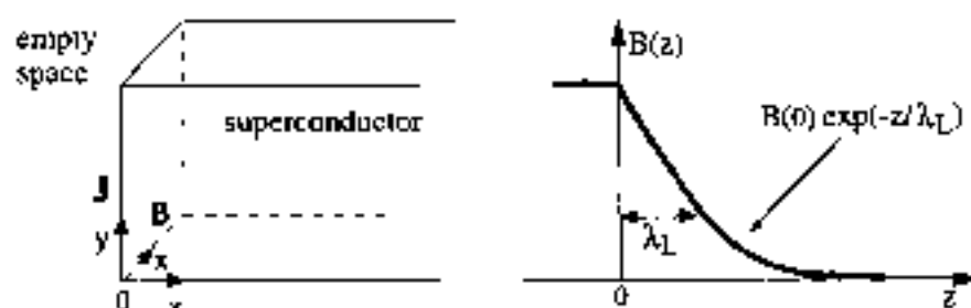
Fig. 16 Semi-infinite slab geometry for illustration of screening currents and penetration depth of the magnetic field parallel to the surface.
