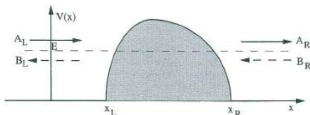
Fig. 4 Schematic representation of a potential (of finite range and arbitrary shape) connecting two leads at zero potential. Arrows indicate the wavevectors of the propagating plane waves (of energy E ), and A_L , B_L , A_R , B_R the amplitudes.
