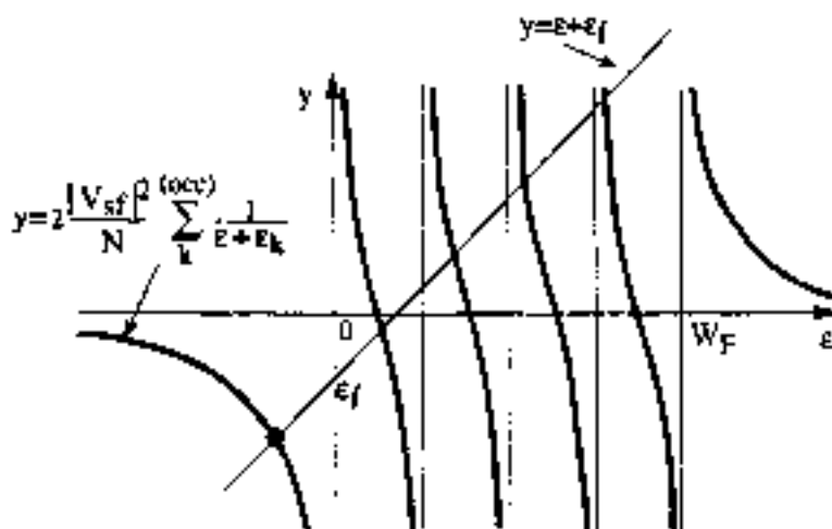
Fig. 11 Graphical solution of the eigenvalue problem for the Kondo effect (notice that \varepsilon_f < 0 and also 0 < -\varepsilon_k \leq W_F ).
