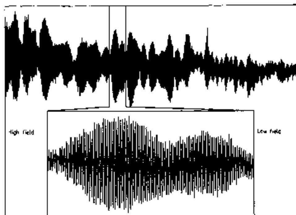
Fig. 10 Experimental de Haas-van Alphen magnetization oscillations for a sample containing randomly oriented particles of lithium dispersed in paraffin wax. The full trace covers the field range 12.9–7.9 T at a temperature of 20 mK. The portion of the trace between 11.1 and 10.8 T is shown expanded in the inset [from M. G. Hunt, P. H. P. Reinders and M. Springford, J. Phys. Condens. Matter 1 , 6589 (1989)].
