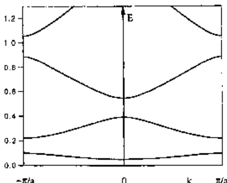
Fig. 3 Energy bands of lower energy in the Kronig-Penney model for P = 3\pi/2 . The energy E (in Rydberg) is plotted as a function of k in the first Brillouin zone: the value of the lattice parameter considered is a = 0.1a_B ( a_B Bohr radius)
