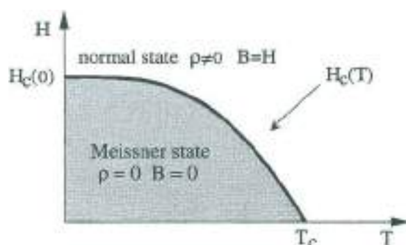
Fig. 3 Schematic phase diagram illustrating normal and superconducting regions of a type-I superconductor.
