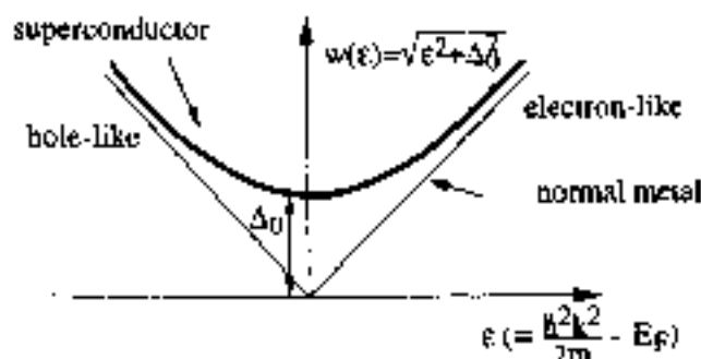
Fig. 10 Quasiparticle energy spectrum for the normal metal and for the superconductor at zero temperature.
