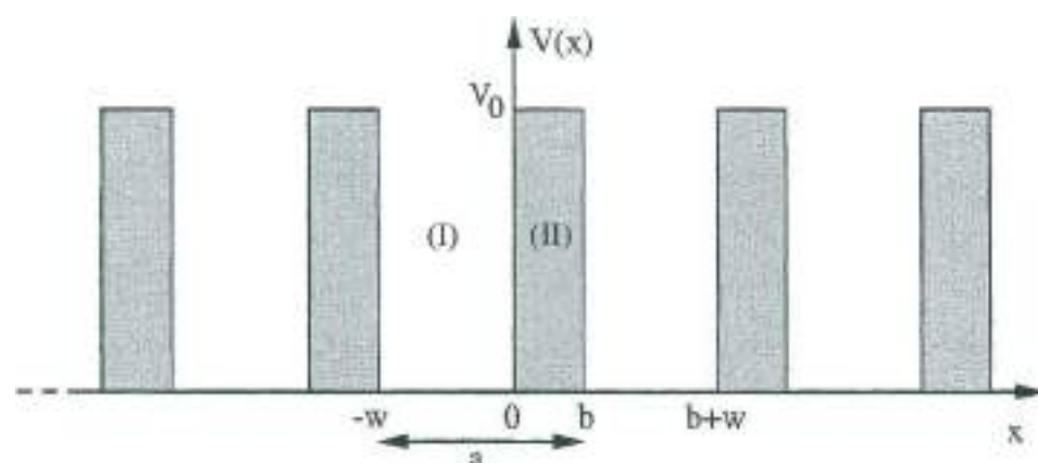
Fig. 1 One-dimensional potential formed by a periodic array of quantum wells.
