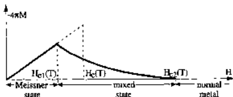
Fig. 6 Magnetization versus applied field H for a type-II superconductor. The equivalent area construction of the thermodynamic field H_T(T) is also illustrated.
