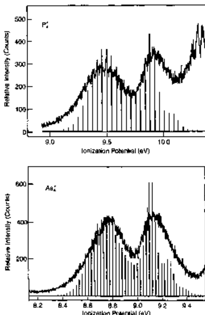
Fig. 23 Experimental photoelectron spectrum of P_4^+ (figure a) and As_4^+ (figure b), and best fit with a linear E \otimes e Jahn-Teller model [from Lai-Sheng Wang, H. Neu, Y. T. Lee, D. A. Shirley, E. Chelchikhani and E. R. Grant, J. Chem. Phys. 93 , 6318 (1990); copyright 1990 by the American Physical Society].
