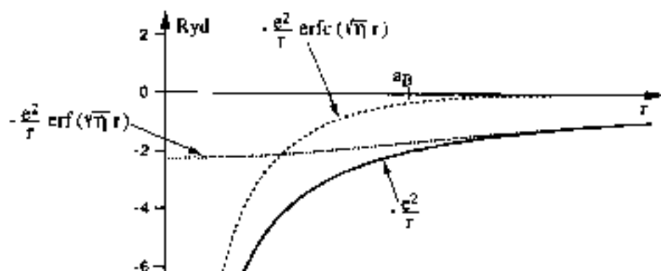
Fig. 5 Decomposition of the potential -e^2/r (singular at the origin and of long-range nature) into a contribution -(e^2/r)\text{erf}(\sqrt{\eta}r) (regular at the origin and of long-range nature) and a contribution -(e^2/r)\text{erfc}(\sqrt{\eta}r) (singular at the origin and of short-range nature). Energies are expressed in Rydbergs, length in Bohr radius units; we have chosen \sqrt{\eta} = 1/a_B^{-1} .
