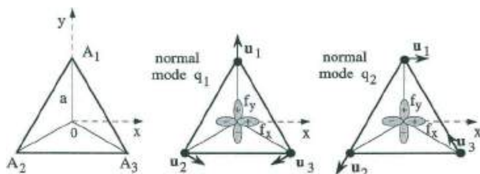
Fig. 4 Geometry of the regular triangular molecule and nuclear displacements of the degenerate vibrational mode \epsilon . The doublet of electronic states ( f_x, f_y ) centred at the origin is also indicated
