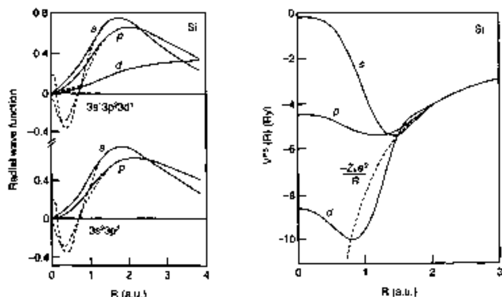
Fig. 8 (a) Comparison of the pseudowavefunction (solid lines) and the corresponding all-electron wavefunctions (dashed lines) for the configurations 3s^2 3p^2 and 3s^1 3p^2 3d^1 of silicon. (b) Non-local pseudopotential of Si for angular momentum l=0, 1, 2 . The dashed line denotes the Coulomb potential of a point-like atomic core [from M. T. Yin and M. L. Cohen, Phys. Rev. B 26 , 5663 (1982); copyright 1982 by the American Physical Society].
