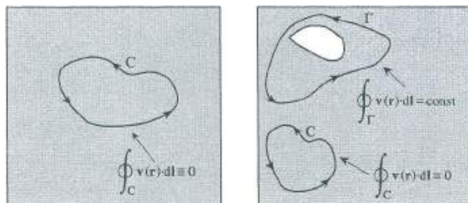
Fig. 17 Schematic illustration of a simply-connected domain and multiply-connected domain wherein it is defined an irrotational vector field, i.e. a field \mathbf{v}(\mathbf{r}) such that \text{curl } \mathbf{v}(\mathbf{r}) \equiv 0 . In Fig. (17a), we have \oint_C \mathbf{v}(\mathbf{r}) \cdot d\mathbf{l} \equiv 0 for any closed path C within the connected domain. In Fig. (17b), the circulation \oint_C \mathbf{v}(\mathbf{r}) \cdot d\mathbf{l} vanishes for any circuit C that does not enclose the hole, while \oint_{\Gamma} \mathbf{v}(\mathbf{r}) \cdot d\mathbf{l} \equiv \text{const} (in general different from zero) for any closed circuit \Gamma that encloses the hole. In either cases, we can construct the function \chi(\mathbf{r}) = \int_{P_0}^{P(\mathbf{r})} \mathbf{v}(\mathbf{r}') \cdot d\mathbf{l} and write \mathbf{v}(\mathbf{r}) = -\nabla \chi(\mathbf{r}) ; in the simply-connected geometry \oint_C \mathbf{v}(\mathbf{r}) \cdot d\mathbf{l} \equiv 0 and \chi(\mathbf{r}) is an ordinary single-valued function; in the multiply-connected geometry \oint_C \mathbf{v}(\mathbf{r}) \cdot d\mathbf{l} \neq 0 (in general) and \chi(\mathbf{r}) is a multiply-valued function.
