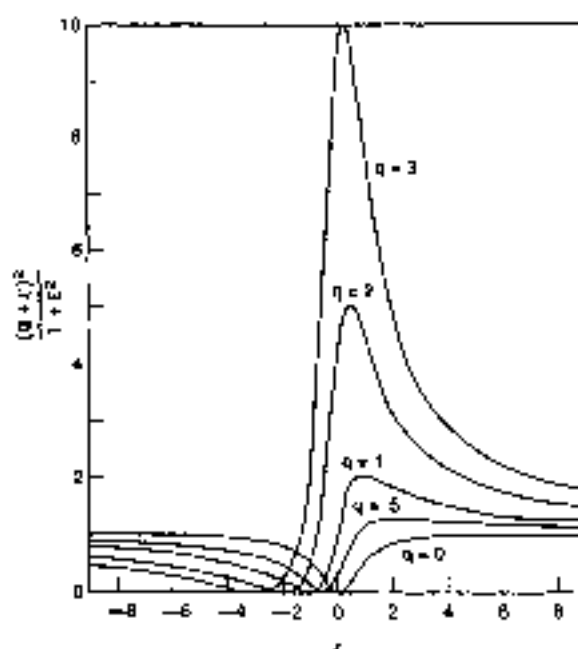
Fig. 14 Natural lineshapes for different values of q (reverse the scale of abscissas for negative q ); asymmetry and antiresonances caused by interference between the discrete state and the background are shown (from U. Fano, Phys. Rev. 124 , 1966 (1961); copyright 1961 by the American Physical Society).
