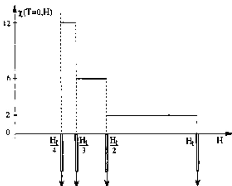
Fig. 9 Magnetic susceptibility (in units of 2\mu_B n_2/H_L ) of the two-dimensional free-electron gas at zero temperature.
