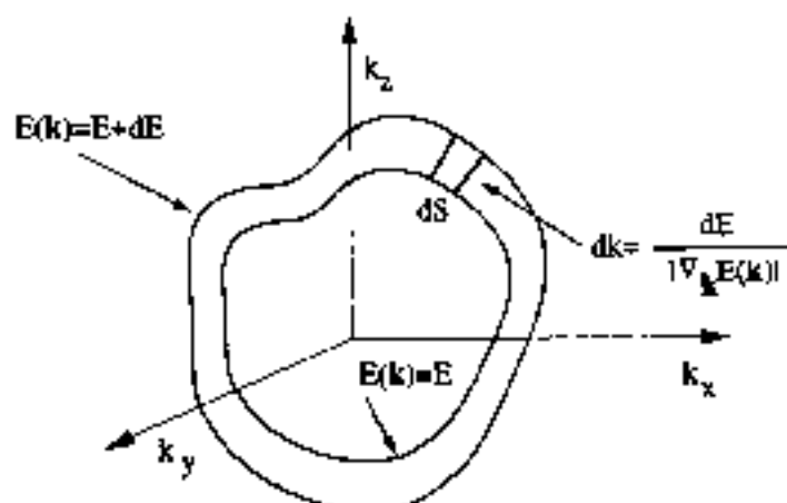
Fig. 21. Schematic representation of two isoennergetic surfaces in the \mathbf{k} space
