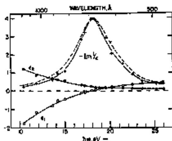
Fig. 9 Dielectric functions \epsilon_1(0, \omega) , \epsilon_2(0, \omega) and -\text{Im} 1/\epsilon(0, \omega) for beryllium, obtained from optical measurements. The dashed curve for -\text{Im} 1/\epsilon(0, \omega) is elaborated from electron-scattering experiments [from J. Toss, H. A. Fowler and L. Marton, Phys. Rev. 172 , 670 (1968), copyright 1966 by the American Physical Society].
