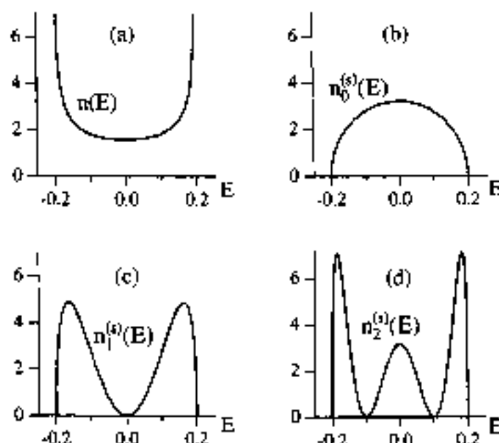
Fig. 11 Local density of states on the bulk orbital of a constant infinite linear chain (a), at the surface orbital of a semi-infinite chain (b), and on the next two orbitals (c) and (d). The chosen value of \gamma is \gamma = -0.1 eV. Energies are in eV, and the density-of-states is in electron/eV.
