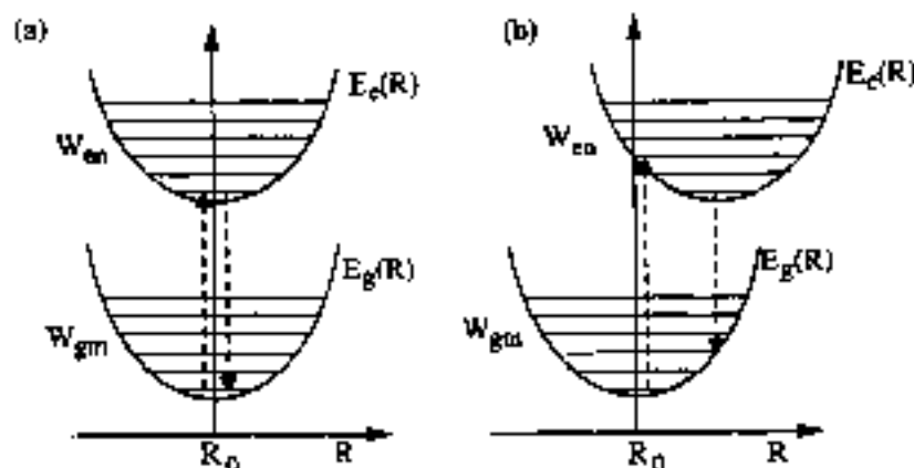
Fig. 2 Schematic behaviour of the adiabatic electronic energies E_g(R) and E_e(R) of the ground-state and lowest excited state of a model dimer system ( R is assumed to be a one-dimensional variable). In case (a) the minima of the adiabatic potential sheets coincide. In case (b) the minima are in different configurations (Franck-Condon model). The quantized vibronic energies are also indicated.
