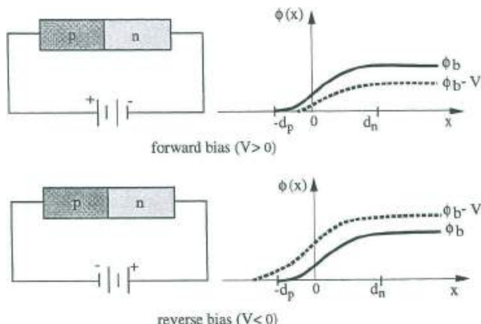
Fig. 3 Forward and reverse bias for a pn junction.
