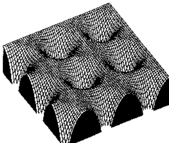
Fig. 10 Schematic representation of the muffin-tin potential.
