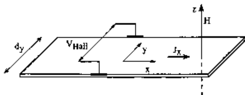
Fig. 12 Standard geometry for Hall effect and magnetoresistivity measurements. V_{\text{Hall}} is the Hall potential, and J_x is the current density in the flow direction.
