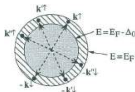
Fig. 8 Schematic representation of the origin of the condensation energy in the BCS ground state. The electron pairs ( k \uparrow , -k \downarrow ) in the blurred region of k space, within an energy shell \Delta_0 around the Fermi level, contribute to the condensation energy of the superconductor (notice that, typically, \Delta_0 \approx 1 \text{ meV} and E_F \approx 1 \text{ eV} ). The dashed lines are a reminder of the binding energy of a Cooper pair.
