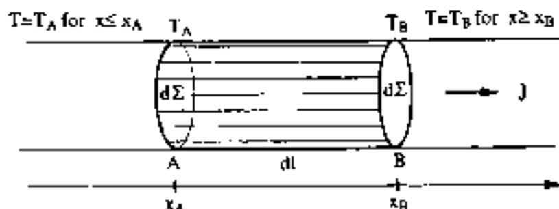
Fig. 13 Schematic figure for the calculation of the Thomson coefficient.
