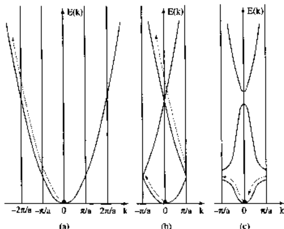
Fig. 14. Schematic representation in k space of the motion of an electron under the influence of a constant electric field F in x direction. In the free-electron case (Fig. 14a), the momentum, velocity and energy increase indefinitely in time. Fig. 14b is the same as Fig. 14a, with the free-electron parabola folded in the first Brillouin zone for convenience. In the presence of the electric field and of a periodic potential, the electron velocity oscillates and the electron undertakes a very fast oscillating motion (Fig. 14c).
