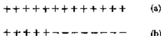
Fig. 7 (a) Schematic representation of a linear Ising chain with all spins parallel to each other. (b) Suppression of long-range order in a linear chain, by a single break.
