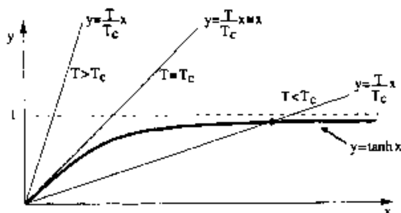
Fig. 1 Graphical solution of the mean field equation (T/T_c)x = \tanh x , for the spontaneous magnetization of a ferromagnetic crystal.
