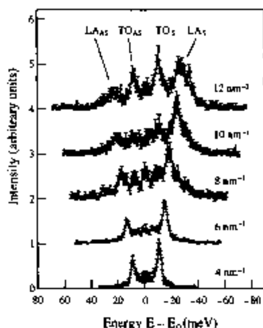
Fig. 7 Inelastic X-ray scattering spectra of polycrystalline \text{H}_2\text{O} ice at -20^\circ\text{C} . The reference energy E_0 is that of the incident beam; the intensity of the scattered beam versus E is reported at the indicated values of the wavevector transfer. The labels TO, LA, S and AS stand for transverse optical, longitudinal acoustic, Stokes and anti-Stokes, respectively [from G. Ruocco, F. Sette, U. Bergmann, M. Krisch, C. Mascareccchio, V. Mazzacurati, G. Signorelli and R. Verbeni, Nature 379, 521 (1995); reprinted with permission from Nature, copyright 1996 Macmillan Magazines Limited]
