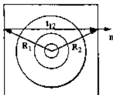
Fig. 9 Schematic visualization of the Wigner-Seitz cell, of the spherically symmetric cellular potential, and of a pair of surface conjugate points R_1 and R_2 for imposing boundary conditions.
