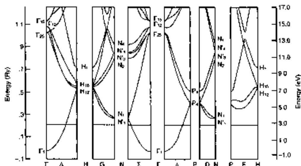
Fig. 11 Band structure of sodium. The Fermi energy is indicated by a dotted line (from D. A. Papaconstantopoulos "Handbook of the Band Structure of Elemental Solids" (Plenum, New York 1986)).
