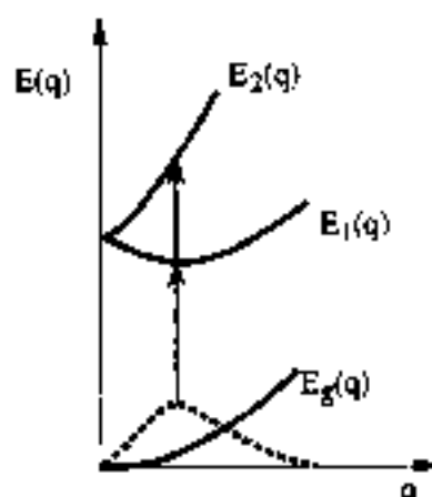
Fig. 21 Adiabatic surfaces E_1(q) and E_2(q) of the vibronic H \otimes c system as a function of the radial coordinate q = (q_1^2 + q_2^2)^{1/2} ; the non-degenerate ground adiabatic surface E_g(q) , from which transition begins, is also indicated. The radial density distribution for a two-dimensional oscillator is shown by a dotted line. The origin of the two principal maxima in the semiclassical band shape is indicated by two solid arrows.
