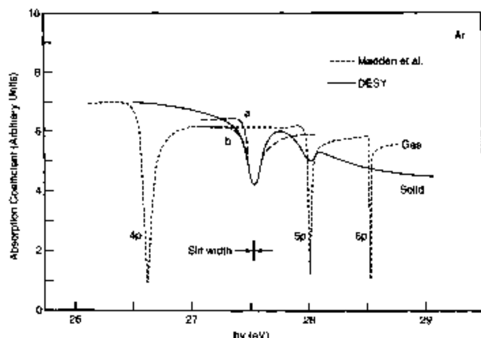
Fig. 16 Absorption spectrum of solid Ar (solid curve) and gaseous Ar (dashed curve). The theoretical curves a and b are fitted on the absorption cross-section of Fano, with two different sets of parameters (see Table 1) [from R. Haensel, G. Keitel, C. Kutz and P. Schreiber, Phys. Rev. Lett. 25 , 208 (1970) (copyright 1970 by the American Physical Society); the absorption spectrum of gaseous Ar is given by R. P. Madden, D. L. Edger and K. Codling, Phys. Rev. 177 , 136 (1969)].
