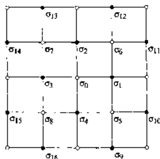
Fig. 11 Two-dimensional square Ising lattice with nearest neighbour spin interactions: labels of sites are introduced for the application of the renormalization procedure.
