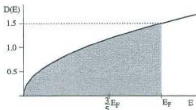
Fig. 3 Density-of-states, in units of N/E_F , for a free-electron gas (the conduction band region occupied by electrons has been shadowed). the average electron energy (3/5)E_F is also indicated
