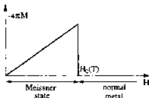
Fig. 4 Magnetization versus applied field for type-I superconductors
