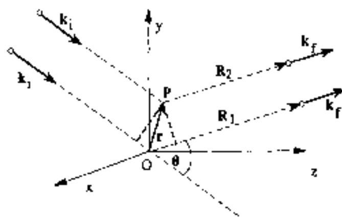
Fig. 3 Schematic geometry of an electromagnetic field scattered from one electron at the origin O and another electron at the point P ; the difference in optical length between the wave scattered from O and the wave scattered from P is k_f \cdot r - k_i \cdot r = \Delta k \cdot r .
