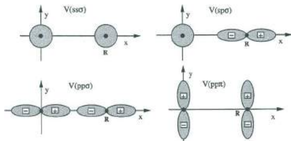
Fig. 1 Pictorial representation of the independent two-center integrals concerning s and p atomic wavefunctions. One center is taken at the origin and the other center R is taken in the x -direction.
