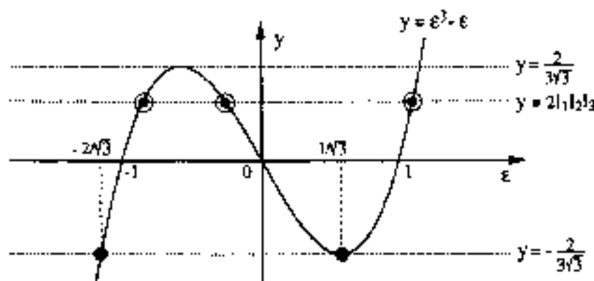
Fig. 9 Graphical solution of the equation \varepsilon^3 - \varepsilon = 2l_1l_2l_3 ; the roots are obtained from the intersection of the cubic curve y = \varepsilon^3 - \varepsilon with the straight line y = 2l_1l_2l_3 . In particular at the point P = (1/\sqrt{3})(-1, -1, -1) we have l_1l_2l_3 = -1/(3\sqrt{3}) ; the equation \varepsilon^3 - \varepsilon = -2/(3\sqrt{3}) has the single root \varepsilon_1 = -2/\sqrt{3} and the doubly degenerate roots \varepsilon_2 = \varepsilon_3 = 1/\sqrt{3} .
