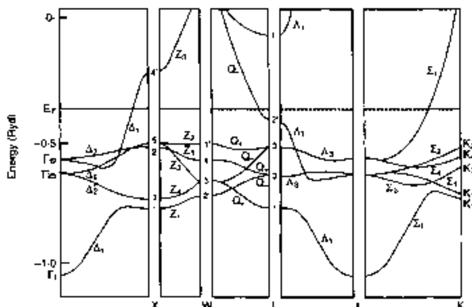
Fig. 13 Band structure of copper [from G. A. Burdick, Phys. Rev. 129, 138 (1963); copyright 1963 by the American Physical Society]
