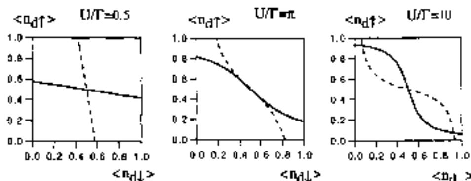
Fig. 3 Graphical solution of the self-consistent equations (31) for different values of the dimensionless ratio U/T .
