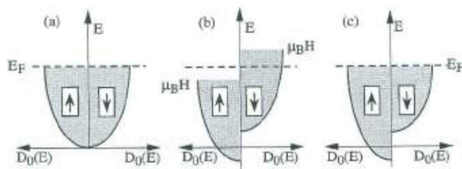
Fig. 11 Schematic representation of the origin of the Pauli spin paramagnetism of a free-electron gas; arrows indicate the direction up or down of the electron spin magnetic moment; D_0(E) denotes the density-of-states for one spin direction.
