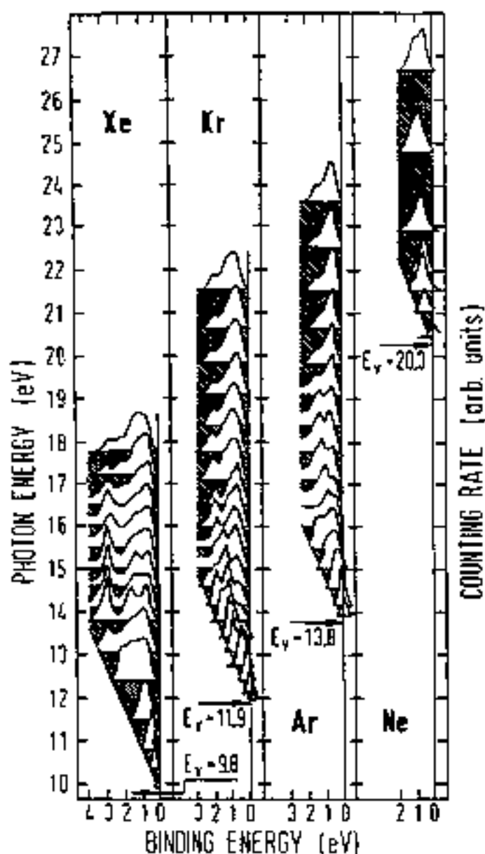
Fig. 2 Energy distribution curves of emitted photoelectrons for solid Ne, Ar, Kr, and Xe, at various photon energies. The zero-count line for each individual curve is shifted upwards (proportions) to the exciting photon energy. E_\gamma represents the vacuum energy measured from the top of the valence band [from N. Schwentner, F.-J. Himpsel, V. Saile, M. Skibowski, W. Steinmann and E. E. Koch, Phys. Rev. Lett. 34 , 528 (1975); copyright 1975 by the American Physical Society].
