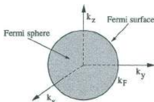
Fig. 2 Schematic representation in the k -space of the Fermi sphere of occupied states and of the Fermi surface of the free-electron gas. At T = 0 each state of wavevector k , with k < k_F , is occupied by two electrons of either spin.
