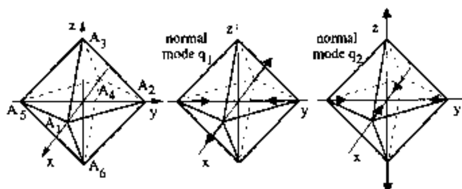
Fig. 6 Geometry of the octahedral complex and degenerate vibrational modes q_1 and q_2 , partner of the \epsilon representation.
