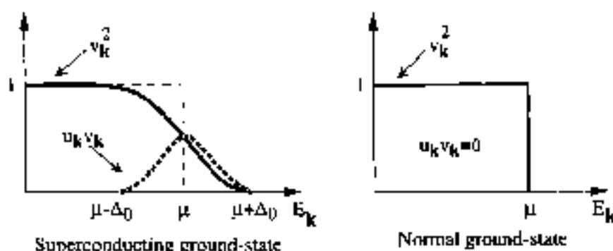
Fig. 9 Behaviour of the quantities v_k^2 and u_k v_k for the superconducting ground state and for the normal ground state
