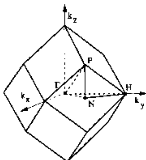
Fig. 19 Brillouin zone for the body-centered cubic lattice (rhombic dodecahedron). Some high symmetry points are also indicated: \Gamma = 0 ; N = (2\pi/a)(1/2, 1/2, 0) ; P = (2\pi/a)(1/2, 1/2, 1/2) ; H = (2\pi/a)(0, 1, 0) .
