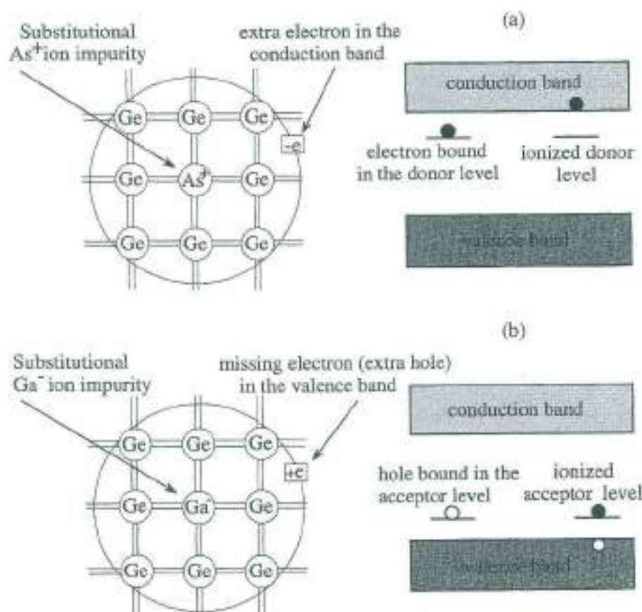
Fig. 4 (a) Schematic picture of a substitutional donor impurity (i.e. arsenic) in germanium: the pentavalent impurity is embodied in the lattice as positive \text{As}^+ ion, with its four external electrons forming four covalent bonds with the nearest neighbour Ge atoms: each \text{As}^+ ion introduces a shallow donor level, below the bottom of the conduction band: the fifth electron, not incorporated in the bonding, is bound to the \text{As}^+ ion by the Coulomb attraction (at low temperature) and is donated to the conduction band (at sufficiently high temperature). (b) Schematic picture of a substitutional acceptor impurity (i.e. gallium) in germanium: the trivalent impurity is embodied in the lattice as negative \text{Ga}^- ion, with its four external electrons forming four covalent bonds with the nearest neighbour Ge atoms: each \text{Ga}^- impurity introduces a shallow acceptor level, above the top of the valence band. The "missing electron" or "hole", created for the formation of the tetrahedral bonding, is bound to the \text{Ga}^- ion by Coulomb attraction (at low temperature) and is given to the valence band (at sufficiently high temperature).
