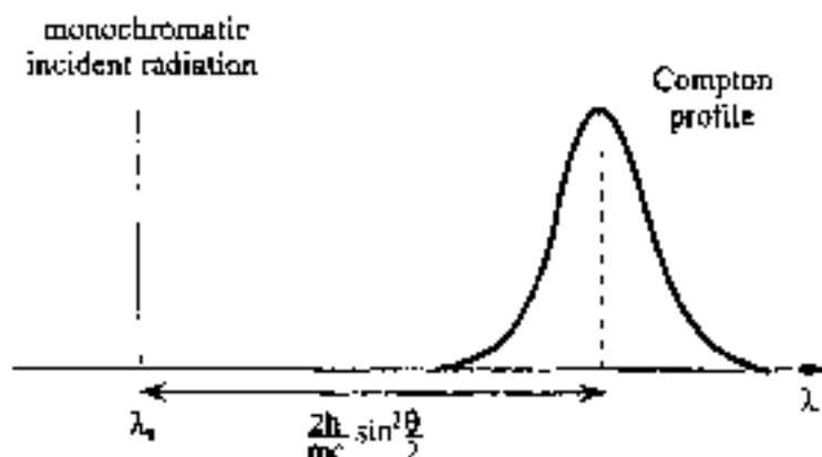
Fig. 11 Schematic representation of the profile of the Compton-scattered radiation. The incident radiation is supposed to be monochromatic, with wavelength \lambda_i ; the scattered radiation is shifted by (2h/mc)\sin^2(\theta/2) and also Doppler-broadened.
