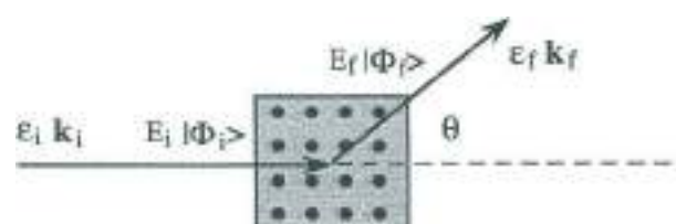
Fig. 14 Diffusion of particles from a crystal and effect of the thermal motion of the atoms: E_i, |\Phi_i\rangle , E_f and |\Phi_f\rangle denote energies and vibrational states of the whole crystal lattice before and after the scattering; \epsilon_i , k_i , \epsilon_f and k_f are the energies and the wavevectors of the probe particle before and after the scattering.
