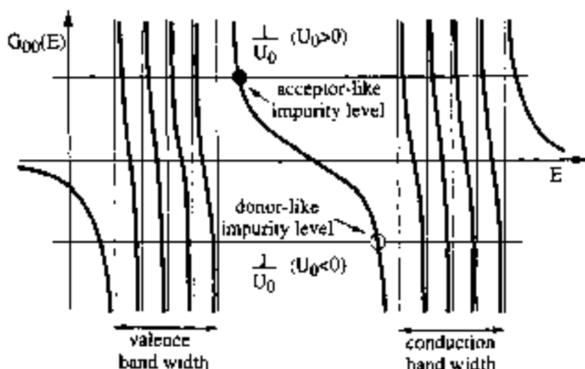
Fig. 6 Schematic graphical solution of the compatibility equation G_{00}(E) = 1/U_0 for impurity levels in semiconductors. The vertical lines correspond to (arbitrarily discretized) energies within the allowed energy bands. The intersection of the Green's function y \equiv G_{00}(E) with the horizontal line y = 1/U_0 yields the energies of the impurity states (we focus here on the states within the energy gap). Small attractive values of U_0 produce a donor-like impurity level, split off from the conduction band; small repulsive values of U_0 produce an acceptor-like impurity level, split off from the valence band. Impurity states, deep in the forbidden energy gap, are controlled jointly by the conduction and valence band states.
