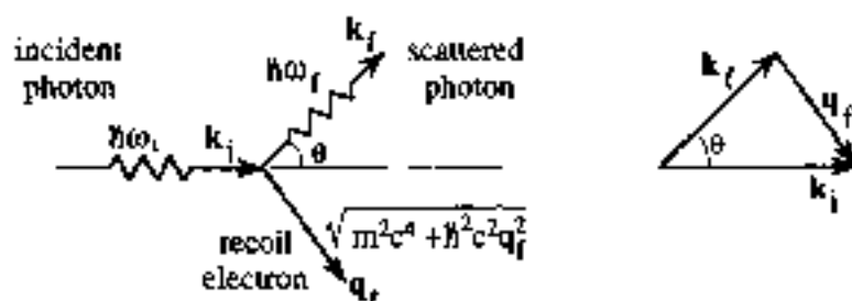
Fig. 10 Schematic representation of the Compton scattering, through an angle \theta , of a photon impinging on an electron initially at rest
