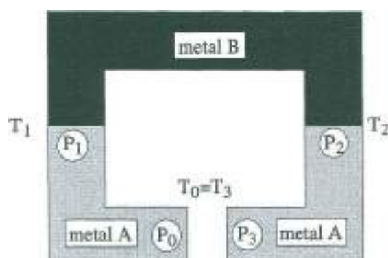
Fig. 12 Standard bimetallic circuit to measure the thermoelectric effect. The two junctions between the metals are kept at different temperatures ( T_1 \neq T_2 ); a voltage appears between points P_0 and P_3 .
