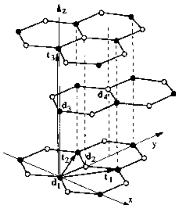
Fig. 11 Three-dimensional crystal structure of graphite. The primitive translation vectors t_1, t_2, t_3 and the end-points of the basis vectors d_1, d_2, d_3 and d_4 , given in Eqs. (14) of the text, are also indicated
