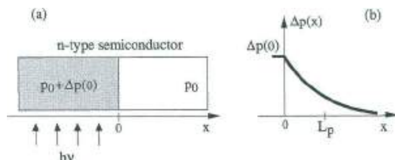
Fig. 10 (a) Schematic representation of an n -type sample subject to irradiation. (b) Distribution of excess holes (and excess electrons) for x > 0 .
