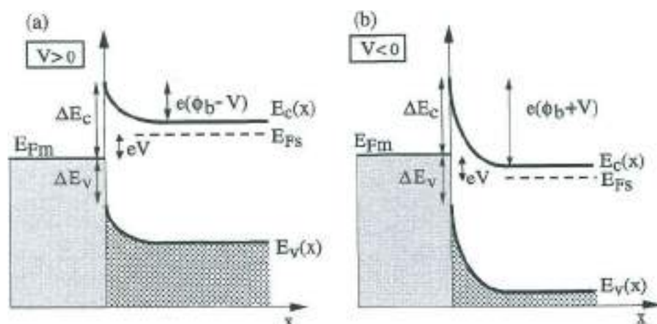
Fig. 14 Schematic energy band profile of a junction between a metal and an n-type semiconductor under forward bias (a) and reverse bias (b).
