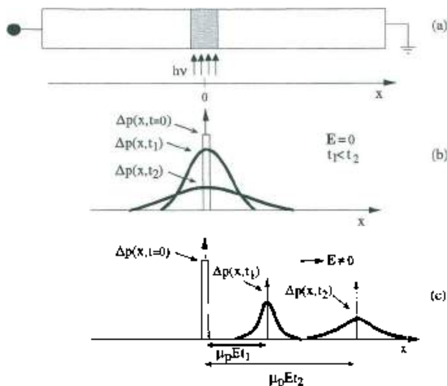
Fig. 12 (a) Schematic representation of an n-type semiconductor with a narrow pulse of holes (and electrons) optically injected at x=0 and t=0 . (b) Distribution of excess holes (and electrons) in the absence of applied electric fields. (c) Distribution of excess holes (and electrons) in the presence of a constant and uniform electric field.
