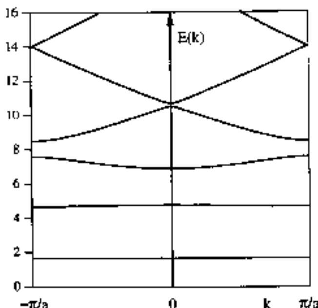
Fig. 13 Energy bands for the periodic Mathieu potential V(x) = 2V_1[1 - \cos(2\pi x/a)] with V_1 = 5(\hbar^2/2m)(\pi/a)^2 . Energies are in Rydberg and a = 5a_Z .
