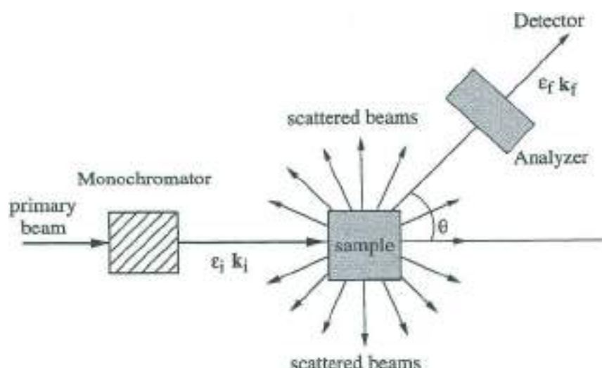
Fig. 1 Schematic experimental set-up for scattering measurements.
