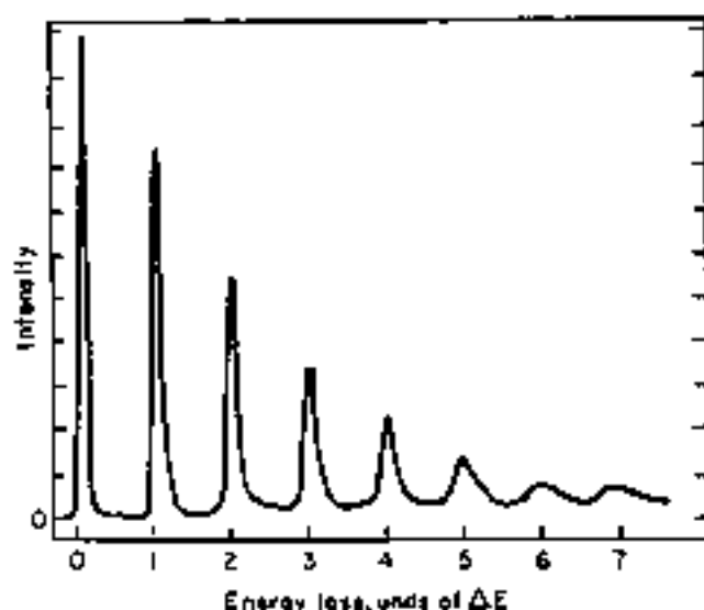
Fig. 4 Energy-loss spectrum (at very small angles) for a beam of 20 keV primary electrons passing through an aluminum film of thickness \approx 2560 \text{ \AA} . The unit of energy-loss \Delta E ( \approx 15 \text{ eV} ) is the plasmon excitation energy for Al. Zero-loss, first-loss, second-loss and other plural-loss peaks are clearly detected [from L. Marston, J. A. Simpson, H. A. Fowler and N. Swanson, Phys. Rev. 126 , 132 (1962); copyright 1962 by the American Physical Society]
