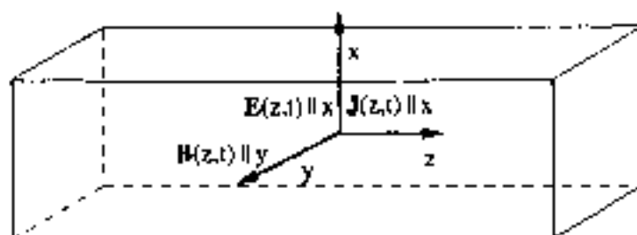
Fig. 1 Geometry chosen for the description of transverse electromagnetic fields in isotropic materials. The electric field and the internal density current are in the x -direction, the magnetic field is in the y -direction, the wave propagation is along the z -direction.
