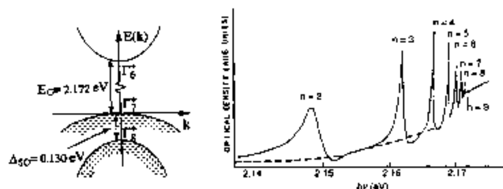
Fig. 11 (a) Schematic band structure of \text{Cu}_2\text{O} showing the conduction band \Gamma_6^+ , and the valence bands \Gamma_7^+ and \Gamma_8^+ , split by spin-orbit interaction. (b) Absorption spectrum of the yellow exciton series in \text{Cu}_2\text{O} at 1.8 K [from K. Shindo, T. Goto and T. Anzai, J. Phys. Soc. Japan 38, 753 (1974)]. Since the band-to-band transition is dipole forbidden at the symmetry point \mathbf{k} = 0 , the exciton series begins with the line n = 2 .
