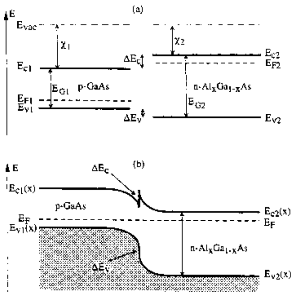
Fig. 11 (a) Energy bands and Fermi levels in two separated semiconductors: p-type GaAs and n-type Al x Ga 1-x As. (b) Energy band profile and Fermi level across the heterostructure at thermal equilibrium.
