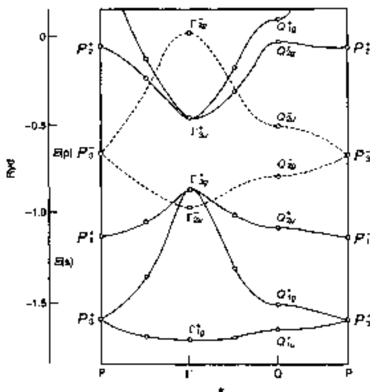
Fig. 4 Band structure of two-dimensional graphite, obtained with the tight-binding method. Bands which are even and odd under reflection in the plane of graphite are indicated with continuous and broken lines respectively. The energies of the valence states of the carbon atom are also indicated. The values of k at the points \Gamma , P and Q , are k = 0 , k = (2\pi/a)(2/3, 0, 0) and k = (2\pi/a)(1/2, 1/2\sqrt{3}, 0) , respectively (from P. Dascari and G. Pastori-Patravici, Nuovo Cimento 50B, 95 (1967), copyright 1967 by Società Italiana di Fisica).
