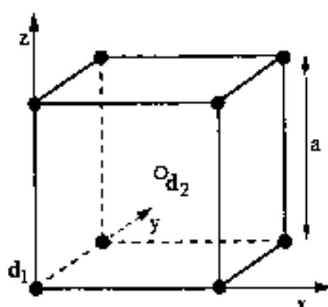
Fig. 7 The cesium chloride structure, the end-points of the basis vectors d_1 and d_2 , given in Eqs. (10) of the text, are also indicated.
