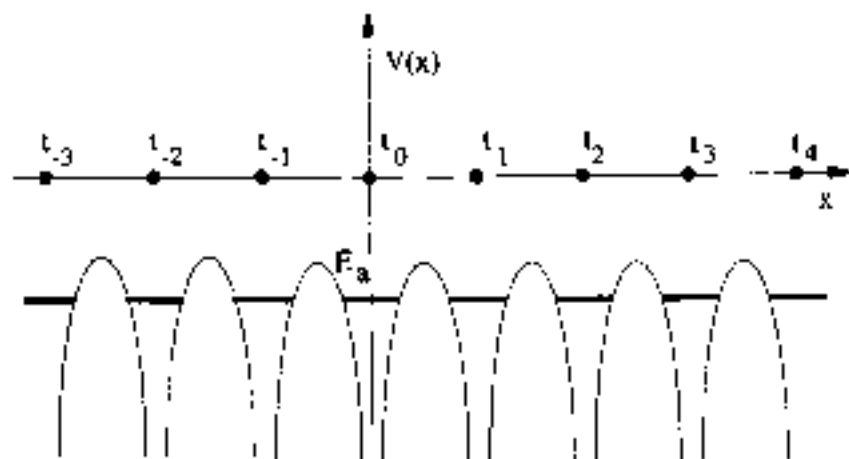
Fig. 8 Schematic representation of the crystal potential as a superposition of atomic-like potentials, centered at the lattice sites l_n . In the tight-binding approximation, the interaction between nearby atomic-like orbitals \phi_a of energy E_a leads to the formation of energy bands.
