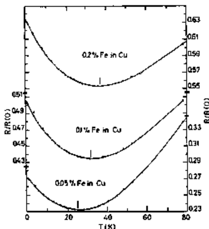
Fig. 5 Resistance at low temperatures for Cu with 0.05%, 0.1% and 0.2% of Fe impurities [from J. P. Frauch, F. D. Manchester and D. L. Martin, Proc. Roy. Soc. (London) A263 , 494 (1961)].
