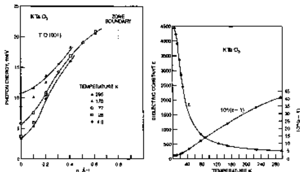
Fig. 15 (a) Temperature dependence of the soft transverse optical branch in \text{KTaO}_3 [from G. Shirane, R. Narhans and V. J. Minkiewicz, Phys. Rev. 157 , 396 (1967); copyright 1967 by the American Physical Society] (b) Dielectric constant and reciprocal susceptibility of \text{KTaO}_3 as a function of temperature [from S. H. Wemple, Phys. Rev. 137 , A1575 (1965), copyright 1965 by the American Physical Society].
