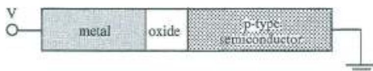
Fig. 16 Schematic representation of a biased metal-oxide-semiconductor junction, no current flows in the structure, and carriers are at thermal equilibrium both in the metal and in the semiconductor.
