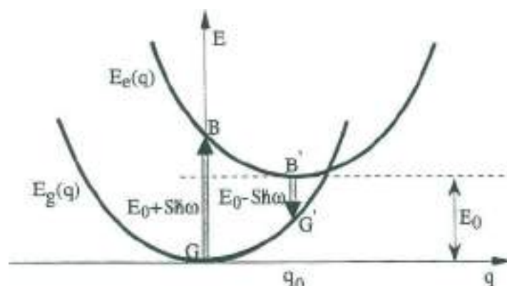
Fig. 17 Configuration-coordinate diagram for allowed transitions between two non-degenerate electronic states (Franck-Condon model). The adiabatic potential surfaces for the ground state and the lowest excited state are indicated as a function of a single normal coordinate q .
