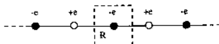
Fig. 4 Schematic representation of a one-dimensional ionic crystal in the point ion approximation, for the calculation of the Madelung constant. The nearest neighbour distance is denoted by R . The ion at the origin has been surrounded by a box.
