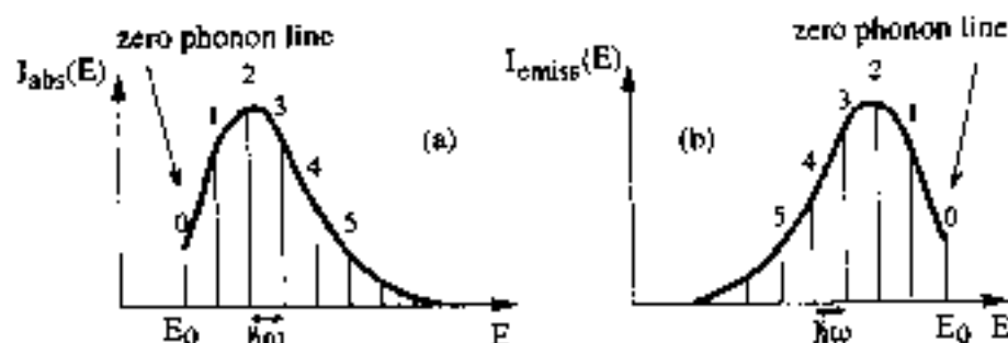
Fig. 18 (a) Polarisade spectrum of optical absorption for the two-level single-mode model (the system is initially in the ground electronic state and ground vibrational state); the zero-phonon line is indicated by an arrow. (b) Polarisade spectrum of optical emission for the two-level single-mode model (the system is initially in the excited electronic state and ground vibrational state); the zero-phonon line is indicated by an arrow. In the figures we have chosen S = 2.5 .
