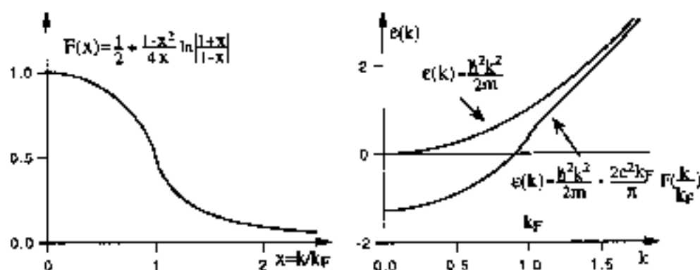
Fig. 4 (a) Schematic plot of the function F(x) . (b) Kinetic energy and Hartree-Fock orbital energy as a function of the wavevector k for the homogeneous electron gas. Energies are in Rydbergs, k is in units of a_0^{-1} (inverse Bohr radius), and we have taken k_F = 1/a_0 .
