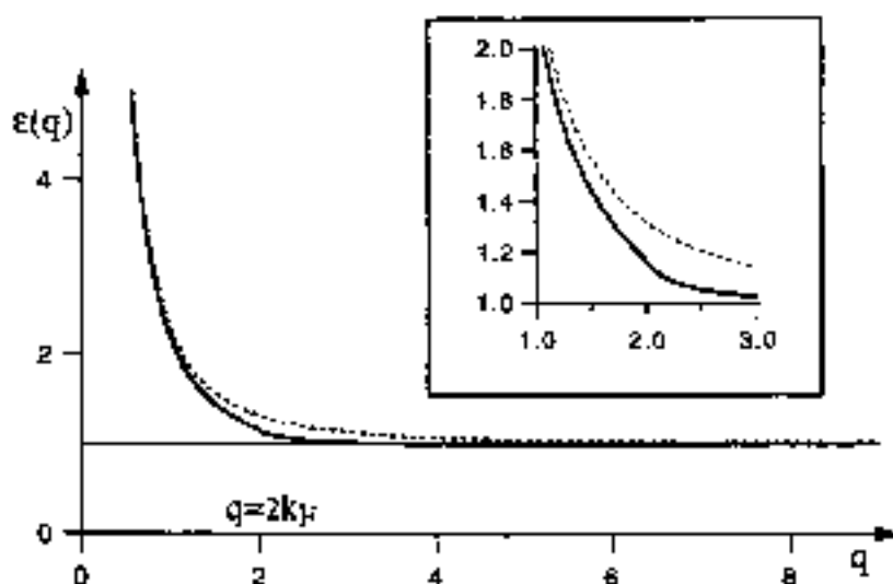
Fig. 6 Behaviour of the static Lindhard (solid line) and Thomas-Fermi (dashed line) dielectric function of a free-electron gas. The inset shows the behaviour of \epsilon(q) near q=2k_F (we have chosen k_F = 1/a_B^{-1} or equivalently r_s = 1/92 ; q is in units of a_B^{-1} ).
