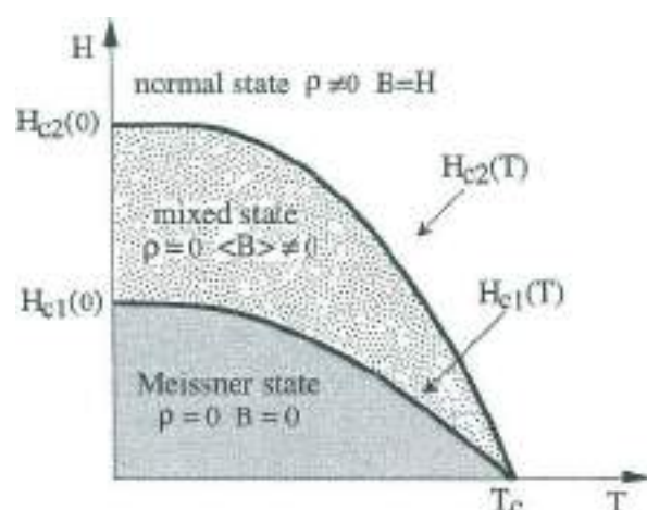
Fig. 5 Schematic phase diagram illustrating normal, mixed and Meissner regions of a type-II superconductor (the zero resistivity of the mixed state occurs if flux lines are "pinned" by appropriate material defects); in the mixed state, \langle B \rangle denotes the average magnetic field in the superconductor
