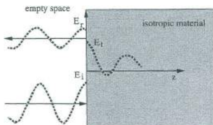
Fig. 2 Schematic representation of incident, reflected and transmitted electromagnetic waves at the surface (the z = 0 plane) of an isotropic material. the normal incident situation is considered.
