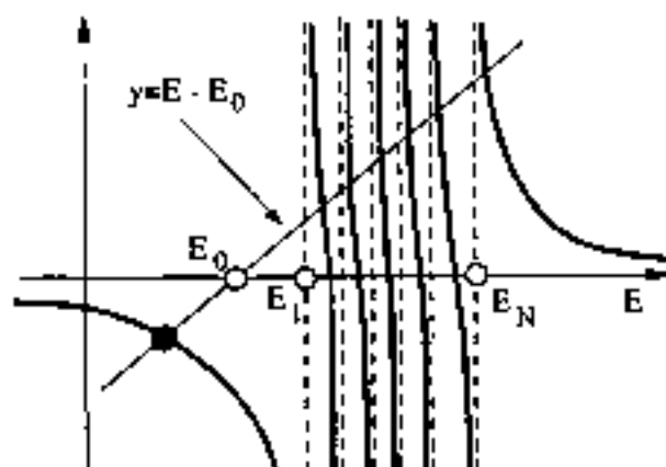
Fig. 17 Graphical solution of the eigenvalues of the Hamiltonian describing a discrete state E_0 interacting with a quasi-continuum of states extending from E_{\min} = E_1 to E_{\max} = E_N . We illustrate the case E_0 < E_{\min} . Notice that a "collective state" always appears with energy smaller than E_0 .
