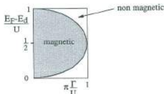
Fig. 4 Phase diagram corresponding to the Hartree-Fock solution of the Anderson Hamiltonian for a magnetic impurity in a normal metal [from P. W. Anderson, Phys. Rev. B124, 41 (1961)].
