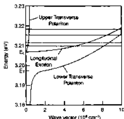
Fig. 12 Dispersion curves of the transverse exciton-polaritons of CuCl in the anomalous dispersive region. The dashed lines refer to the inner energies used to study luminescence line shape due the decay from bound pairs of excitons [from J. K. Pribbraun, G. L. Koss, P. Bassani and J. P. Wolfe, Phys. Rev. B 28 , 1046 (1983), copyright 1983 by the American Physical Society]
