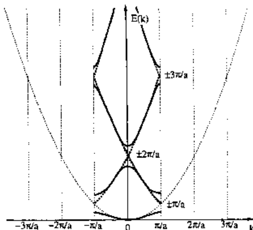
Fig. 12 Empty lattice states (free-electron parabolae) and folding in the first Brillouin zone. At the center and at the border of the first Brillouin zone we have also indicated the wavenumbers of the degenerate plane waves. In the presence of a periodic potential, gaps open at the center and at the border of the Brillouin zone, as shown qualitatively by continuous lines.
