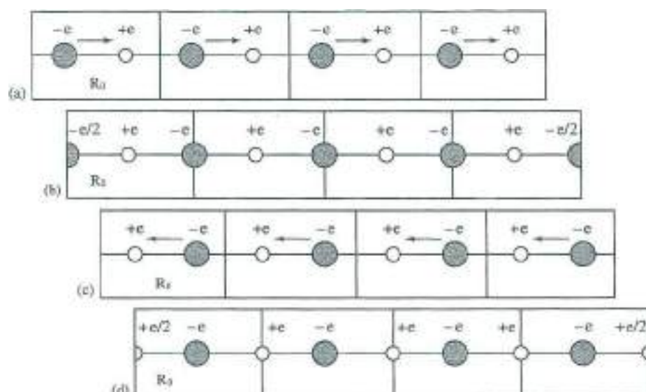
Fig. 11 Schematic illustration of the electric polarization of a one-dimensional crystal composed by a number of unit cells of volume \Omega . The crystal is constituted by uniformly charged spheres of charge +e and -e (white and black circles) at distance R_0 . Four different ways to choose the unit cell and to assemble the crystal are indicated; arrows indicate the electric dipole vector in the unit cell. In case (a) the polarization is P = +eR_0/\Omega ; in case (b) and (d) it is zero; in case (c) P = -eR_0/\Omega . If all the negative charges of the crystal are displaced by \delta , while the positive charges are kept fixed, the change of polarization is in any case given by \Delta P = -e\delta/\Omega , regardless of the different ways the crystal has been assembled.
