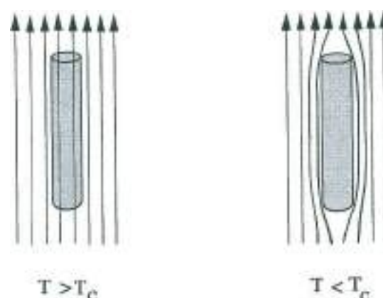
Fig. 2 Exclusion of a weak external magnetic field from the interior of a superconductor.
