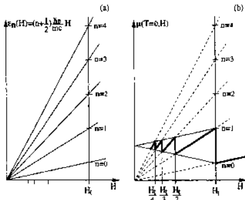
Fig. 6 (a) Plot of Landau levels versus H for several values of the quantum number n . (b) Chemical potential \mu(T=0, H) versus H for a two-dimensional free electron gas at zero temperature, showing discontinuities at H = H_c/i , with i integer number.
