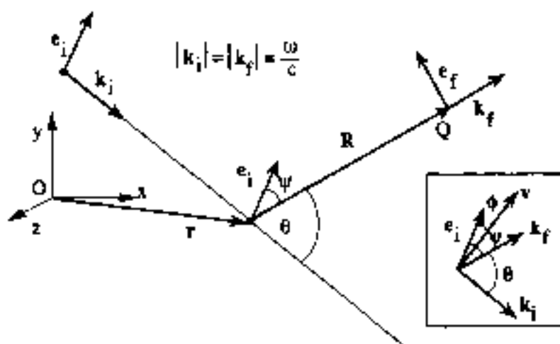
Fig. 2 Schematic representation of an incident electromagnetic wave (of frequency \omega , propagation vector \mathbf{k}_i , polarization vector \mathbf{e}_i ) elastically scattered from a free electron at the point \mathbf{r} and detected at the point \mathbf{Q} \equiv \mathbf{r} + \mathbf{R} . In the inset, the angles of geometrical interest are indicated. The scattering angle is \theta ( \cos \theta = \mathbf{k}_i \cdot \mathbf{k}_f , where \mathbf{k}_i and \mathbf{k}_f denote vectors); \psi denotes the angle between \mathbf{e}_i and \mathbf{R} or \mathbf{k}_f ( \cos \psi = \mathbf{e}_i \cdot \mathbf{k}_f ); \phi = \mathbf{e}_f \sin \psi + \mathbf{k}_f \cos \psi ; \mathbf{v} = (\mathbf{k}_f - \mathbf{k}_i \cos \theta) / \sin \theta is the vector that lies in the (\mathbf{k}_i, \mathbf{k}_f) plane and is perpendicular to \mathbf{k}_i ; \delta is the polarization angle ( \cos \delta = \mathbf{e}_i \cdot \mathbf{v} = \cos \psi / \sin \theta ).
