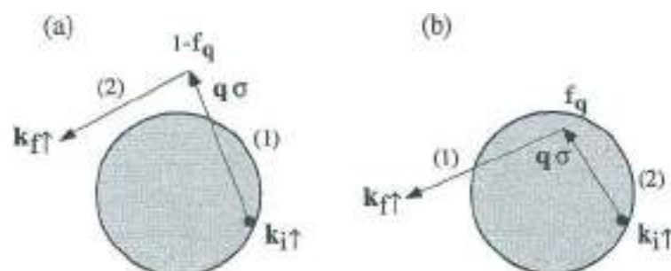
Fig. 6 (a) Direct process in second-order Born approximation for scattering of an electron from the initial state k_i \uparrow to the final state k_f \uparrow via an empty intermediate state q\sigma . (b) Exchange process contributing to second-order scattering amplitude: the filled state q\sigma is first scattered to the final state k_f \uparrow and is then occupied by the electron in the state k_i \uparrow . In Fig. (a) and Fig. (b) the initial states of the Fermi gas can be represented by the same Slater determinant; it is then easily seen that the two final Slater determinants, at the end of the processes of Fig. (a) and Fig. (b), have a pair of electronic functions exchanged; hence the factor (-1) in Eq. (36).
