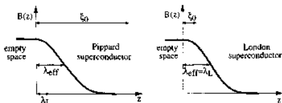
Fig. 18 Qualitative distinction between Pippard and London superconductors; B(z) denotes the magnetic field parallel to the surface, in the geometry indicated in Fig. 16.
