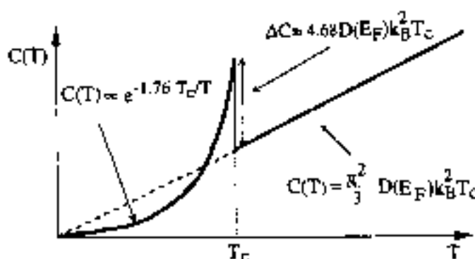
Fig. 15 Characteristic behaviour of the heat capacity of a normal metal and a superconductor, above and below the critical temperature.
