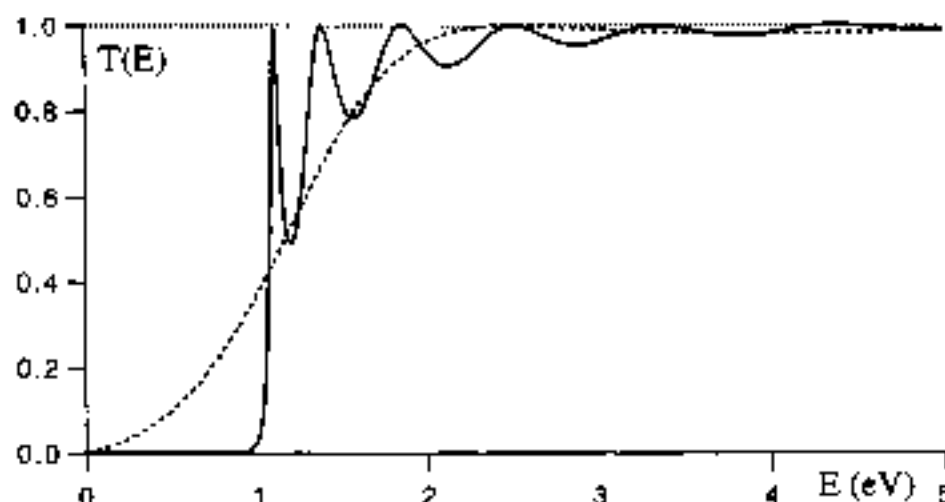
Fig. 6 Transmission coefficient through a barrier of height V_0 = 1 \text{ eV} and length b = 5 \text{ Å} (dashed line), and through a barrier of height V_0 = 1 \text{ eV} and length b = 20 \text{ Å} (solid line).
