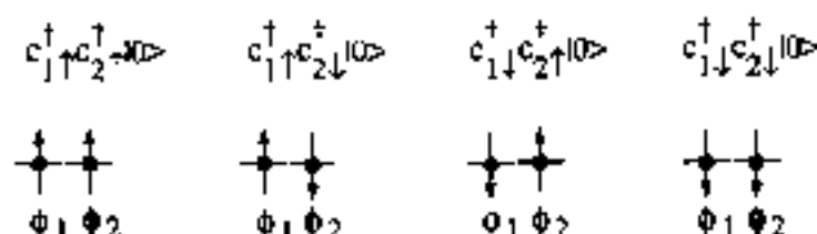
Fig. 3 The four possible two-electron states of a system with two orbitals and two electrons (double occupation of the same orbital is avoided)
