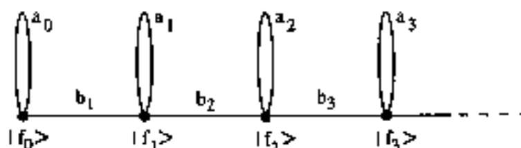
Fig. 14 Schematic representation of the linear chain generated by the Lanczos procedure
