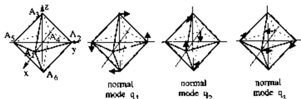
Fig. 8 Geometry of the octahedral complex and normal coordinates q_1, q_2, q_3 of the triply degenerate vibrational mode \tau (even under space inversion symmetry).
