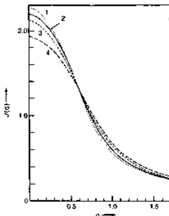
Fig. 12 Compton profile of lithium hydride ( q is in units a_B^{-1} , inverse Bohr radius). (Curves 1 and 2 correspond to the free ion model with overlap and to the cluster model with overlap of Li^+ and H^- wavefunctions; the calculations are taken from G. Grosso, C. Pastor Parravicini and R. Resta, Phys. Stat. Sol. (b) 73 , 371 (1976). Curves 3 and 4 give the experimental results of W. C. Phillips and H. W. Weiss, Phys. Rev. 182 , 923 (1969) and those of J. Felsteiner, R. Fox and S. Kahane, Phys. Rev. B6 , 4689 (1972), respectively.
