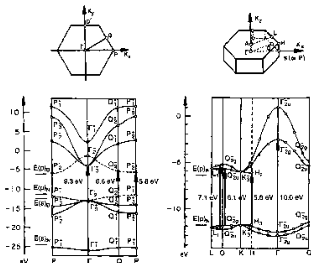
Fig. 5 Two-dimensional (left) and three-dimensional (right) band structures and corresponding Brillouin zones of hexagonal boron nitride. Relevant optical transitions are also indicated [the calculations are due to E. Dogni and G. Pastori Parravicini, Nuovo Cimento 64B, 117 (1969); interpretation of experimental data is due to D. M. Hoffman, G. L. Doll and P. C. Eklund, Phys. Rev. B10, 6061 (1964)]
