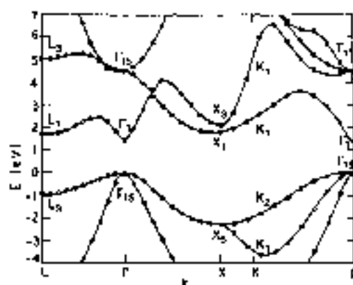
Fig. 7 Energy bands of GaAs by the empirical pseudopotential method (from M. L. Cohen and T. K. Bergstresser, Phys. Rev. 141 , 789 (1966); copyright 1966 by the American Physical Society)
