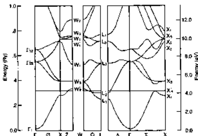
Fig. 12 Band structure of calcium. The Fermi energy is indicated by a dotted line (from D. A. Papaconstantopoulos "Handbook of the Band Structure of Elemental Solids" (Plenum, New York 1986)).
