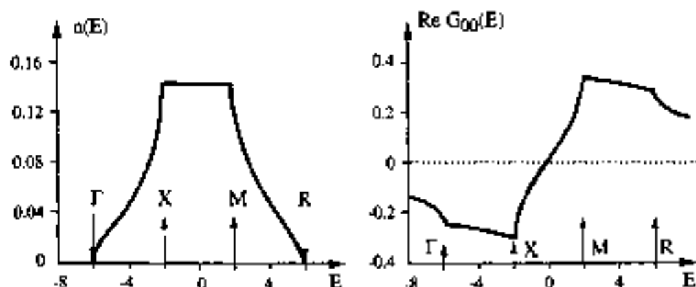
Fig. 25 Density-of-states of the cubium, to illustrate the three-dimensional critical points. The energy E is in units of |\gamma| , and n(E) is normalized to one. Besides n(E) = -(1/\pi)\text{Im } G_{00}(E) , also the real part of the Green's function diagonal matrix element G_{00}(E) , on a localized orbital of the cubium, is reported for convenience [from D. J. Lohrman, L. Hesse, G. Pastori Parravicini and R. D. Graft, Phys. Rev. B 40 , 8464 (1989); copyright 1989 by the American Physical Society].
