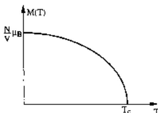
Fig. 2 Spontaneous magnetization as function of temperature.
