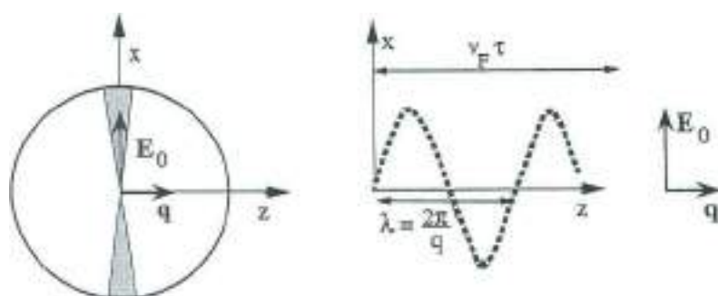
Fig. 9 Illustration of Pippard ineffectiveness concept. Out of all the electrons within the Fermi sphere, only those travelling (almost) parallel to E_0 can absorb energy and contribute to the conductivity, in the extreme anomalous region.
