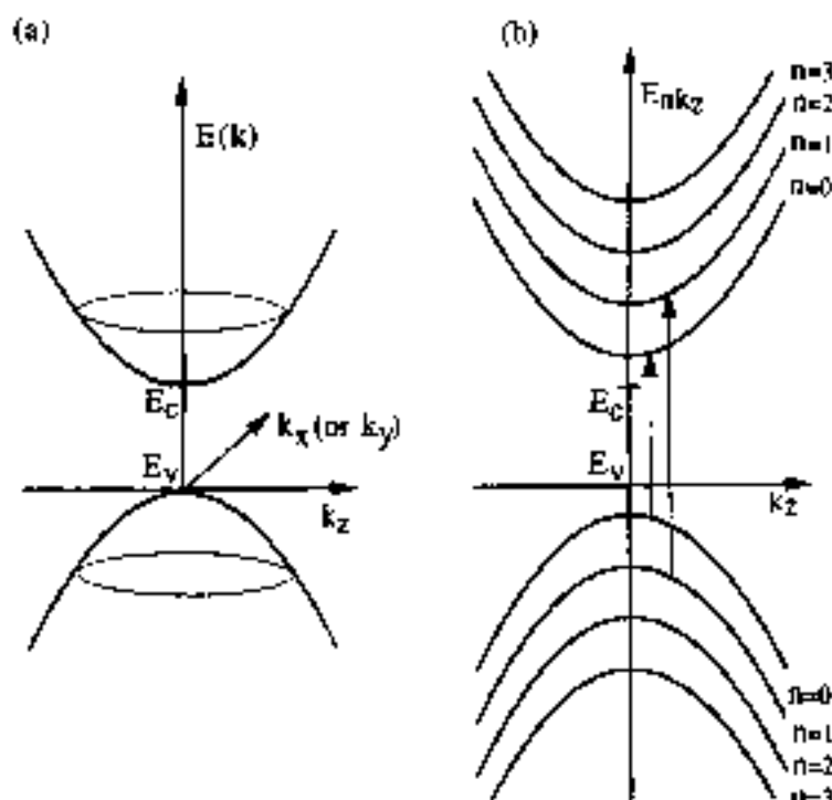
Fig. 4 (a) Schematic representation of an isotropic two-band model semiconductor. (b) Schematic representation of quantization of electron states in the conduction band and in the valence band in the presence of a uniform magnetic field in the z -direction. Arrows indicate examples of optical transitions between valence and conduction states with the same values of n and k_z .
