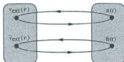
Fig. 7 Schematic representation of the Hohenberg-Kohn theorem. Two different ground-state density functions must correspond to two different potentials, and vice versa.
