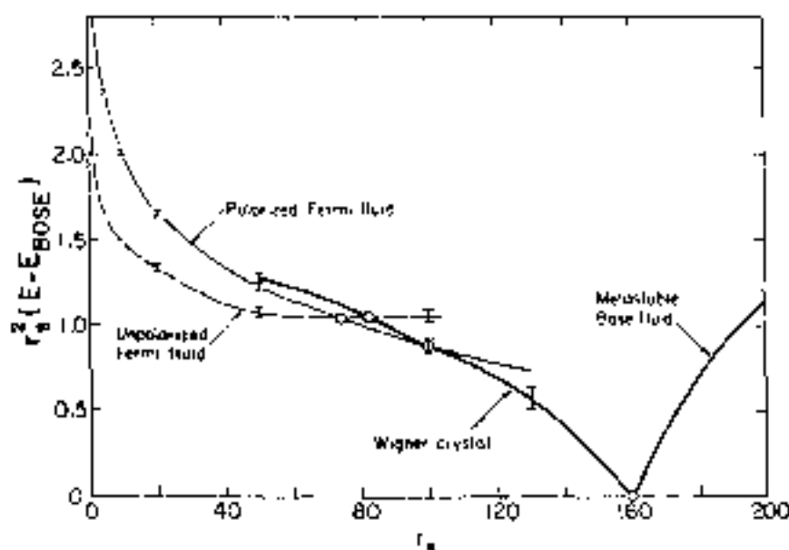
Fig. 6 Energy (times r_s^2 ) in Rydberg versus r_s for several phases of the homogeneous electron gas. The figure shows that the normal Fermi fluid is stable below r_s \approx 75 , the polarized (ferromagnetic) Fermi fluid is stable between r_s \approx 75 and r_s \approx 100 , the Wigner crystal above r_s \approx 100 . In the figure the reference energy E_{\text{BOSE}} is that of the lowest boson phase, i.e. the Bose fluid for r_s < 160 , and the Wigner crystal for r_s > 160 [from D. Ceperley and B. J. Alder, Phys. Rev. Lett. 45, 566 (1980), copyright 1980 by the American Physical Society].
