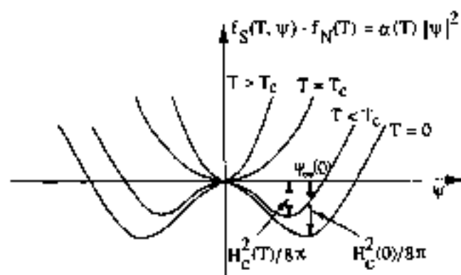
Fig. 19 Schematic behaviour of the Ginzburg-Landau free-energy change (in the absence of fields and gradients) for a typical second-order phase transition.
