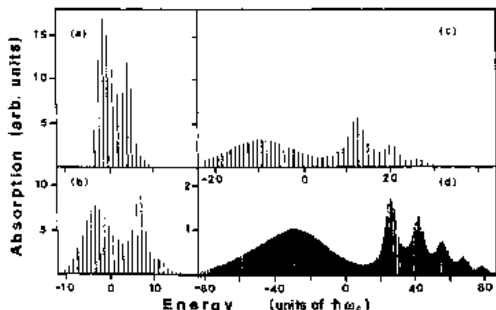
Fig. 22 Absorption spectrum for a transition A \rightarrow E for a vibronic system E \otimes \varepsilon ( A denotes the non-degenerate electronic ground-state and E denotes the doubly-degenerate excited electronic state). The values of the dimensionless Huang-Rhys parameter S are 4, 16, 360, 900 in Figures (a), (b), (c) and (d). [from L. Martinelli, M. Paseno and G. Pastori Parravicini, Phys. Rev. B43, 3395 (1991), copyright 1991 by the American Physical Society].
