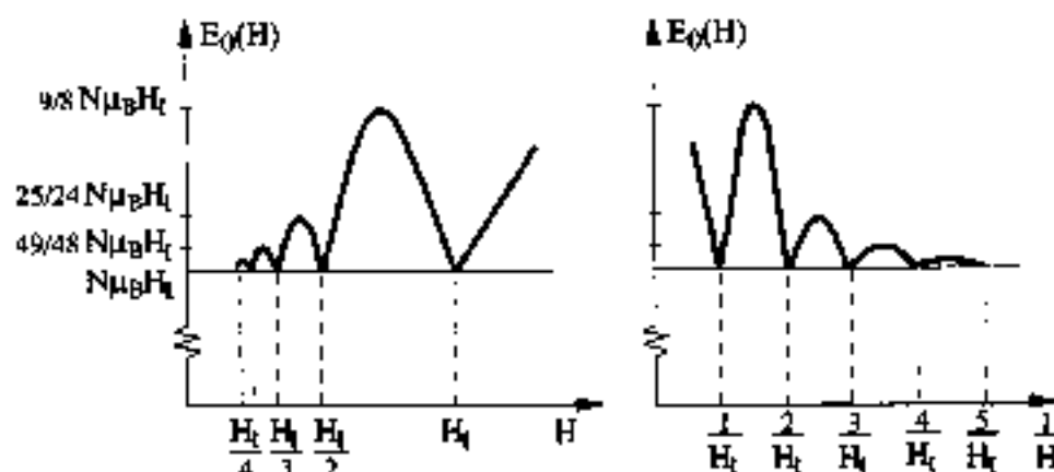
Fig. 7 Ground-state energy of a two-dimensional free-electron gas in a magnetic field as a function of H and 1/H .
