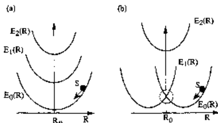
Fig. 1 Schematic representation of adiabatic potential-energy surfaces E_i(R) (the multi-dimensional nuclear variable R is represented as a one-dimensional parameter). In Fig. 1a the adiabatic surfaces are supposed non-degenerate, and the nuclear dynamics of the system S is mostly determined by the single non-degenerate potential surface under consideration. In Fig. 1b two (or more) adiabatic surfaces are degenerate at R_0 , and the nuclear dynamics of the system S is determined by the whole set of degenerate adiabatic surfaces.
