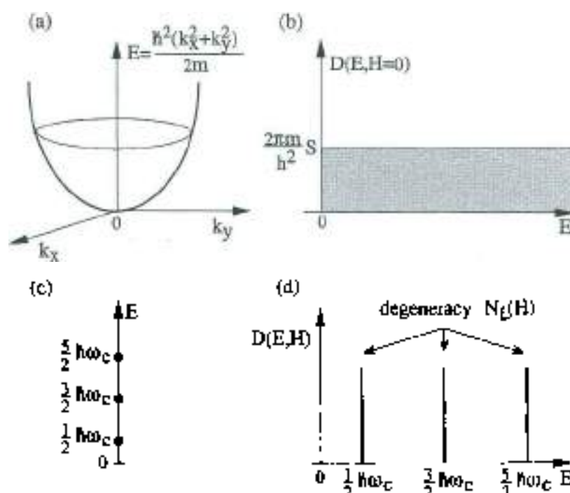
Fig. 1 Energy levels (Fig. 1a) and density-of-states excluding spin degeneracy (Fig. 1b) of a two-dimensional electron gas in the absence of a magnetic field. The energy levels and the density-of-states in the presence of a magnetic field are indicated in Fig. 1c and Fig. 1d, respectively. The degeneracy of the Landau levels is N_L(H) = (e/hc)HS = D(E, H=0)\hbar\omega_c .
