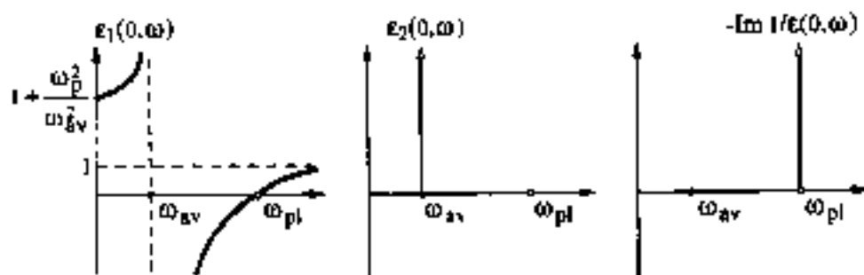
Fig. 11 Schematic behaviour of the Lorentz dielectric function \epsilon(0, \omega) = 1 + \omega_p^2 / (\omega_{gv}^2 - \omega^2 - i\eta) (with \eta \rightarrow 0^+ and \omega > 0 ) and the energy-loss function -\text{Im } 1/\epsilon(0, \omega)
