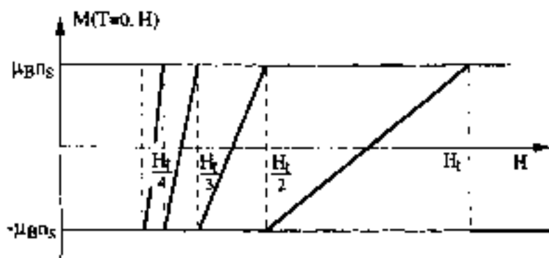
Fig. 8 Magnetic moment per unit surface at T = 0 of a two-dimensional free-electron gas in a magnetic field.
