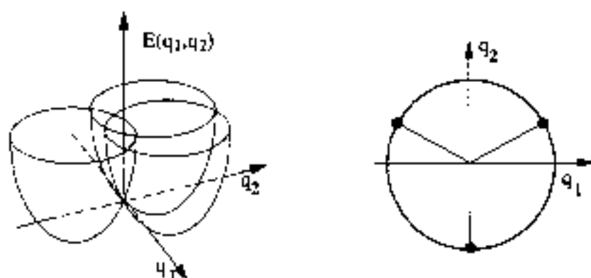
Fig. 7 Schematic representation of the adiabatic-potential energy surfaces in the case of a triply degenerate state T interacting with the e modes ( q_1, q_2 ) in the cubic symmetry environment. The coordinates of the minima of the potential are also shown in a top view.
