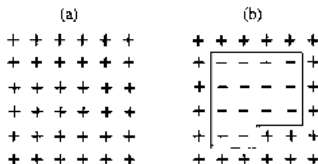
Fig. 8 Break of long range order in a two-dimensional system.
