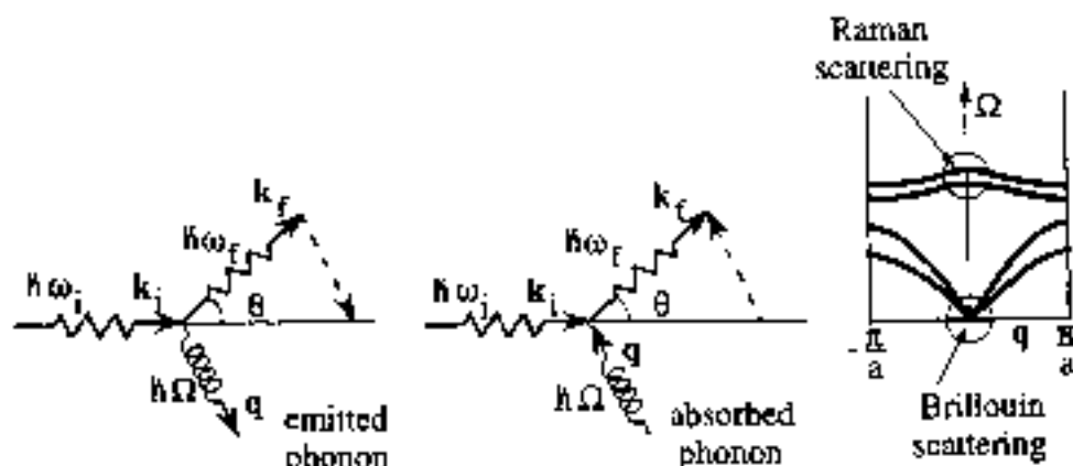
Fig. 8. Scattering of a photon through an angle \theta with creation of a phonon (Stokes process) or annihilation of a phonon (anti-Stokes process); k_i and k_f denote the propagation wavevectors of the photon in the medium, before and after the scattering process. For photons in the visible region, a very small part of the phonon dispersion curves can be explored.
