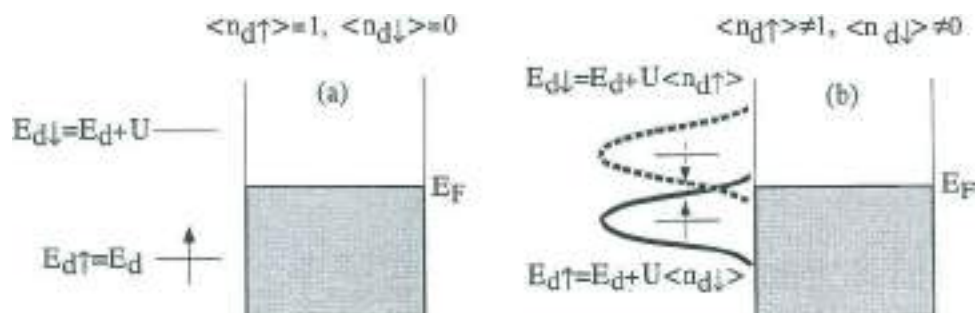
Fig. 2 Schematic representation of the Anderson model. In Fig. (a) the hybridization of the localized level with the Fermi sea is neglected: it is assumed that E_d < E_F and E_d + U > E_F , so that \langle n_{d\uparrow} \rangle = 1 and \langle n_{d\downarrow} \rangle = 0 (or vice versa); then E_{d\uparrow} = E_d + U \langle n_{d\downarrow} \rangle = E_d , while E_{d\downarrow} = E_d + U . In Fig. (b) the hybridization is switched on, and it tends to equalize spin-up and spin-down occupancies and energies.
