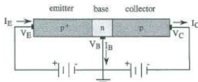
Fig. 6 Schematic representation of a pnp junction transistor in the grounded base arrangement
