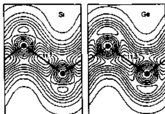
Fig. 10 Calculated pseudovalence charge density in the (110) plane for Si and Ge. The contours are in units of electrons per atomic volume, with a contour step of 1. Atomic positions are denoted by black dots; atomic chains are denoted by straight lines [from M. T. Yin and M. L. Cohen, Phys. Rev. B26, 5668 (1982); copyright 1982 by the American Physical Society].
