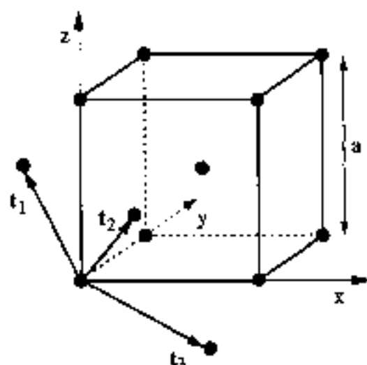
Fig. 5 Body-centered cubic lattice and primitive translation vectors t_1, t_2, t_3 given by Eqs. (8) in the text.
