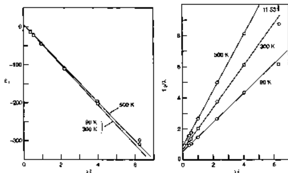
Fig. 5 Dielectric function of copper in the infrared and red region at different temperatures. (a) \epsilon_1 versus square of wavelength (with \lambda in micron); (b) \epsilon_2/\lambda versus square of wavelength (with \lambda in micron) [from S. Roberts, Phys. Rev. 118 , 1509 (1960); copyright 1960 by the American Physical Society].
