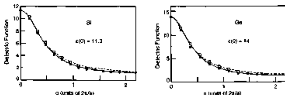
Fig. 13 Static longitudinal dielectric function \epsilon_L(q, 0) for silicon and germanium. Closed boxes [ q along the (1,1,1) direction] and open boxes [ q along the (1,0,0) direction] are from numerical calculations of J. P. Walter and M. L. Cohen, Phys. Rev. B 2 , 1331 (1970). The solid line is the model dielectric function of G. Cappellari, R. Del Sole, L. Rehnig and F. Bechstedt, Phys. Rev. B 47 , 9892 (1993) (copyright 1993 by the American Physical Society). The dashed curve represents the model of Z. H. Levine and S. G. Lowe, Phys. Rev. B 25 , 6310 (1982).
