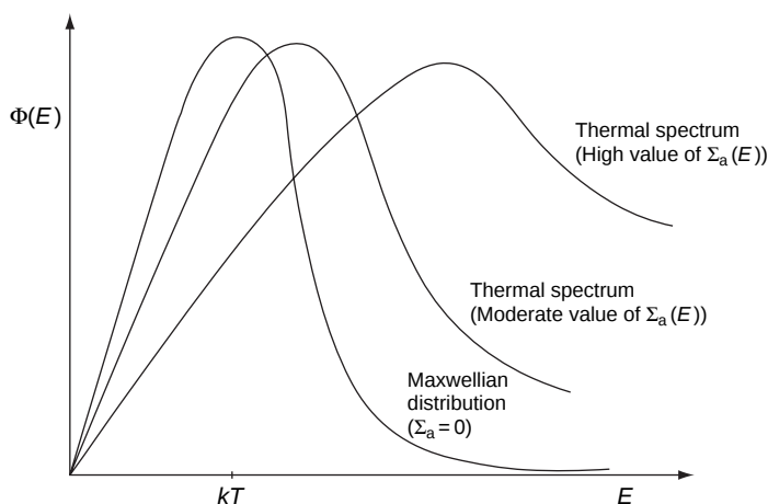
FIGURE 3.5 Thermal spectra compared to a Maxwell-Boltzmann distribution (adapted from A. F. Henry, Nuclear-Reactor Analysis , 1975, by permission of the MIT Press).
