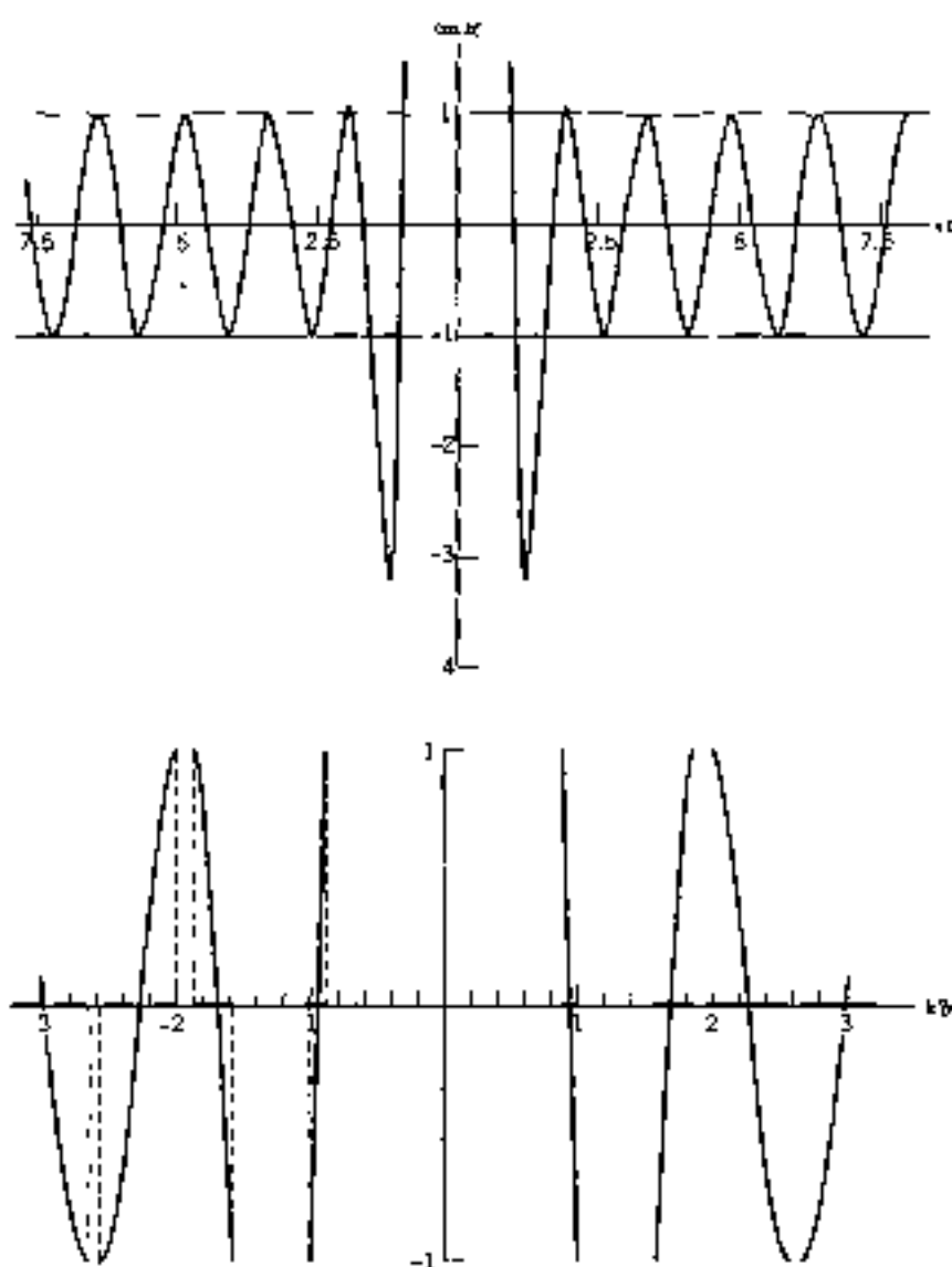
Figure 8.10. Plot of the right-hand-side of Eqs. (8.142) and (8.144) as a function of k' for a Kronig-Penney potential (Figure 8.9) with the choice of 4a = 4b = \xi for the linear dimensions and \sqrt{2m\hbar^2 V_0} = \pi\hbar/2 for the well depth. Since the plotted function equals \cos k\xi , only the segments of the curve between -1 and +1 are allowed. The enlarged detail plot shows the allowed bands (heavy black segments on the abscissa) and the forbidden energy gaps between them and illustrates the transition from tight binding to the nearly-free regime at high energies. The high peak of the curve at k' = 0 is suppressed.
