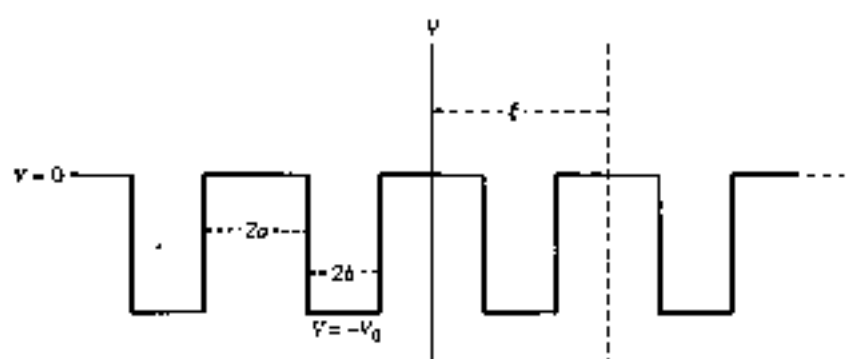
Figure 8.9. Periodic potential with rectangular sections (Kronig-Penney). The period has length \xi = 2a + 2b , and the well depth is V_0 .
