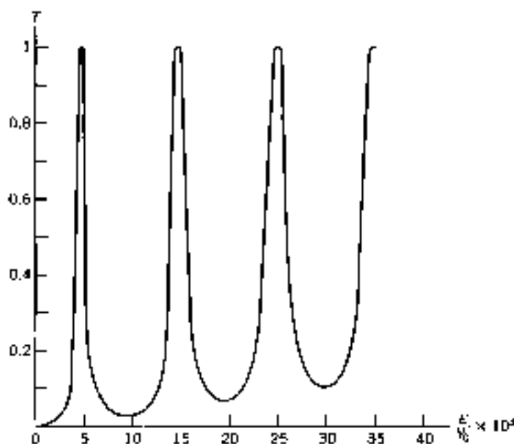
Figure 6.8. Transmission coefficient T versus E/V_0 for a deep square well with \beta = 315 . As \beta increases, the resonances become broader.
