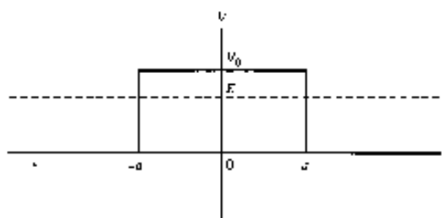
Figure 6.4. Rectangular potential barrier, height V_0 , width 2a .
