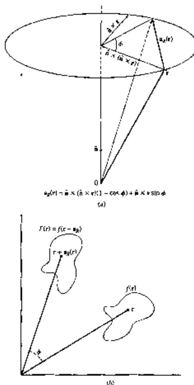
Figure 11.1. Rotation about an axis defined by the unit vector \hat{n} and the rotation angle \phi . (a) shows the displacement \mathbf{u}_R(\mathbf{r}) of the point whose position vector is \mathbf{r} . (b) illustrates the active rotation of a function or state f(\mathbf{r}) about an axis ( \hat{n} ) perpendicular to the plane of the figure: f(\mathbf{r}) \mapsto F(\mathbf{r}) = f(\mathbf{r} - \mathbf{u}_R) .
