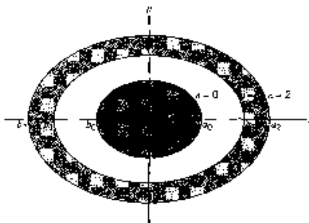
Figure 7.4. Phase space representation of the periodic motion of a particle confined between the classical turning points at x = a_1 and x = b_1 for the bound-state energies E_n = V(a_1) = V(b_1) . The area between two neighboring trajectories is equal to \hbar .
