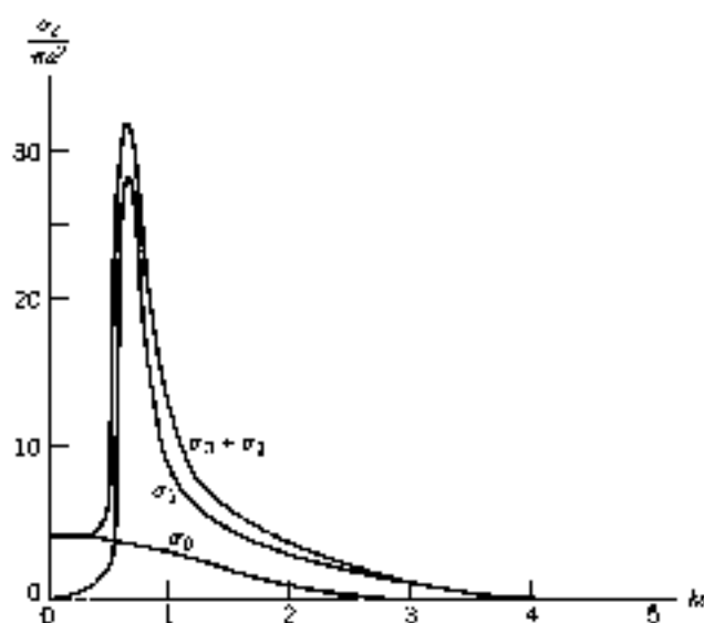
Figure 13.8. Momentum dependence of the partial cross sections ( \sigma_0 and \sigma_1 ) for S and P waves corresponding to the phase shifts of Figure 13.7. The cross sections are given in units of \pi a^2 .
