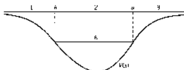
Figure 7.3. Simple one-dimensional potential well. Classically, a particle of energy E is confined to the region between a and b .
