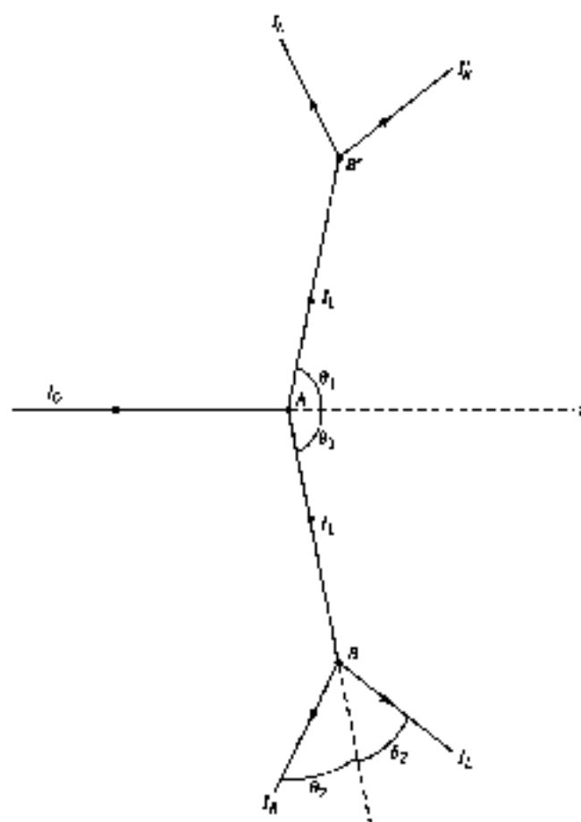
Figure 16.2. Geometry of a double scattering experiment. The first plane of scattering at A is formed by I_0 , I_1 , and I_2 , in the plane of the figure. The first scattering polarizes the beam, and the second scattering at B and B' analyzes the degree of polarization. The second plane of scattering, formed by I_1 , I_3 , and I_4 , need not coincide with the first plane of scattering. The angle between the two planes is \varphi , but is not shown.
