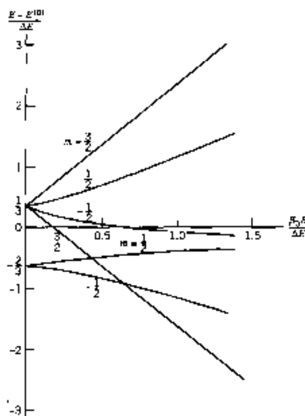
Figure 18.1. Splitting of a 2P energy level of hydrogen in a magnetic field B (Zeeman effect). The unperturbed energy is E^{(0)} , and the fine structure splitting is \Delta E .
