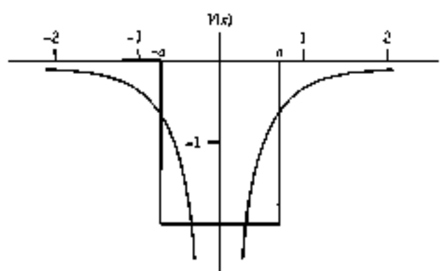
Figure 6.1. Potential approximating the attractive part of nuclear forces ( V = -e^{-\alpha}|x| ) and a one-dimensional square well simulating it.
