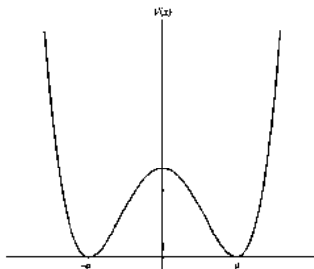
Figure 8.6. Quartic double-well potential, defined by Eq. (8.94).
