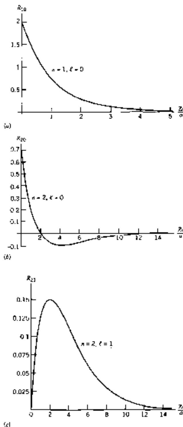
Figure 12.1. Radial bound-state energy eigenfunctions of the hydrogenic atom for n = 1, 2 , and 3. The radial coordinate r is scaled in units of a/Z . The wave functions are normalized as \int_0^\infty [R_{nl}(r)]^2 r^2 dr = 1 .
