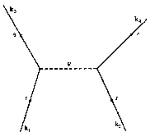
Figure 21.1. Diagram representing the two-particle matrix element \langle qr | V | rz \rangle . The vectors k_1 and k_2 (in units of \hbar ) are "in" momenta, and k_3 and k_4 are "out" momenta. (See Problems 1 and 2 in Chapter 21.)
