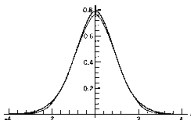
Figure 8.1. The thick line is the normalized ground state energy eigenfunction, \psi_0(x) = 1.47 \text{ Ai}[\sqrt{2}(x - 0.8086)] , for the potential V(x) = |x|^2 , and the thin line represents the optimal normalized Gaussian variational trial function, \phi(x) . The x coordinate and the energy are made dimensionless by scaling, as described in Section 7.3. The mean-square deviation between the two functions is only \int_{-\infty}^{\infty} |\psi_0(x) - \phi(x)|^2 dx \approx 10^{-3} !
