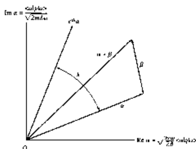
Figure 10.1. Two-dimensional phase space in Argand diagram representing a coherent state |\alpha\rangle in terms of the eigenvalue \alpha of the lowering or annihilation operator a . Also shown is the effect of a "displacement" D_\beta and a "rotation" R_\lambda on the coherent state |\alpha\rangle .
