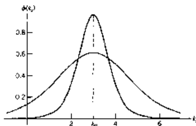
Figure 2.1. Example of a one-dimensional momentum distribution. The function \phi(k_x) = \sqrt{\alpha/2} [\cosh \alpha(k_x - k_0)]^{-1} represents a wave packet moving in the positive x direction with mean wave number k_0 = 3 . The function \phi(k_x) is normalized so that \int_{-\infty}^{\infty} |\phi(k_x)|^2 dk_x = 1 . The two functions correspond to \alpha = 0.72 and \sqrt{\pi} (heavy line).
