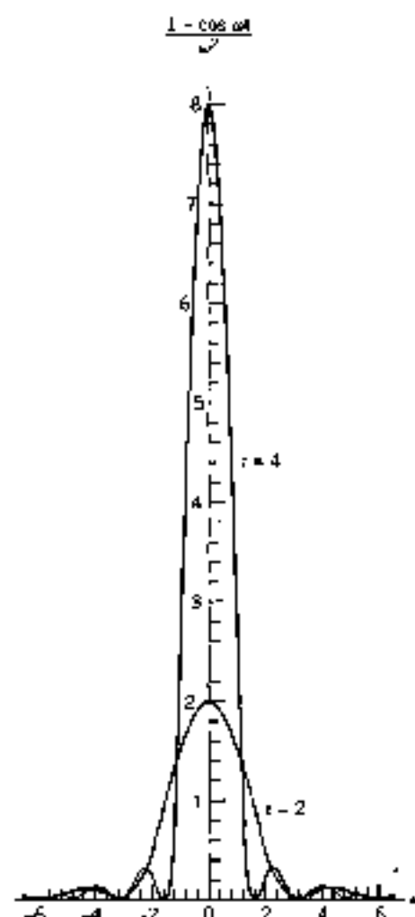
Figure 19.3. Plot of (1 - \cos \omega t)/\omega^2 versus \omega for different values of the time, t ( t = 2 and 4 ). The width of the peak is inversely proportional to t , and its height increases as t^2 , so that the area under the curve is proportional to t .
