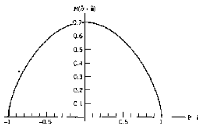
Figure 16.4. Outcome entropy H(\sigma \cdot \hat{n}) for a measurement of \sigma \cdot \hat{n} as a function of P \cdot \hat{n} .
