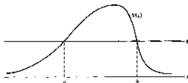
Figure 7.5. Potential barrier.
