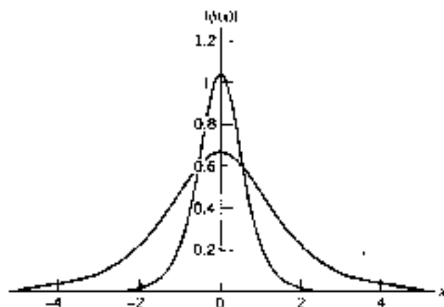
Figure 2.2. Normalized wave packet corresponding to the momentum distributions of Figure 2.1. The plotted amplitude, |\psi(x)| = \frac{\sqrt{\pi}}{\sqrt{4\alpha}} \left( \cosh \frac{\pi x}{2\alpha} \right)^{-1} , modulates the plane wave e^{ik_0 x} . Note the reciprocity of the widths of the corresponding curves in Figures 2.1 and 2.2.
