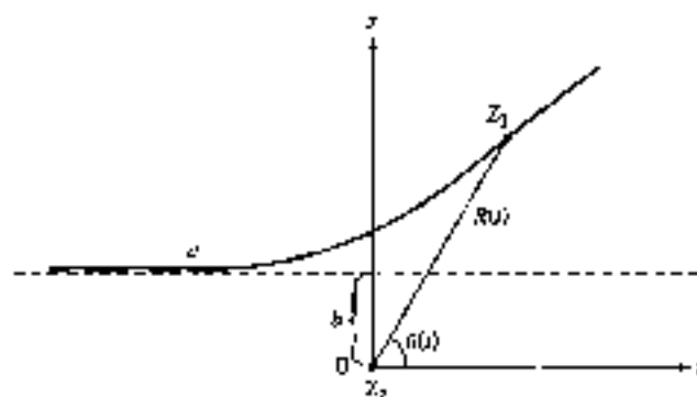
Figure 19.1. The Coulomb field of a charged particle Z_1 passing near a charged target Z_2 causes internal excitation. The impact parameter is b , and the coordinates \theta(t) and R(t) determine the instantaneous position of the projectile.
