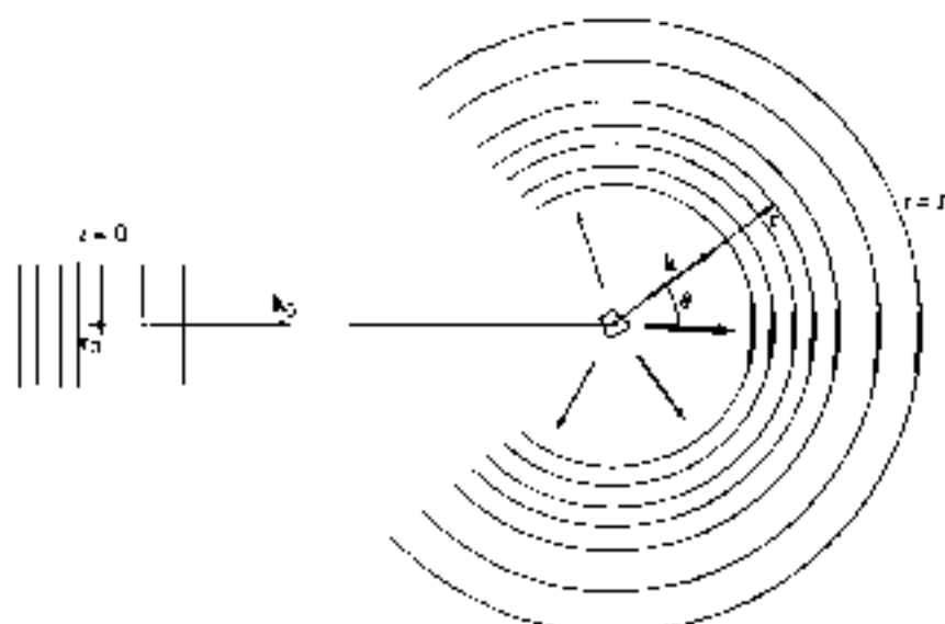
Figure 13.2. Scattering of a wave packet incident from the left with mean momentum \hbar k_0 . In elastic scattering, the wave packet is scattered with equal energy but varying amplitudes in different directions (indicated by the thickness of the arrows). In the forward direction, the scattered wave interferes with the advancing incident wave.
