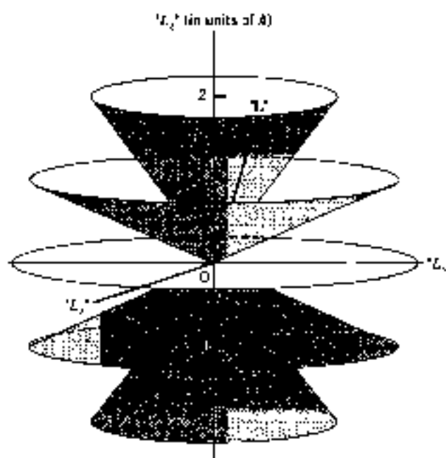
Figure 11.2. A cartoon illustrating the angular momentum eigenstates |\ell m\rangle for \ell = 2 . The semiclassical angular momentum vector " \mathbf{L} " has length \sqrt{\ell(\ell+1)}\hbar = \sqrt{6}\hbar , but its z component assumes the possible values " L_z " = 0, +\hbar , +2\hbar . This is visualized by supposing that the " \mathbf{L} " vector is stochastically distributed on one of the circular cones with uniform probability. The mean values of " L_x " and " L_y " obtained from this model [zero and (6 - m^2)\hbar^2/2 , respectively] agree with the expectation values of the corresponding quantum operators.
