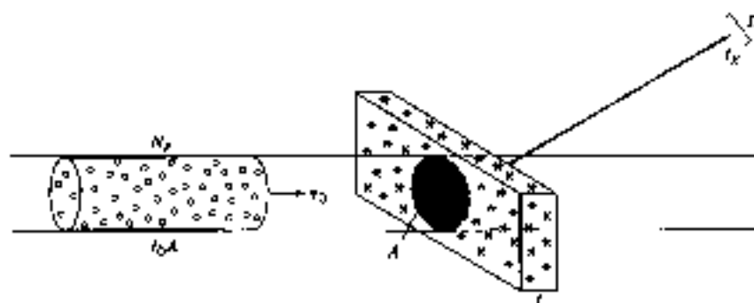
Figure 13.1. Sketch of a scattering experiment. A pulse of N_p = I_0 A projectile particles is incident from the left with velocity v_0 . The beam intersects an area A of the target (thickness r and particle density n ) and encounters N_T = nrA target particles. The detector D registers I_k outcomes X , and the corresponding cross section is \sigma = I_k/N_p I_0 .
