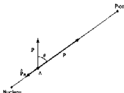
Figure 17.2. Kinematics of the decay of a spin-polarized hyperon at rest into a nucleon and a pion. The polarization vector is \mathbf{P} . The magnitude of the relative momentum p equals that of the momenta of the two decay products in the rest frame of the hyperon. The unit vector \hat{\mathbf{p}}_N points in the direction of emission of the nucleon.
