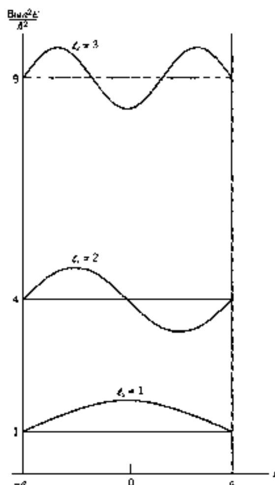
Figure 4.2. The three lowest energy eigenvalues ( l = 1, 2, 3 ) and the corresponding eigenfunctions for a one-dimensional box of dimension L = 2a . The unit of energy on the ordinate is \hbar^2/8ma^2 . The maximum amplitude of the normalized eigenfunctions is \sqrt{1/a} .
