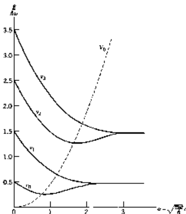
Figure 8.5. The energy E = \hbar \omega \left( n + \frac{1}{2} \right) in units of \hbar \omega versus a = \sqrt{m\hbar^2/\kappa} a for the four lowest energy eigenstates of the double oscillator, V(x) = m\omega^2(|x| - a)^2/2 . For comparison with the energy levels, the dashed curve shows the barrier height V_0 .
