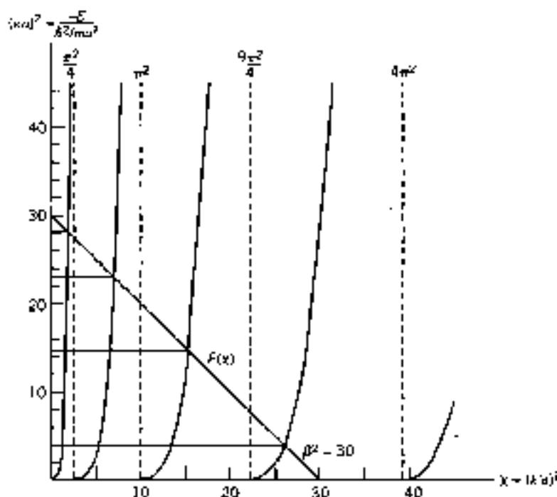
Figure 6.6. Graphical determination of the energy levels in a square well with \beta^2 = 30 . The curves for (a) \sqrt{\chi} \geq 0 ( f_{\text{even}} ) alternate with those for (a) \sqrt{\chi} \leq 0 ( f_{\text{odd}} ). The ordinates of the intercepts are the binding energies in units of \hbar^2/2ma^2 . The dashed-line asymptotes intersect the abscissa at the energy eigenvalues (6.52), again in units \hbar^2/2ma^2 , for a particle confined to the box -a \leq x \leq a . This figure may be used as a template for estimating the bound-state energies for any one-dimensional square well; merely draw a parallel to the diagonal straight line F(\chi) = \beta^2 - \chi for the desired value of \beta .
