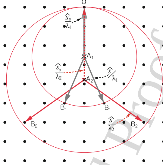
Fig. 1.20. Ewald construction for diffraction peaks
