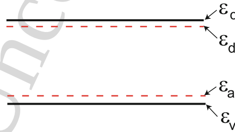
Fig. 7.3. Impurity levels in semiconductors doped with N_d donors and N_a acceptors per unit volume
