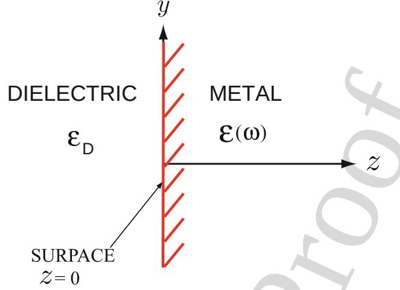
Fig. 3.6. Interface between a dielectric and a metal
