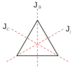
Fig. 5.1. Equilateral triangle
