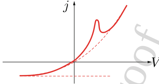
Fig. 7.7. Current-voltage characteristic across a heavily doped p-n junction
