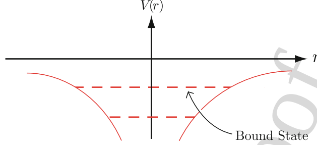
Fig. 4.1. Coulomb potential
