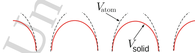
Fig. 4.3. Tight-Binding Potential
