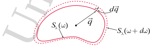
Fig. 2.10. Constant frequency surfaces in three-dimensional wave vector space
