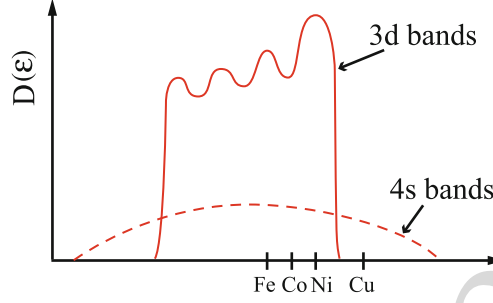
Fig. 10.16. Schematic illustration of the density of states of the transition metals
