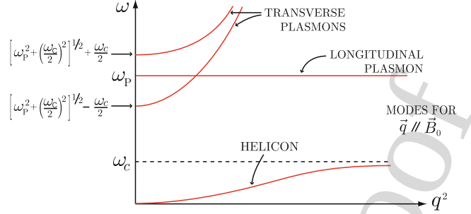
Fig. 14.5. The dispersion curves of magnetoplasma modes in a metal when the wave propagates in the z -direction parallel to the dc magnetic field \mathbf{B}_0
