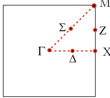
Fig. 5.5. First Brillouin zone of a square lattice
