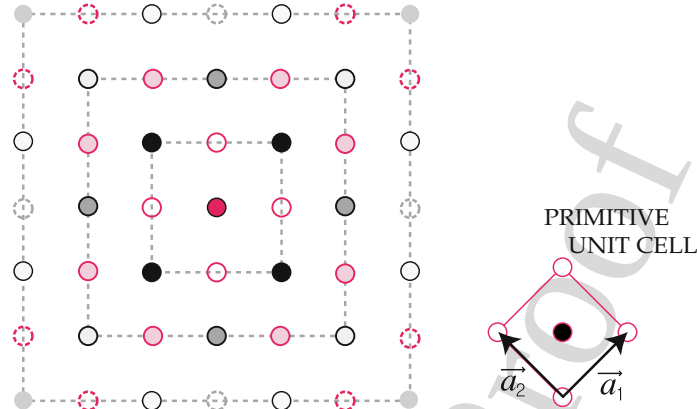
Fig. 1.25. Evjen method for a simple square lattice in two dimensions
