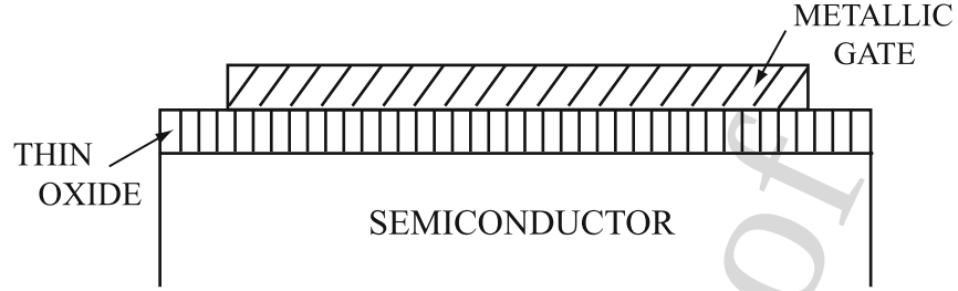
Fig. 7.9. Metal-oxide-semiconductor structure
