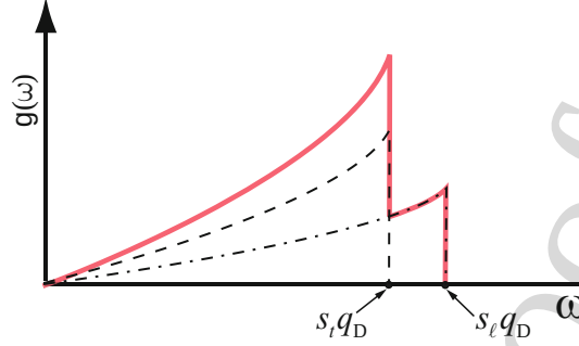
Fig. 2.11. Three-dimensional density of states in the Debye model
