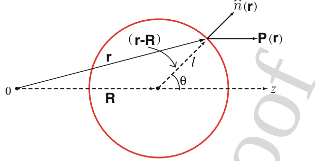
Fig. 8.4. A Lorentz sphere of radius \ell centered at \mathbf{R}
