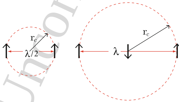
Fig. 14.11. Schematic of the origin of the geometric resonances in ultrasonic attenuation
