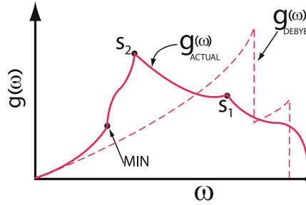
Fig. 2.15. Comparison of the density of states g(\omega) for a Debye model and that of a real crystal
