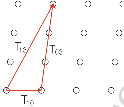
Fig. 1.1. Translation operations in a two-dimensional lattice
