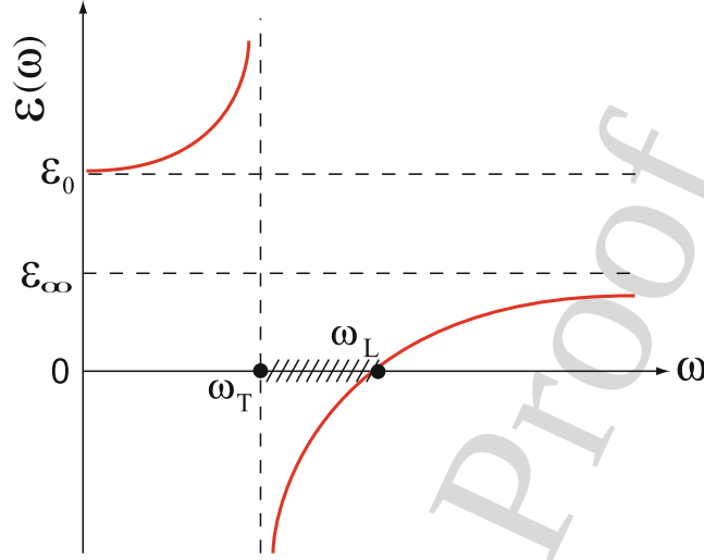
Fig. 8.21. Dielectric function \varepsilon(\omega) of a polar crystal
