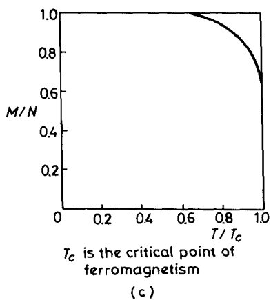
Fig. 17-3 (a) specific heat, (b) energy, (c) magnetic moment. The dotted lines are results from mean field approximation. (See Chapter 27, T_c is 4J in the mean field approximation).
