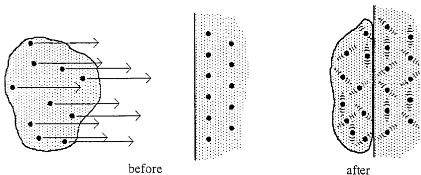
Figure 12.3 A ball of putty before and after its collision with a wall. The motion of some representative molecules is indicated. During the collision the coherent component of their motion (translation) is transformed into random thermal motion. Since there are far more states available for the molecules to oscillate in random directions than for them to all move in the same direction, the entropy increases during the collision.
