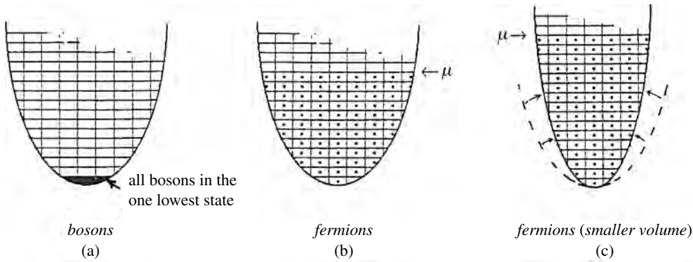
Figure 9.8 At low temperatures, systems become “degenerate,” with all particles occupying the states of lowest energy. (a) All bosons fall into the one state of lowest energy. (b) Unlike the bosons, no two identical fermions may occupy the same state, so they fill the lowest N states, forming a “Fermi sea.” (c) If identical fermions must fill a smaller spatial volume, the Fermi level is correspondingly higher.
