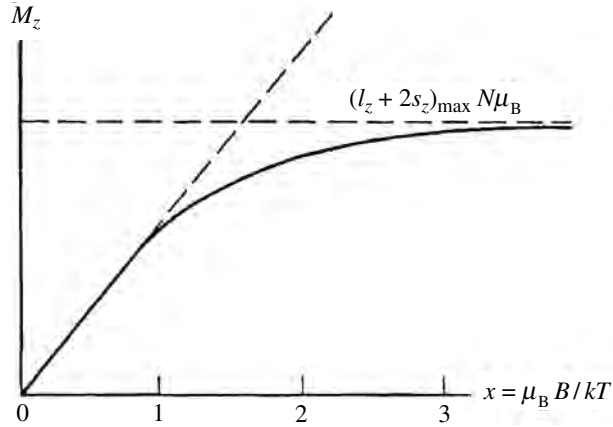
Figure 17.4 Plot of magnetic moment M_z vs. x = \mu_B B / kT for a typical paramagnetic substance. For \mu_B B / kT \ll 1 , the magnetic moment increases linearly with the external magnetic field according to the Curie law, M_z = C(B/T) . For \mu_B B / kT \gg 1 , the magnetic moment reaches its maximum value, (l_z + 2s_z)_{\max} N \mu_B . For \mu_B B / kT intermediate between these two extremes, it would be necessary to use equations 17.7 and 17.10 for the magnetic moment.
