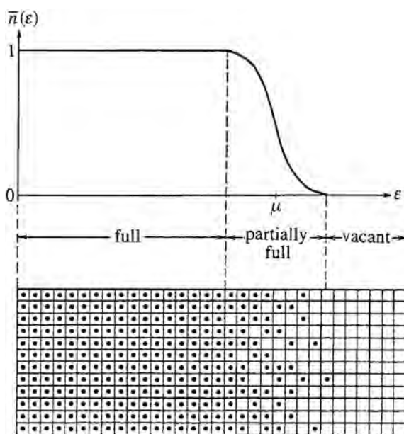
Figure 22.2 Only electrons near the Fermi level ( \varepsilon_f \approx \mu ) have any freedom at all, because only these electrons might be able to find vacant neighboring states into which they can move in response to thermal agitation or other stimuli.
