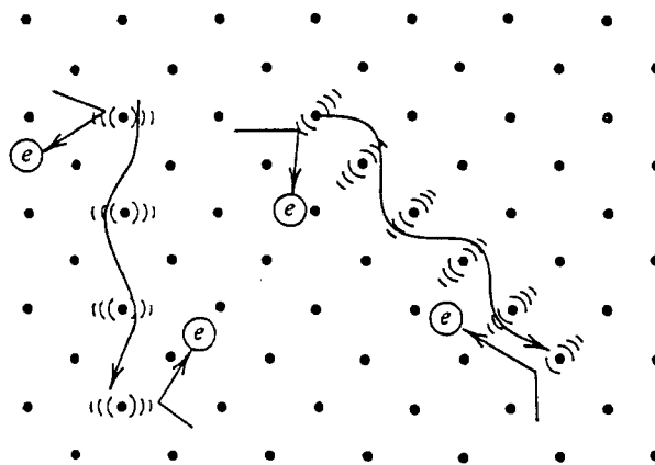
Figure 24.7 Interactions between superconducting electrons are mediated by phonons. That is, an electron interacts with one lattice point, and the elastic wave that it produces travels through the solid until it transfers this energy to some other electron.
