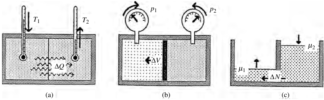
Figure 9.4 For thermal, mechanical, or diffusive interactions, the second law guarantees the following. (a) Heat flows from hot to cold; as a result, the higher temperature falls and the lower temperature rises. (b) The piston moves from high pressure toward low. As a result, the higher pressure falls and the lower pressure rises. (c) Particles flow from high chemical potential to low. As a result, the higher chemical potential falls and the lower one rises. That is, all changes are in the direction that approaches equilibrium.
