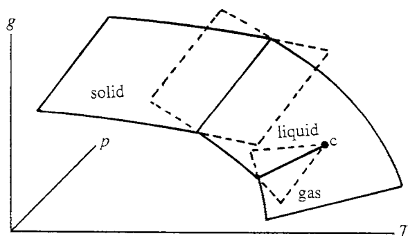
Figure 14.9 Plot of the molar Gibbs free energy g as a function of T and p , showing parts of the minimum- g surfaces corresponding to the solid, liquid, and gas phases. Because dg = -s dT + v dp , the slopes of these surfaces in the T and p directions are equal to the molar entropy and volume, respectively. The lines of intersection of the surfaces identify the phase boundaries. The critical point c for the liquid–gas transition is also indicated.
