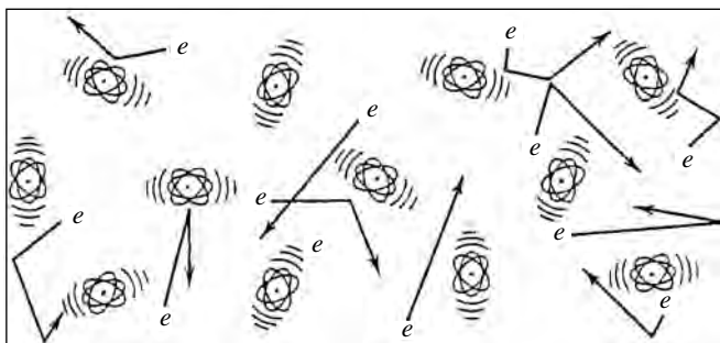
Figure 22.1 We can view a solid as a system of atomic oscillators, and it might also include a gas of conduction electrons that are confined within its boundaries.
