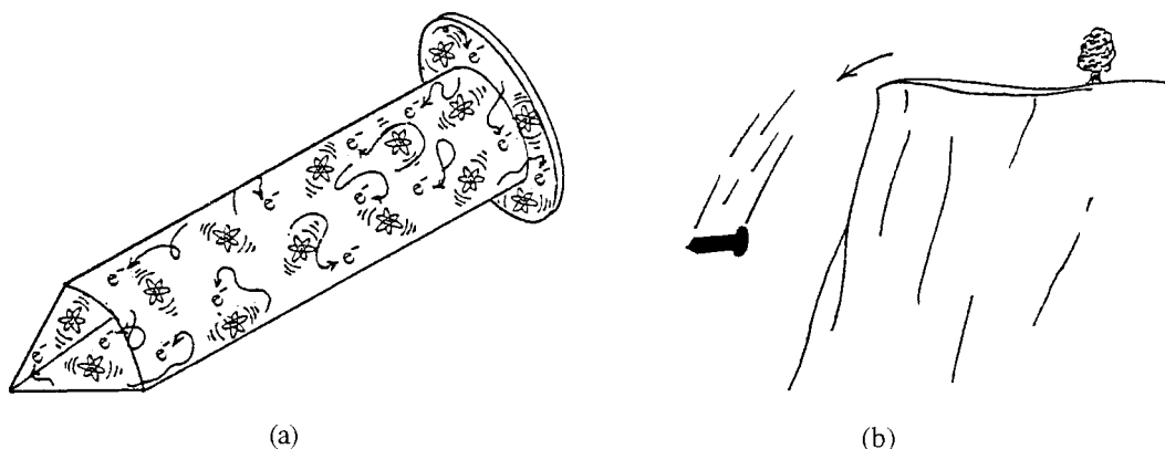
Figure 4.1 (a) The internal energy of a nail includes such things as the vibrations of the iron atoms and the potential and kinetic energies of the conduction electrons. (b) If the nail were thrown over a cliff, its motion relative to the Earth and its potential energy due to the Earth's gravity would not be part of its internal energy, because they involve more than just the nail itself.
