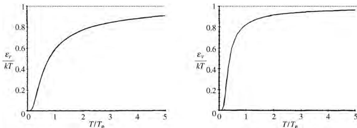
Figure 18.2 Plots of the average rotational (left) and vibrational (right) energies per molecule as a function of the temperature for a diatomic gas. The energy is in units of kT and the temperature is in units of the excitation temperature T_e , which is typically 5–10 K for rotations and 1000–2000 K for vibrations.
