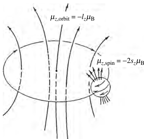
Figure 17.3 An atomic electron makes two contributions to the magnetic moment of the atom, one due to its orbit and the other due to its spin. Both orbits and spins create tiny current loops, with corresponding magnetic moments. The gyromagnetic ratio g is -1 for the orbit and -2 for the spin.
