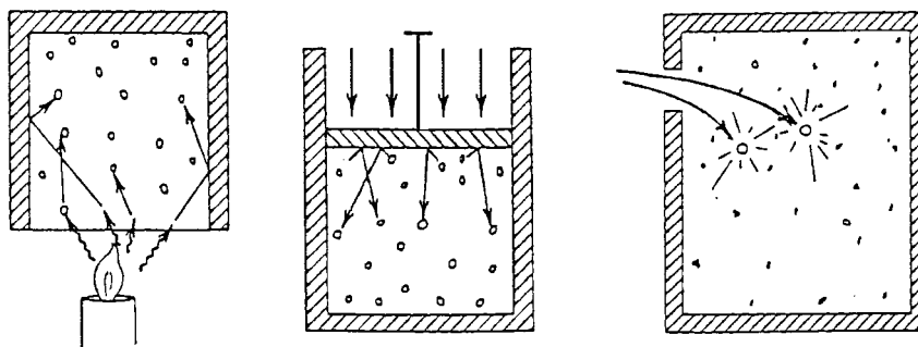
Figure 6.1 The addition of energy or particles usually occurs in a small localized region of a system, such as along a boundary. The system is not in equilibrium until interactions among particles have provided the opportunity for the added energy and particles to be anywhere, so that all possible distributions are equally likely. The time required for this to happen is the relaxation time. From that point on, the probabilities for the various possible configurations remain the same.
