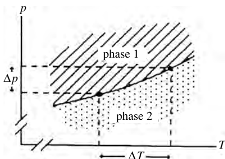
Figure 14.5 A small portion of a line separating two phases on a phase diagram. The two phases are in equilibrium along this line, so their chemical potentials must be equal. For them to remain equal as we move along this line, they must both change by the same amount: \Delta\mu_1 = \Delta\mu_2 .
