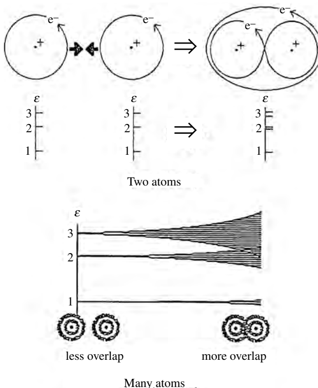
Figure 23.1 (Top) A schematic diagram, showing that when as identical atoms are brought together, their outer electrons may be shared. The identical electron states of the isolated atoms split into slightly different states for mutually shared electrons. (Bottom) When N atoms come together, each electron state splits into a band of N different states. The larger the overlap of atoms, the greater the spreading. So in general the bands are wider when the atoms are closer together and the bands for outer states are wider than those for inner states.
