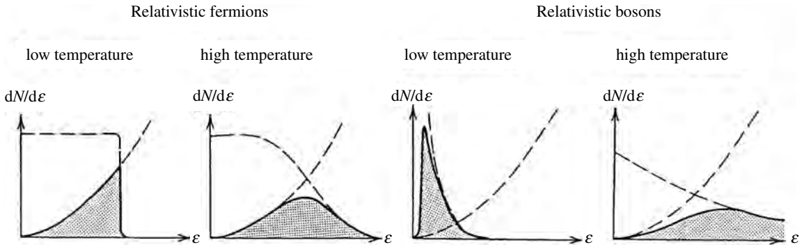
Figure 20.3 Particle distributions in relativistic ( g(\varepsilon) \propto \varepsilon^2 ) quantum gases at low and high temperatures.
