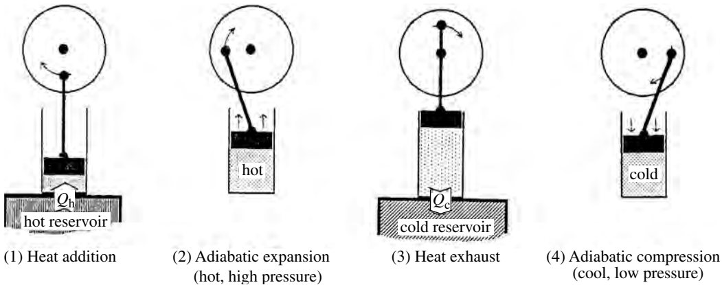
Figure 13.2 Elements of a simple piston engine.
