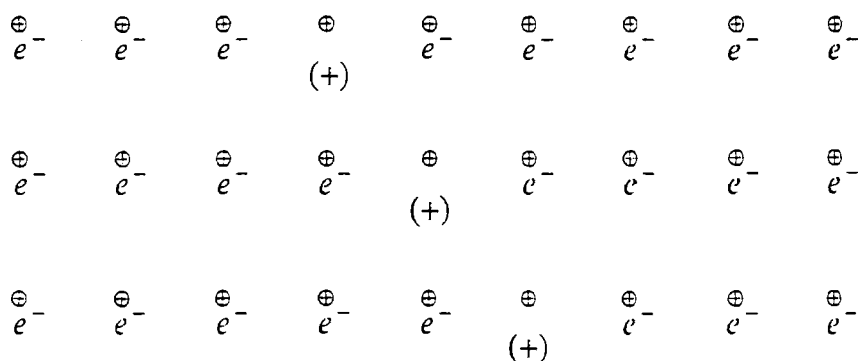
Figure 10.6 Illustration of conduction by holes in the valence band, with the three sequences progressing from top to bottom. The encircled plus signs represent the fixed positive ions. When an electron moves in one direction to fill up a vacancy, it leaves another vacancy behind. Each vacancy is called a “hole” and carries a net positive charge, because it is an atom that is missing an electron. In the figure the electrons are moving to the left and the hole is moving to the right, this being the conventional direction of the electric current.
