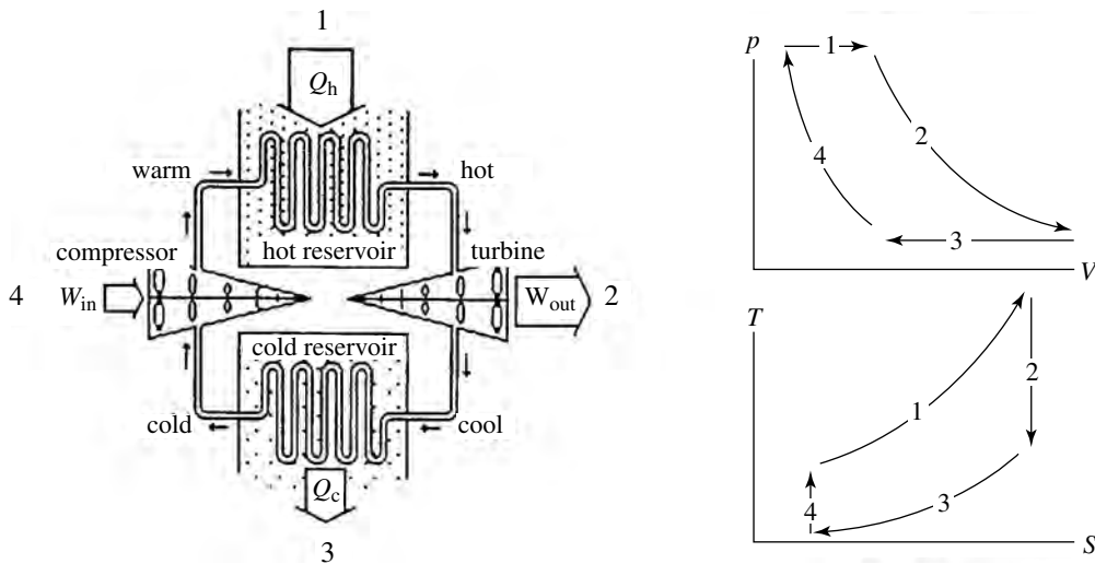
Figure 13.5 Elements of a gas turbine engine, and the model cycle on a p-V diagram and on a T-S diagram. The cycle includes (1) isobaric heating from the hot reservoir, (2) adiabatic expansion through the turbine, (3) isobaric cooling in the cold reservoir, (4) adiabatic compression in the compressor.
